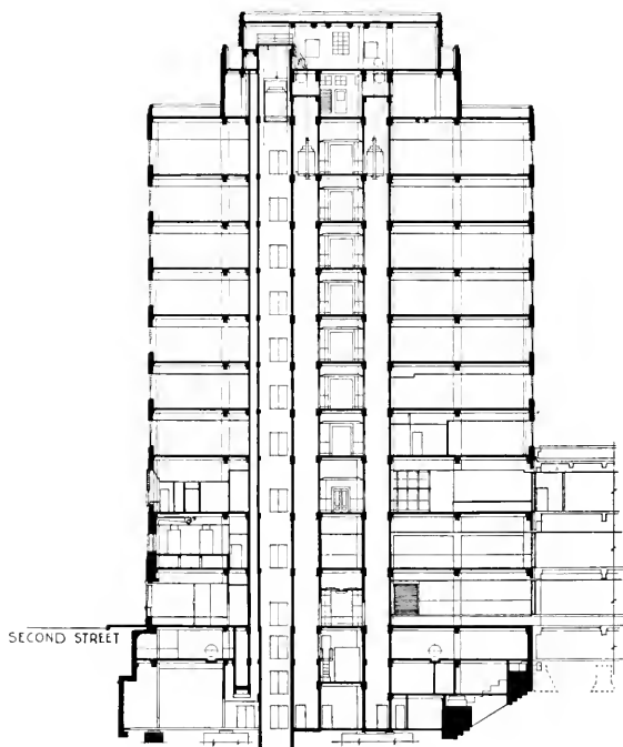
CROSS SECTION
