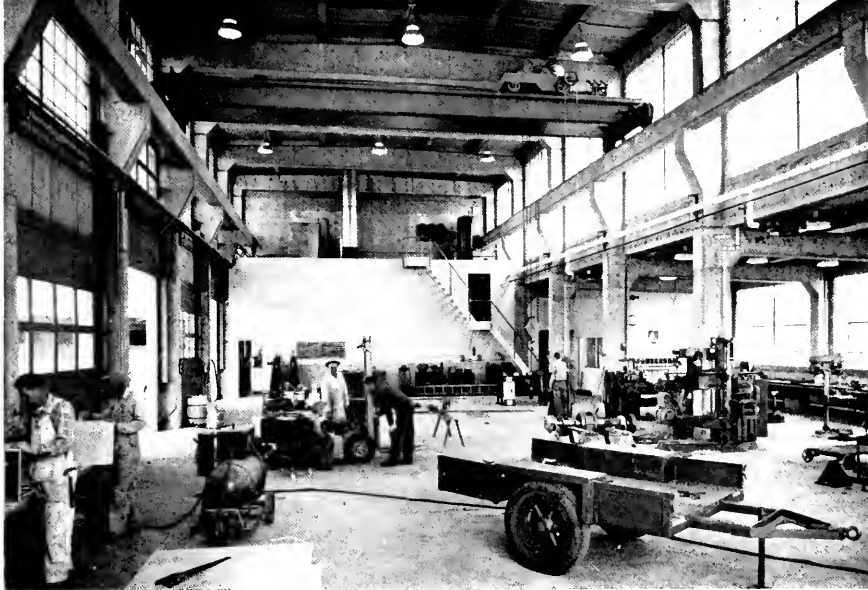
Interior of shop showing rigid frame of concrete skeleton. Concrete framing cast in single unit with overhead beams, columns, horizontal beams and corbels tied together. All work may be done indoors.
