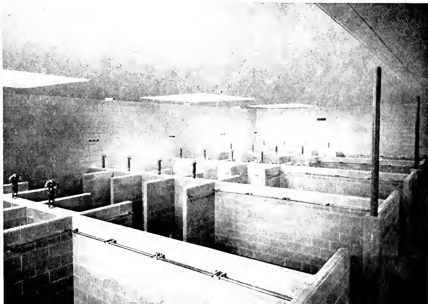
CLEAR glazed Structural Units used in girls' shower and dressing room of South East Junior-Senior High School in San Diego, California. Sam W. Hamill, Architect.
