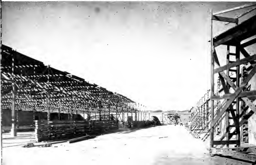
PRE-CAST tilt-up concrete walls are set on solid base
