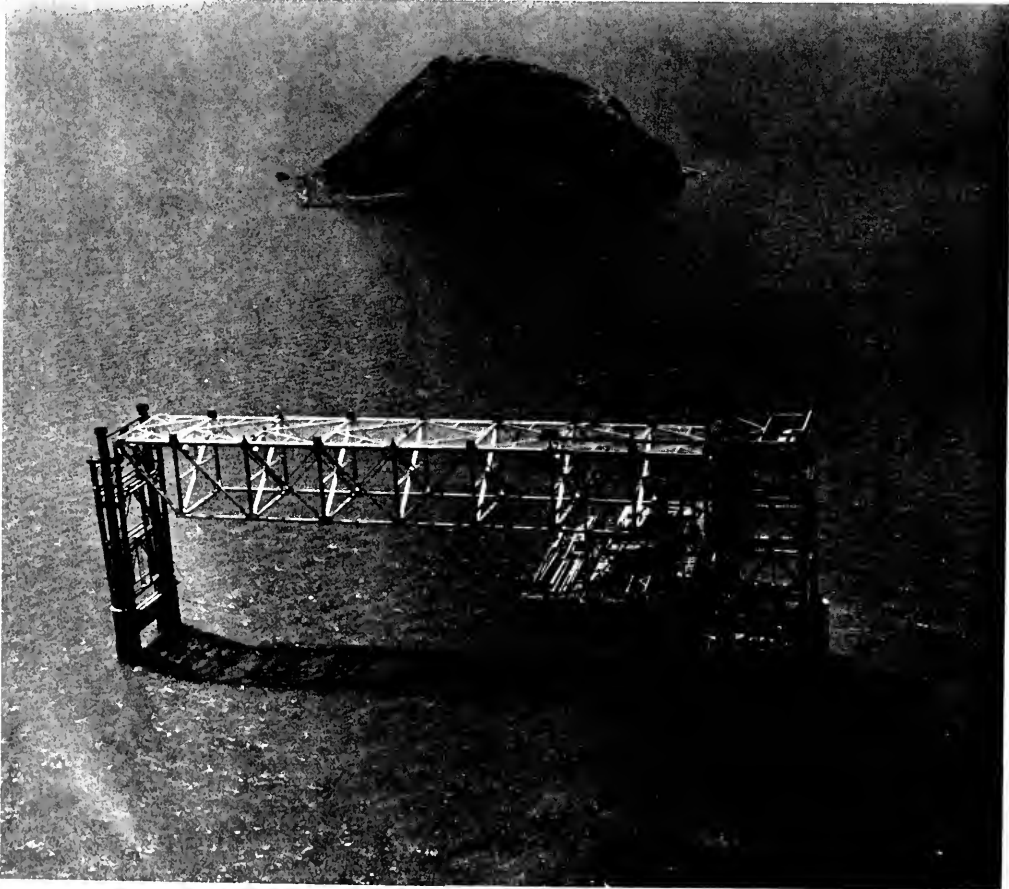
Fig. 3—Erecting First Piece of Steel Upon Aluminum Falsework Truss.
