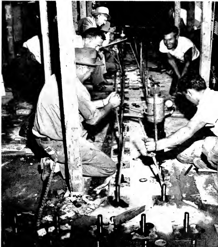
Tensioning crew in action. Note method of taking up elongation of bar with pin wrench. Split washer or shims at hand to slip into place when proper elongation is obtained.
