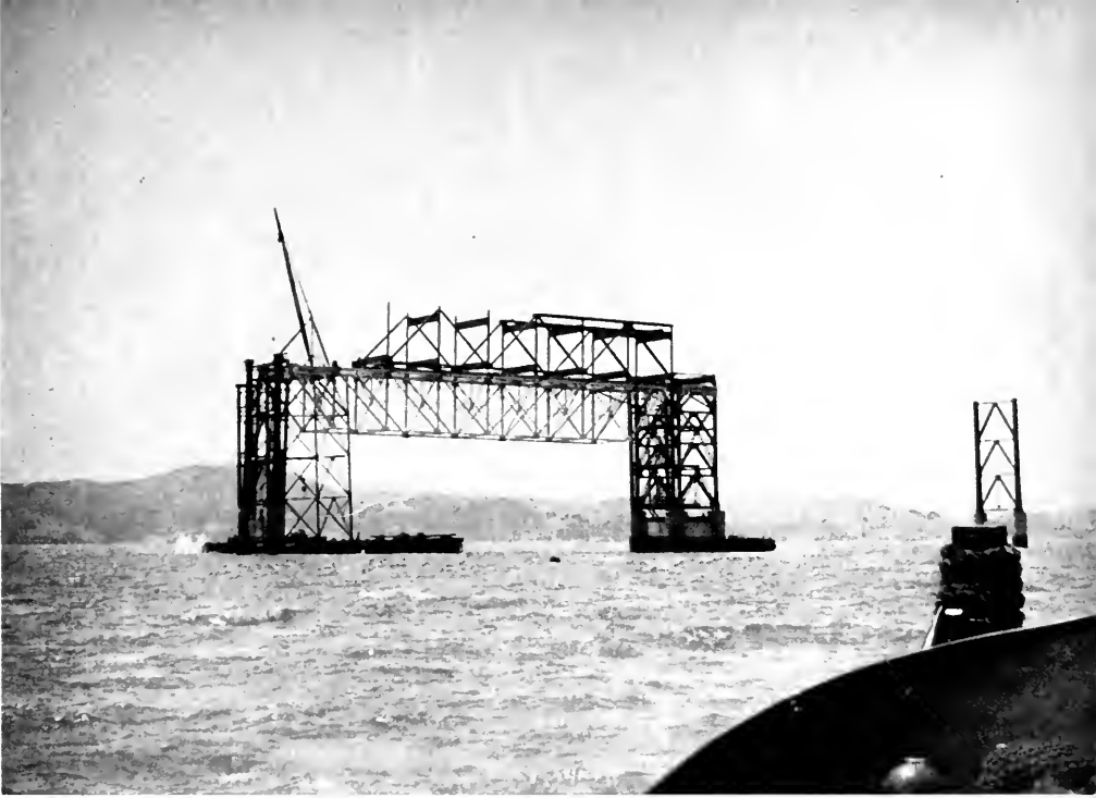
Fig. 4—Position of Permanent Steel Truss Being Erected Upon Aluminum Falsework Truss.
