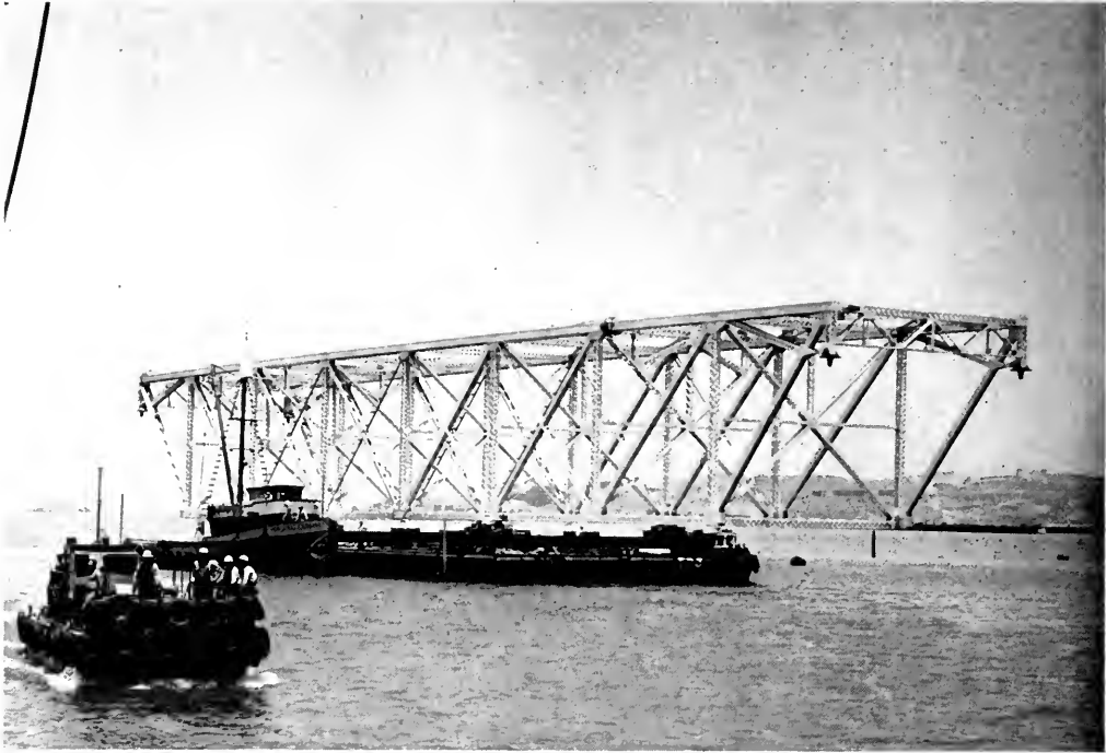
Fig. 1—Aluminum Falsework Truss Being Towed Into Position.
