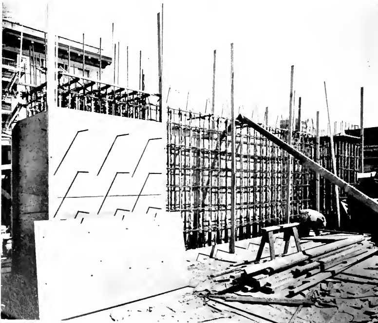
View of entire pylon at Third Floor level at completion of tensioning of Stress steel bars.
