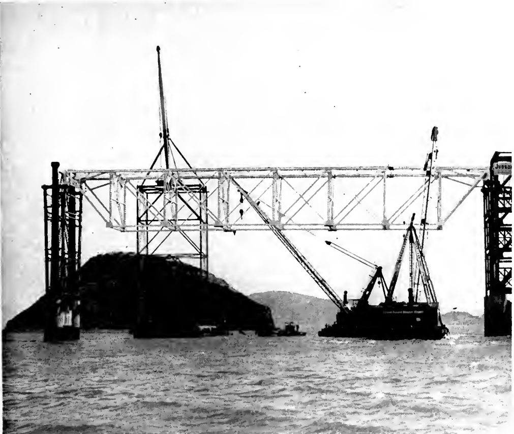
Fig. 2—Aluminum Falsework Truss Raised Into Position and Ready for Steel Erection.
