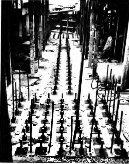
View of entire pylon at Third Floor level at completion of tensioning of Stress steel bars.
