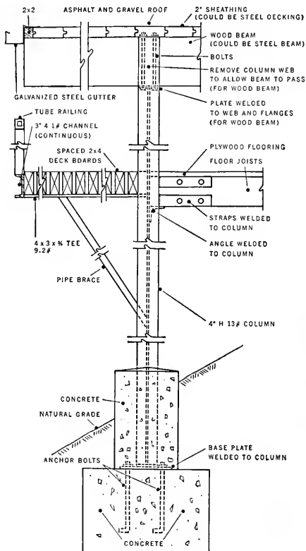
TYPICAL SECTION
