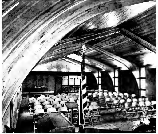
Heavy haunches of the fir arches provide support for this church.
