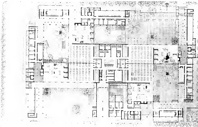
MAIN FLOOR PLAN 3
