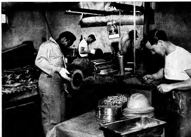
PARTIAL VIEW of polishing room, showing polisher satin-finishing door plate, buffing door framing, pans, small parts, etc.
