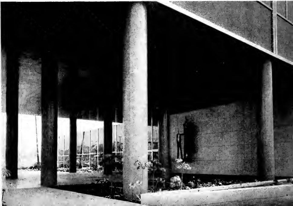
West entrance foyer showing glazed ceramic tile saffit and column facing with anchor type ceramic veneer wall as background for planting and for bronze sculpture.
