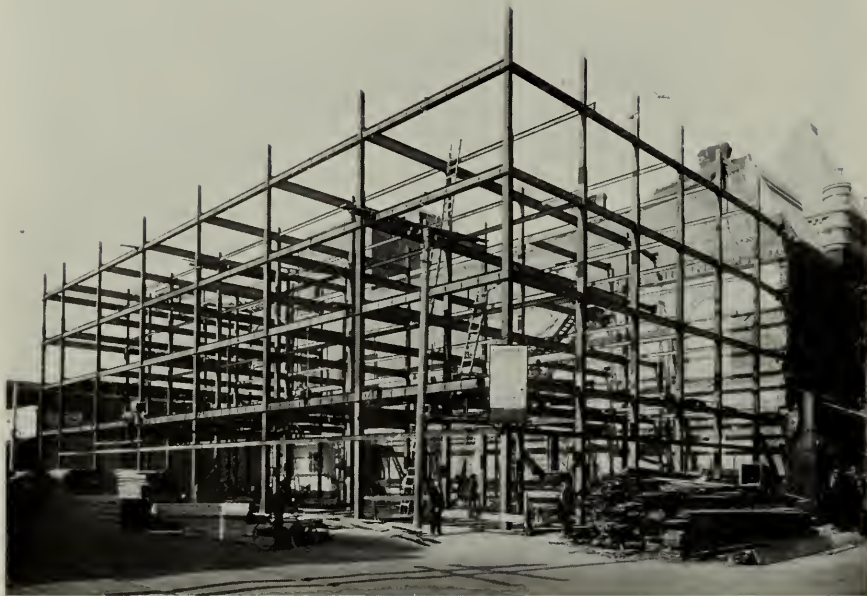
STEEL FRAME OF L. L. CORY BUILDING, FRESNO, CALIFORNIA
