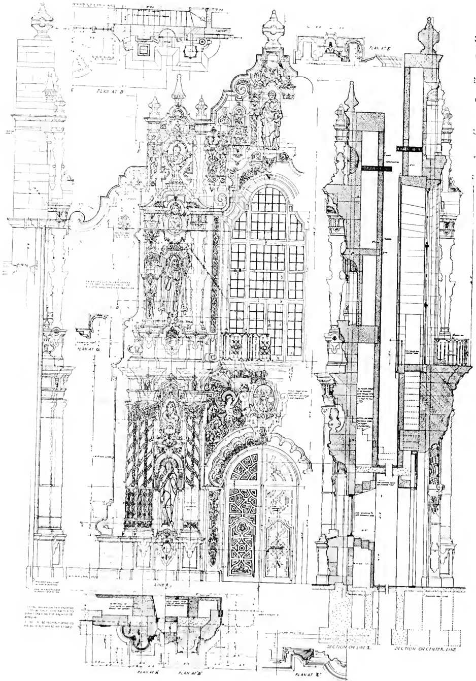
FRONTISPIECE AT ENTRANCE, CALIFORNIA STATE BUILDING, PANAMA-CALIFORNIA EXPOSITION, SAN DIEGO C.R.A.M., GOODHUE & FERGUSON, ARCHITECTS Bertram Grosvenor Goodhue, Advisory and Consulting Architect to the Exposition.
