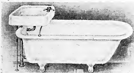
THE "BOUDOIR" BATH FIXTURE
