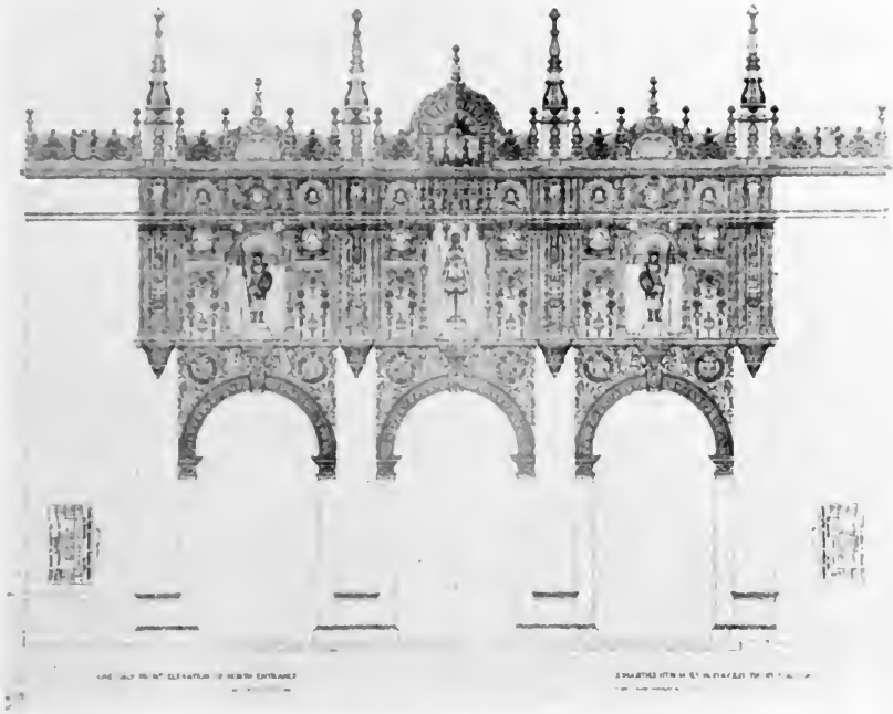
DETAIL OVER DOORWAY, TRANSPORTATION BUILDING Bliss & Fardle, Architects
