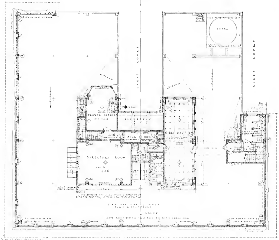
ROOF PLAN
