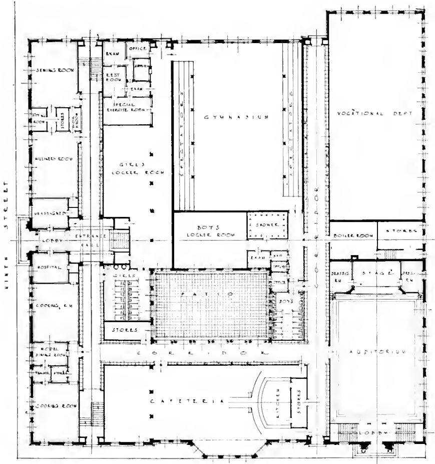
BISSELL AVENUE JUNIOR HIGH SCHOOL, RICHMOND, CAL. Jas. T. Narbett, Architect
