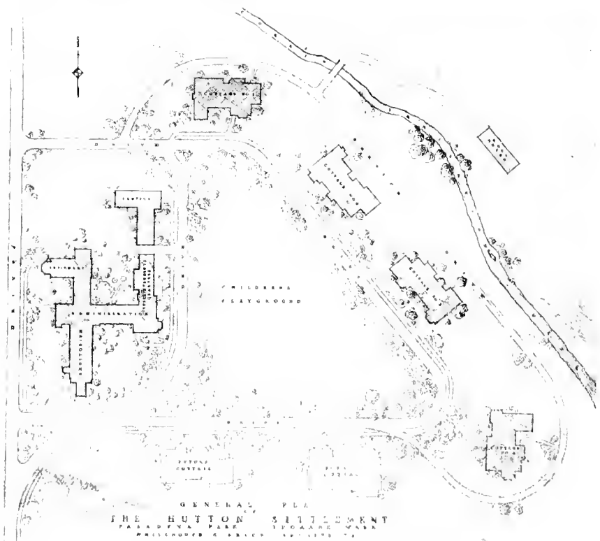
GENERAL PLAN, THE HUTTON SETTLEMENT, PASADENA PARK, SPOKANE, WASH. Whitthouse & Price, Architects
