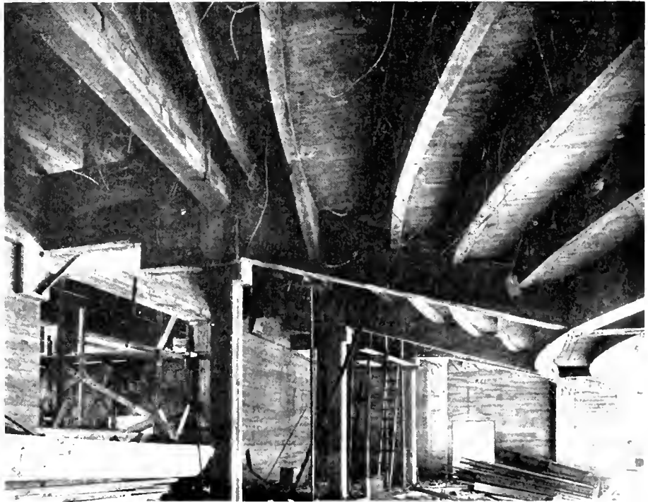
CONSTRUCTION PHOTOGRAPHS, MOROSCO, THE AIRE, LOS ANGELES - MORGAN, WALLS & MORGAN, ARCHITECTS
