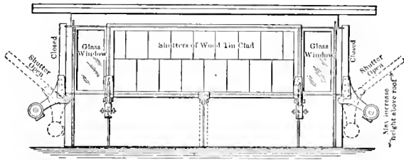
SMOKE VENT. MONITOR TYPE SIDE ELEVATION
