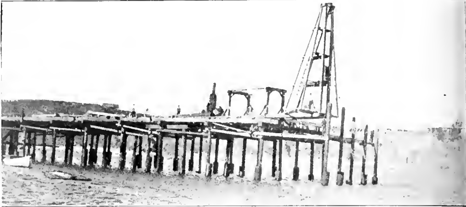
Fig. 1—This photograph shows the use of Armeo ingot iron corrugated pipes to protect a wharf, recently built at Port Orford, Curry County, Oregon, from the ravages of the teredo.
