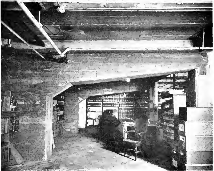
CANTILEVER IN BASEMENT AT INNER PROPERTY LINE COLUMN, ROBERT DOLLAR BUILDING, SAN FRANCISCO CHAS. W. McCALL, ARCHITECT
