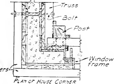
DETAILS OF INGERSOLL STANDARD FORMS
