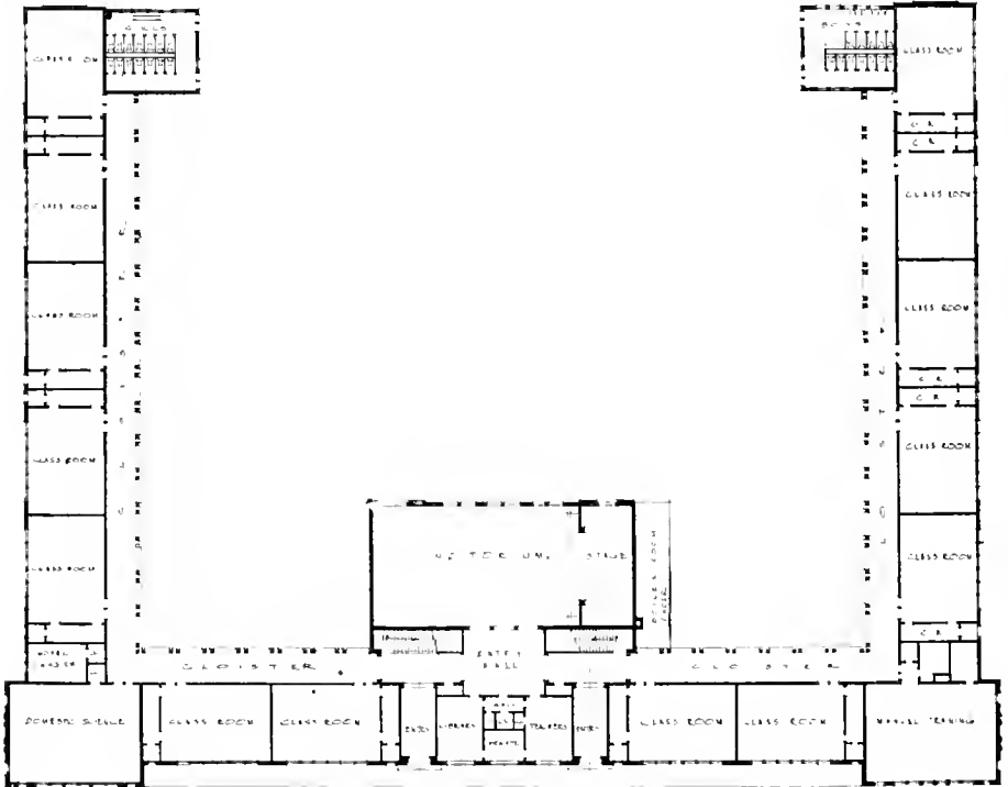
STEGE SCHOOL, RICHMOND SCHOOL DISTRICT, CAL. Jas. T. Nabrett, Architect
