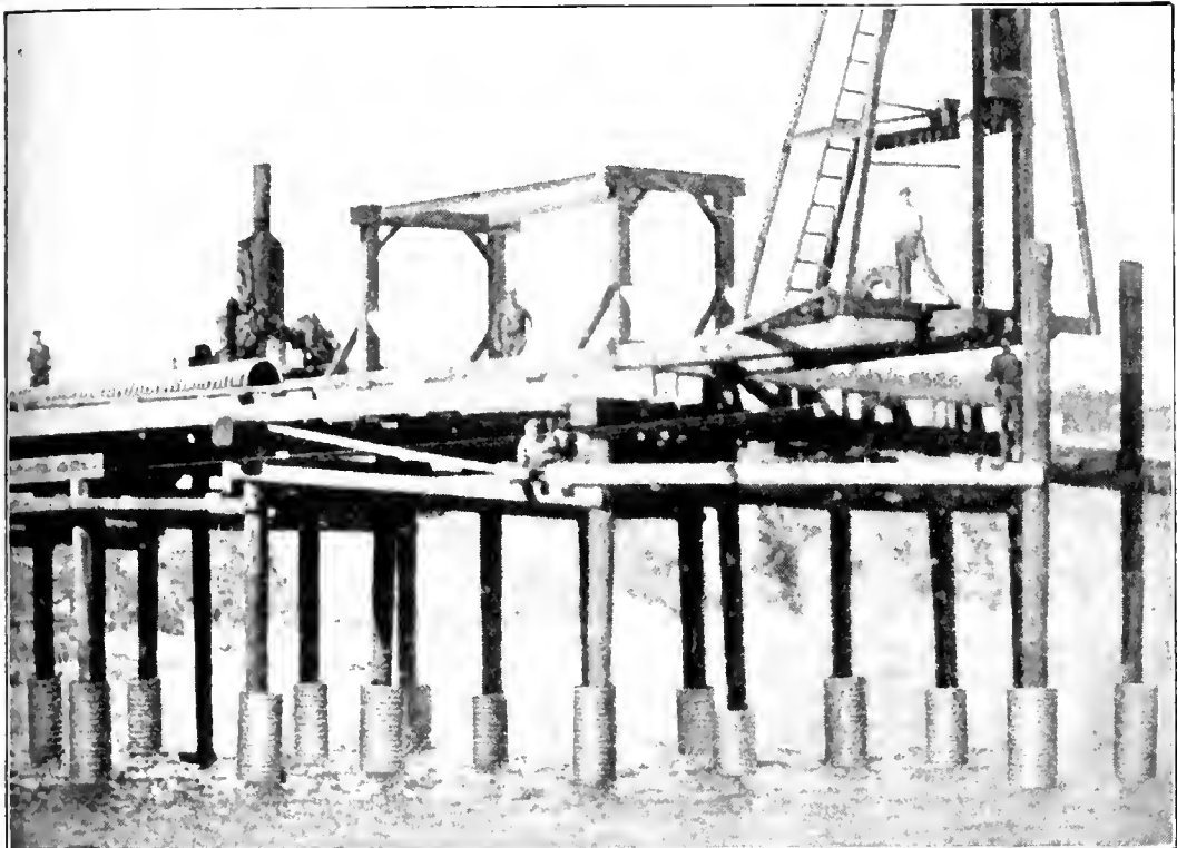
Fig. 3—A close-up view of the wharf recently constructed by the port of Port Orford, Curry County, Oregon, showing how mgot iron corrugated pipes were installed to prevent attacks by marine woodborers.
