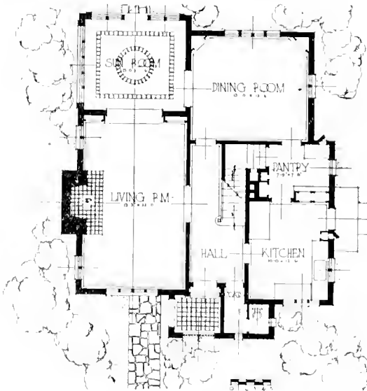
PLAN, E. V. PRICE RESIDENCE
