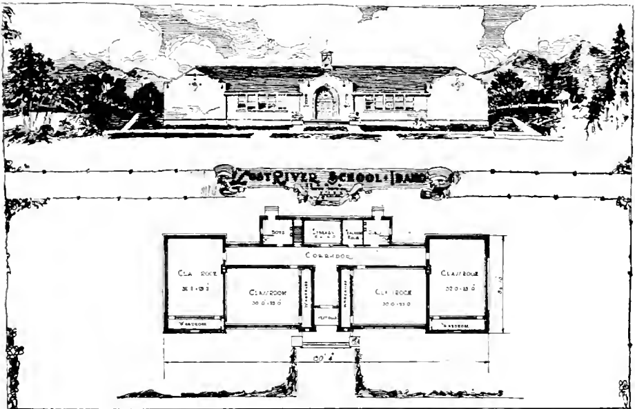
LOST RIVER SCHOOL, IDAHO Newton J. Thornton, Architect
