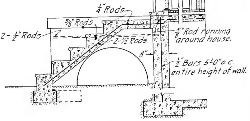
CROSS SECTION OF WALL.
