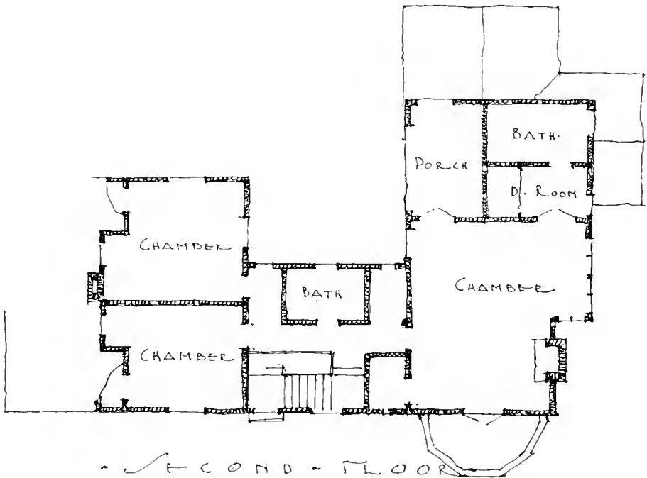
SECOND FLOOR PLAN, HOUSE FOR MR. JESSE ROBINSON, CLAREMONT MANOR, CALIFORNIA
