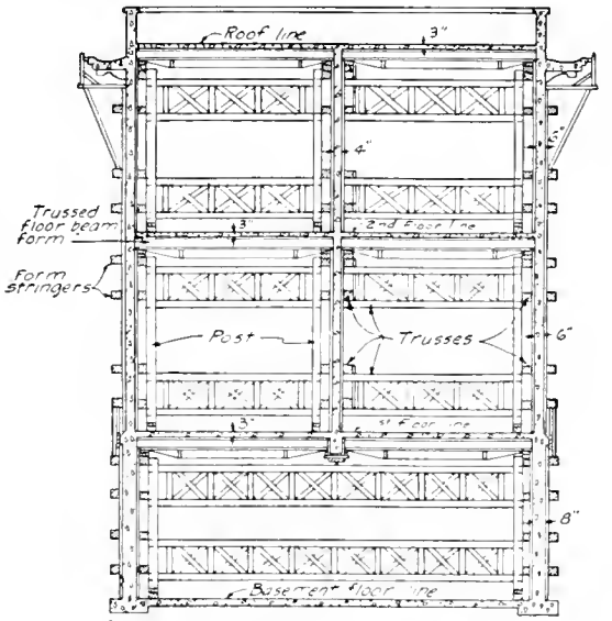
DETAILS OF INGERSOLL STANDARD FORMS
