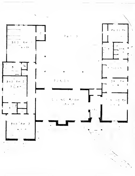
PLAN, HOUSE OF C. A. STRAYER, LOS ANGELES
