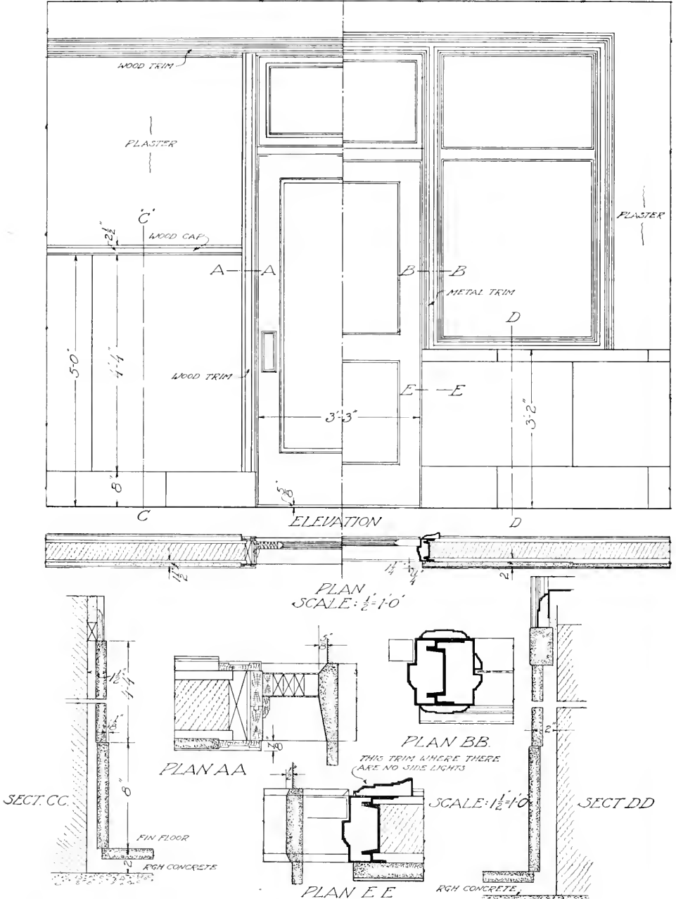
DETAILS FOR MARBLE WAINSCOTING IN OFFICE CORRIDORS
