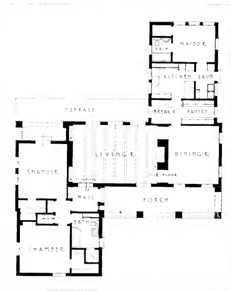
PLAN, HOUSE OF THEODORE CHAPIN, PASADENA Frederick Kennedy, Jr., Architect
