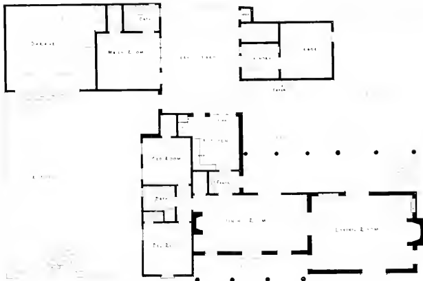
PLAN, RESIDENCE FOR W. P. HERBERT, SANTA MONICA John Byers, Architect
