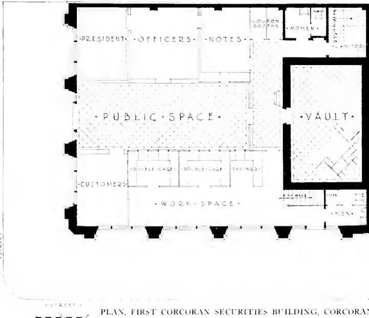
PLAN, FIRST CORCORAN SECURITIES BUILDING, CORCORAN F. Eugene Barton, Architect
