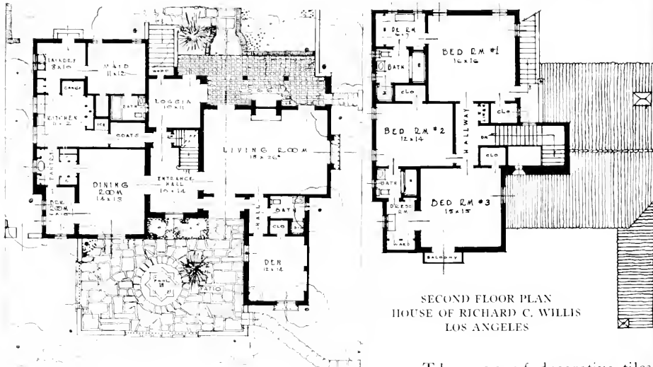
PLAN, HOUSE OF RICHARD C. WILLIS, LOS ANGELES Ralph C. Flewelling, Architect
