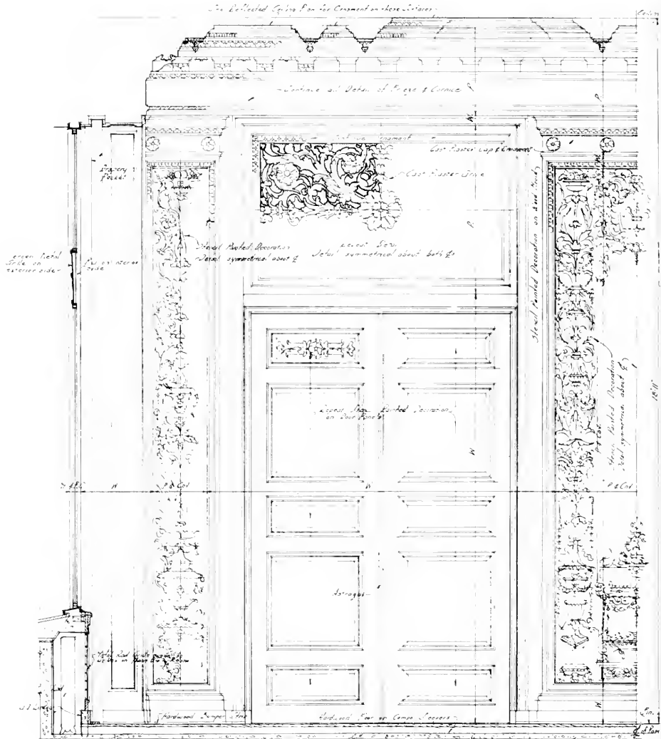
PART EAST ELEVATION. TYPICAL DETAIL OF SMALL DINING ROOM. Scale - 3/4" = 1'
