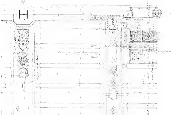
REFLECTED PART PLAN OF BANQUET HALL CEILING
