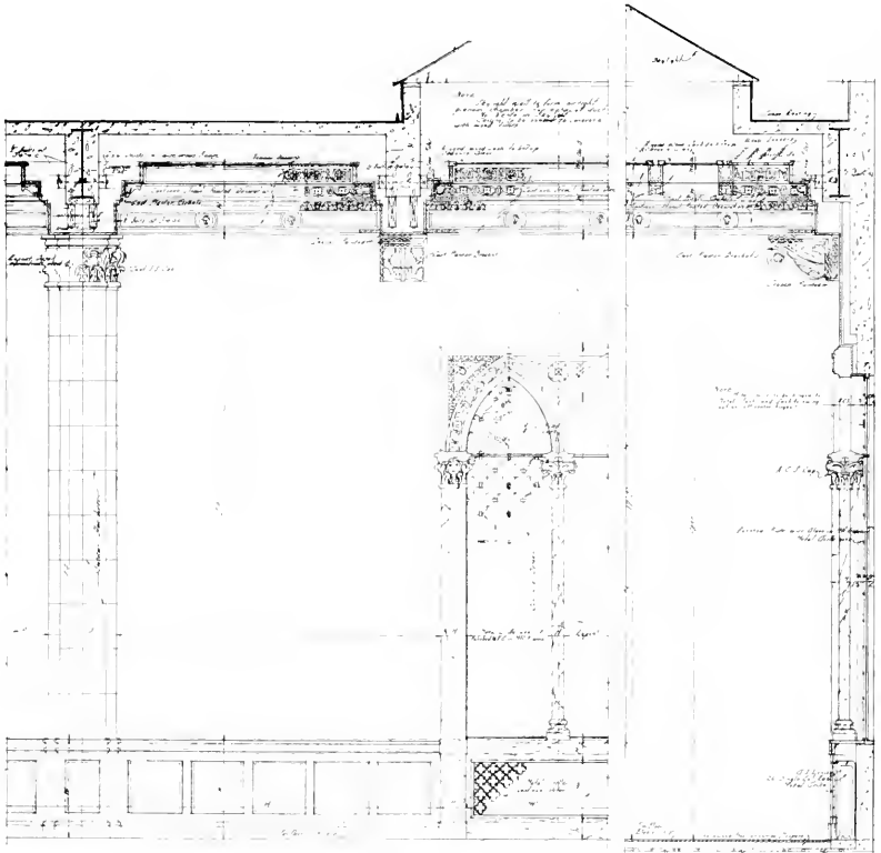
PART ELEVATION OF SOUTH WALL & WINDOW
