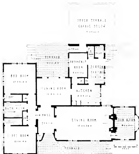
HOUSE OF DR. I. E. HARRIS, ALTADENA, CALIFORNIA BENNETT AND HASKELL, ARCHITECTS
