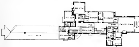
HOUSE OF HAROLD S. CHASE, HOPE RANCH, SANTA BARBARA Reginald D. Johnson, Architect
