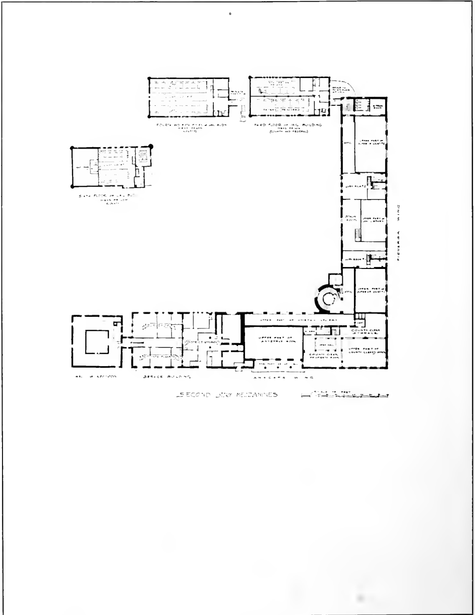
PLAN, SECOND STORY MEZZANINE, COURT HOUSE, SANTA BARBARA WILLIAM MOOSER CO., ARCHITECTS
