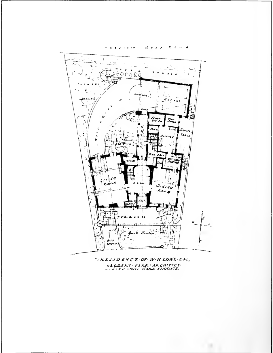
GROUND PLAN, HOUSE OF W. H. LOWE, SAN FRANCISCO ALBERT FARR, ARCHITECT; J. FRANCIS WARD, ASSOCIATE
