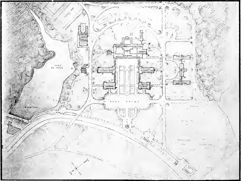
PLOT PLAN, ST. MARY'S COLLEGE, CALIFORNIA John J. Donovan, Architect
