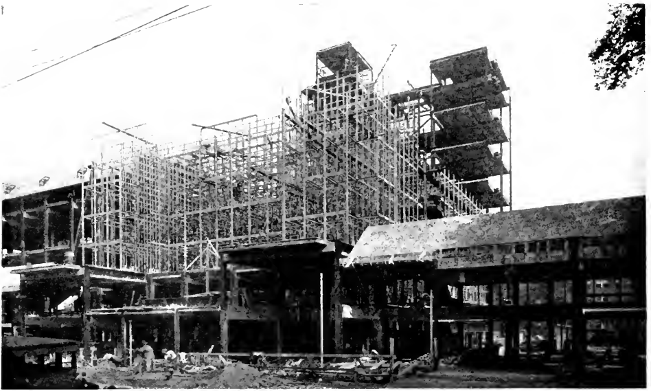
YALE UNIVERSITY LIBRARY, NEW HAVEN CONNECTICUT Arc Welded Construction Under Westinghouse Supervision
