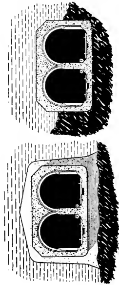
TUBES WOULD BE BUILT IN SECTIONS ASHORE, TOWED TO SITE AND SUNK INTO POSITION ON THE PIERS, AFTER THE SAME MANNER AS THE SECTIONS TO THE OAKLAND-ALAMEDA TUBE
