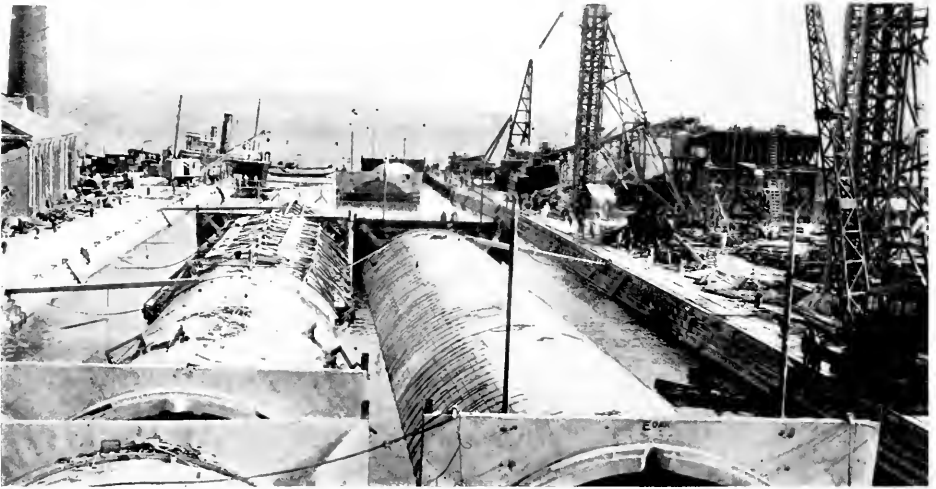
FOUR PRECAST SEGMENTS FOR GEO. A. POSEY TUBE Drydock Flooded for Removal of Completed Segment
