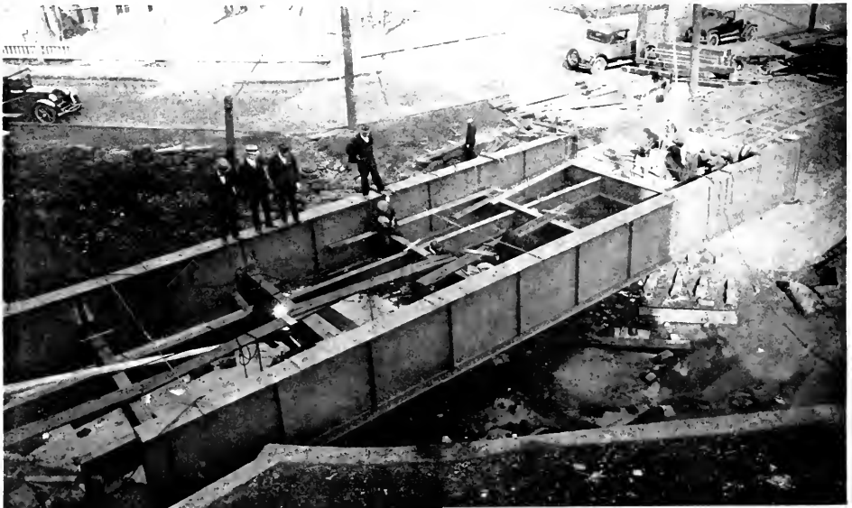
FIRST WELDED PLATE GIRDER BRIDGE, TURTLE CREEK, PENNSYLVANIA
