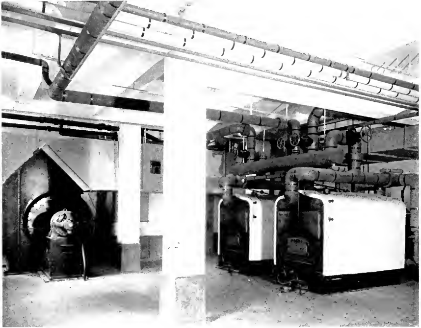
Boiler Room, showing Ventilating Fan and Heating Equipment, Santa Barbara County Court House, Santa Barbara, California WILLIAM MOOSER CO., Architects and Managers of Construction
