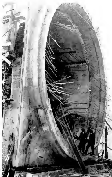
END OF COMPLETED CONCRETE SEGMENT Showing Collar and Inside Joint Lap Reinforcement
