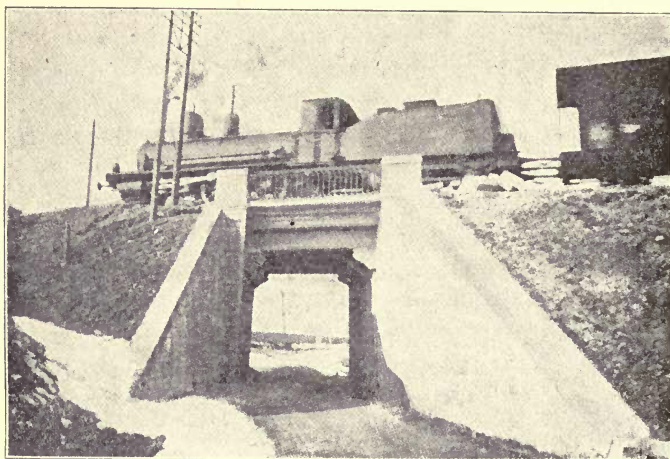
Fig. 142.—Reinforced Concrete Girder Railroad Bridge.
