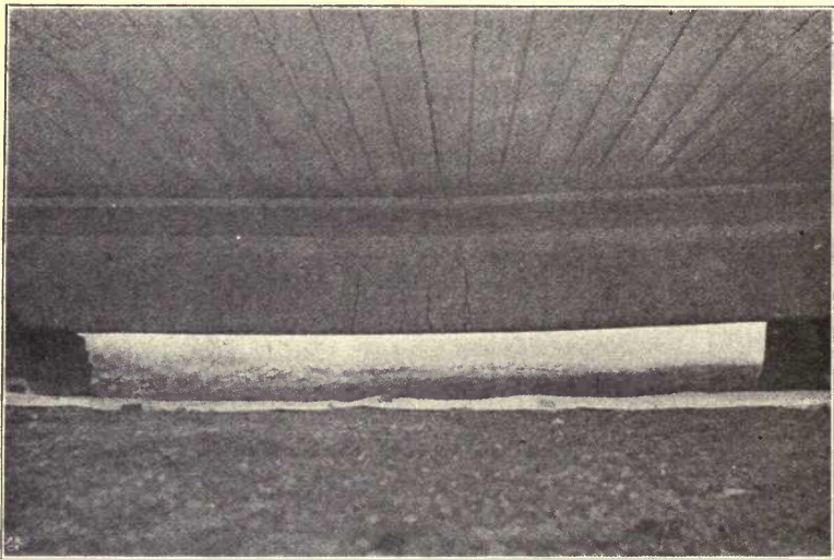
Fig. 6.—This Beam was designed for a super-imposed load of 4 tons, and was tested by a load of 34 tons. It cracked in the center and deflected considerably; nevertheless, it carried the load for 4 years without further sign of weakness.
