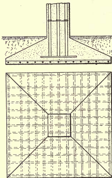
Fig. 49.—Reinforced Concrete Column Footing.
