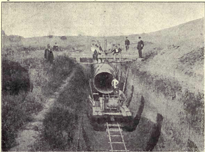
Fig. 121.—Pipe of 5 feet 9 inches diameter. Paris Sewage Disposal System.
