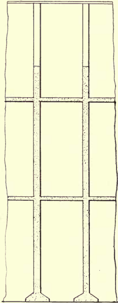
Fig. 95.—Section of Dam 50 feet high with two Platforms built on Rock.
