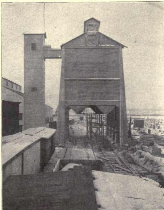
Fig. 112.—Storage Bins, Hecla Portland Cement Co.
