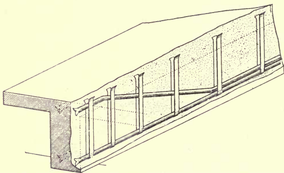
Fig. 3.—Perspective View of Armored Concrete Girder.
