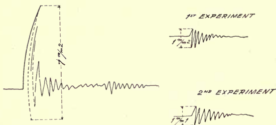
Fig. 87.—Vibration Diagrams.
