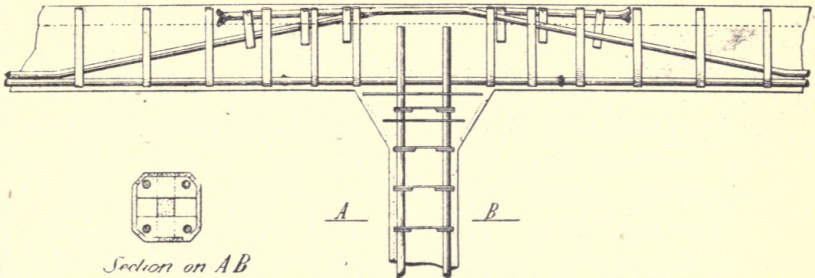
Fig. 4.—Connection of a Continuous Girder to a Column.
