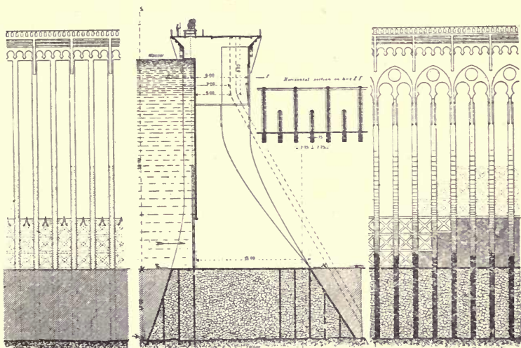
Fig. 96.—Design for the Nile Dam at Assuan, of Reinforced Concrete, 100 feet high.
