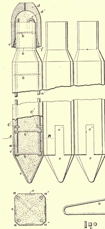
Fig. 55.—Details of Reinforced Concrete Piles.
