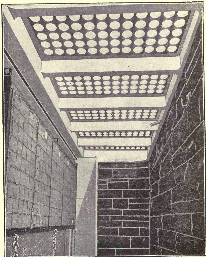
Fig. 140.—View of Reinforced Concrete Side-walk Lights from below.
