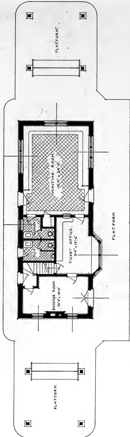
FIRST AND SECOND FLOOR PLANS— RAILWAY STATION AT BALDWIN, L. I. FRANK J. FORSTER, ARCHITECT.
