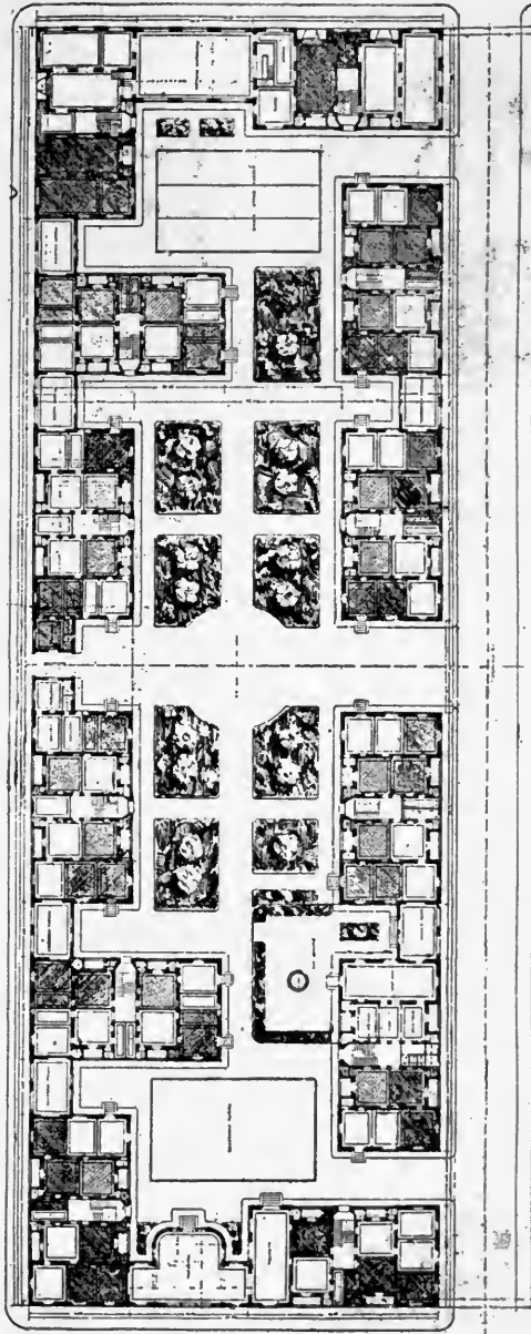
GROUND FLOOR AND SECOND FLOOR PLAN OF ROTTOLE HOUSING DEVELOPMENT, MILAN, BY THE UMANITARIA SOCIETY.
