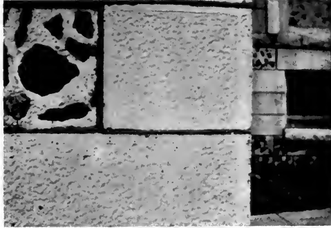
An Excellent and a Poor Example of Concrete Finish. The Corner Stones Are Finished With the Pointer and Appear Well. The other Stones Have Aggregate of Too Large Size Impressed Into Surface.
