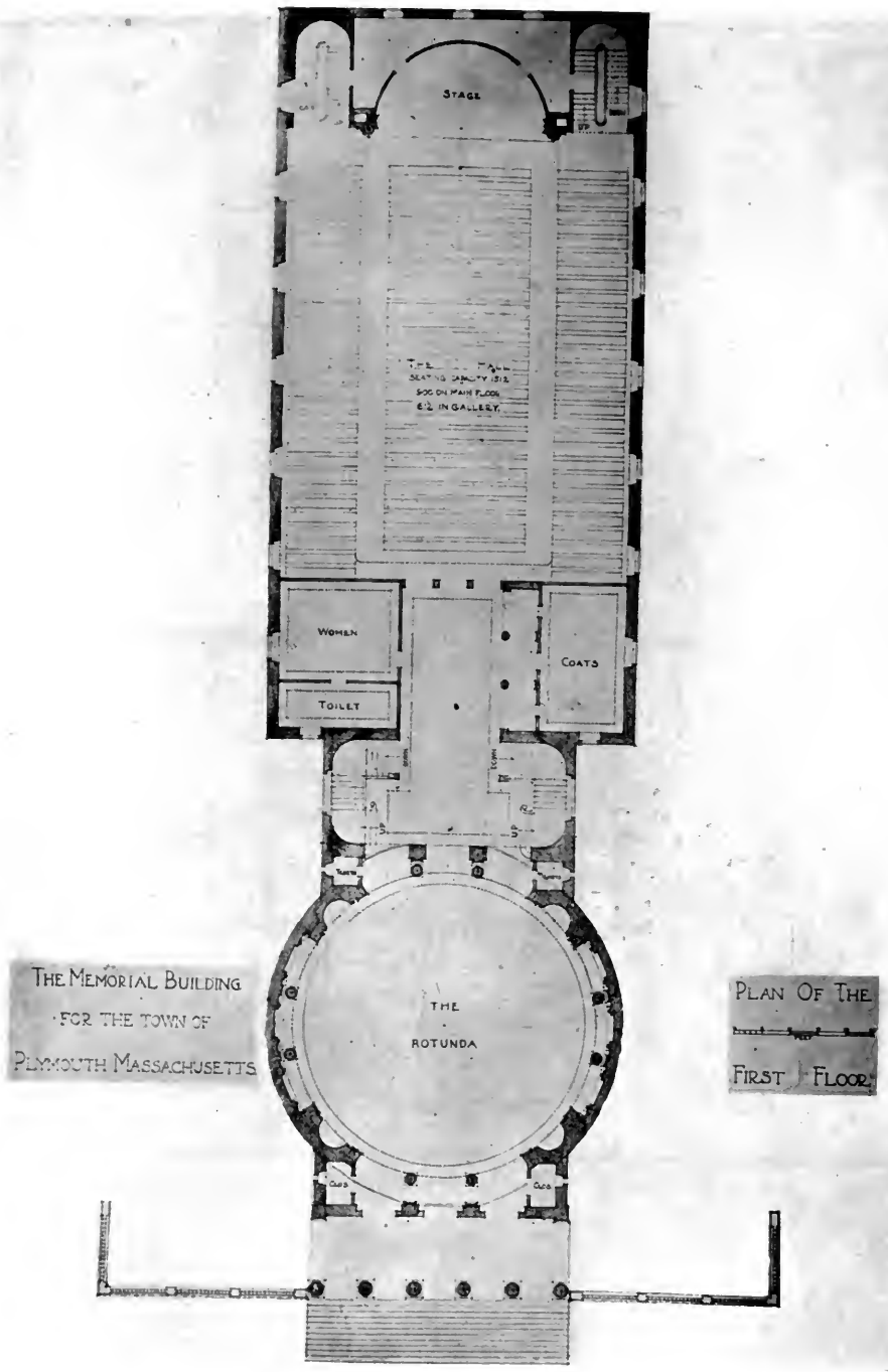
WINNING DESIGN IN A COMPETITION FOR PROPOSED MEMORIAL COMMUNITY BUILDING AT PLYMOUTH, MASS. LITTLE & RUSSELL, ARCHITECTS
