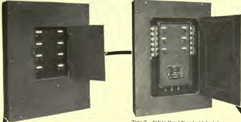
Type T—Safety Panel Board with Inner Door open, giving access to switches.
