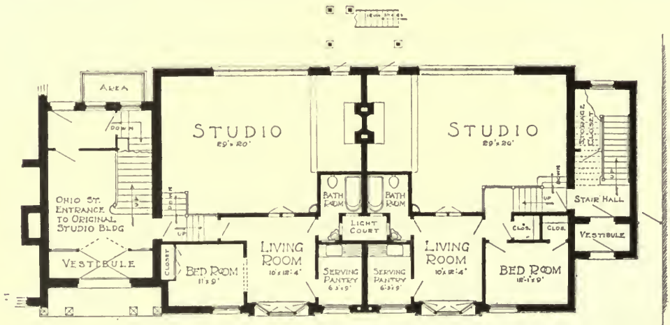
FIRST STORY PLAN FIG. 114. ANNEX NO. 1—TREE STUDIOS, CHICAGO, ILL. Woltersdorf & Bernhard, Architects.
