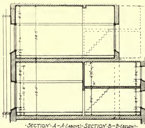
SECTION-A-A-(ABOVE)-SECTION-B-B-(BELOW). FIG. 121. CROSS SECTION THROUGH STUDIOS, 120 RIVERWAY, BOSTON, MASS., William D. Austin, Architect.
