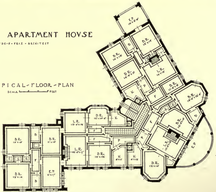
FIG. 138. — EXTERIOR AND FLOOR PLAN OF LOMBARDY APARTMENT HOUSE, BALTIMORE, MD.
