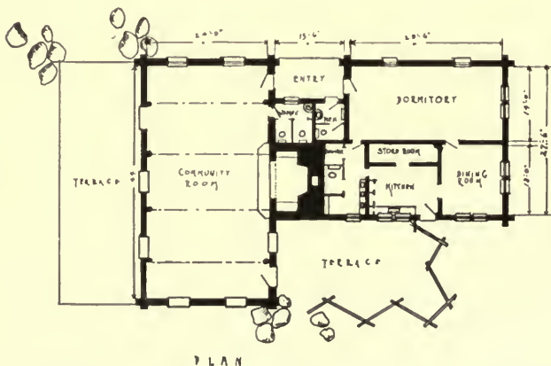
COMMUNITY ROOM AND RANGERS' QUARTERS, YELLOWSTONE NATIONAL PARK.
