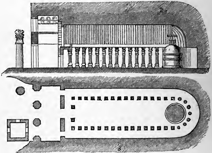
FIG. 40.—CHAITTA NEAR POONA.
