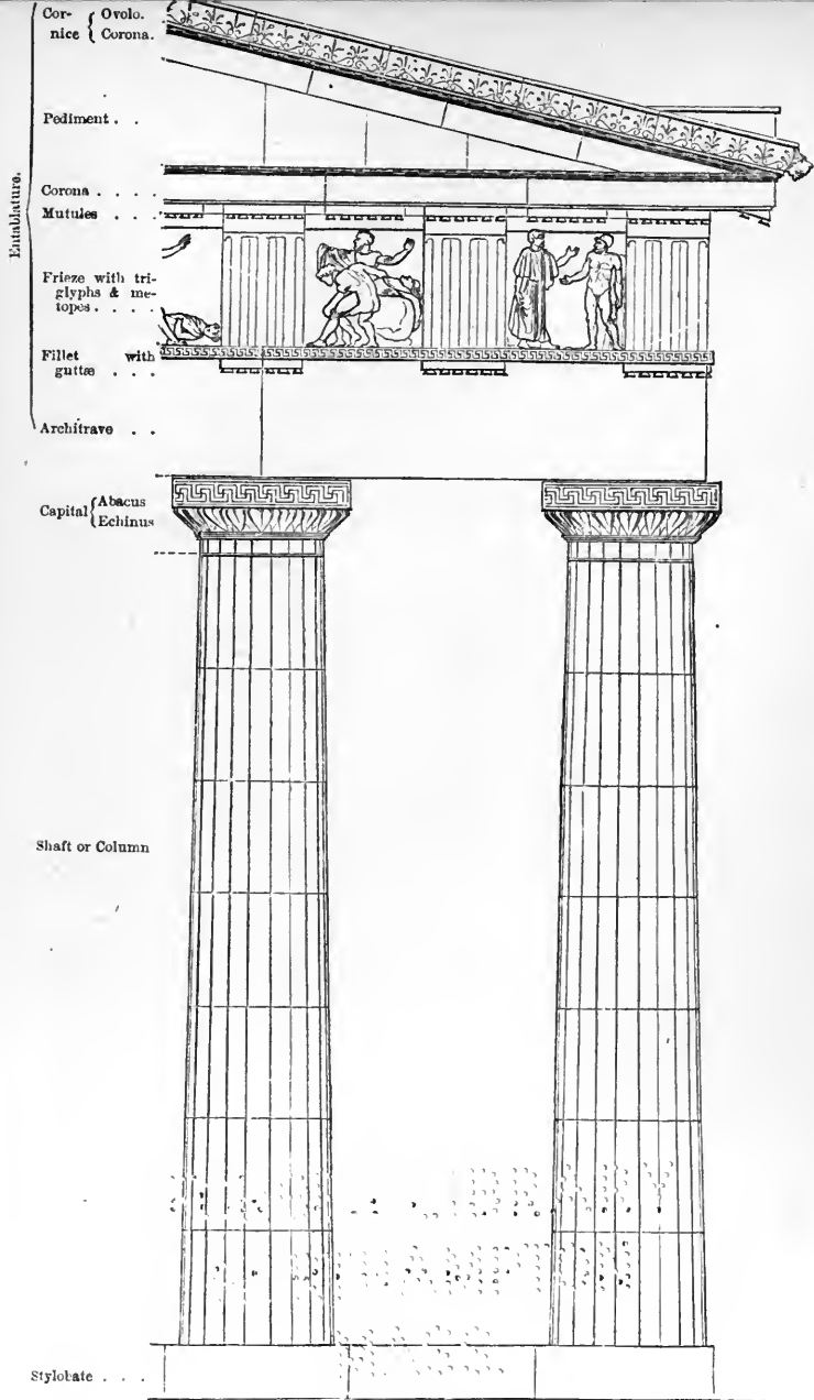
FIG. 57.—THE GREEK DORIC ORDER FROM THE THESEUM.
