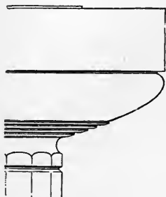
FIG. 53.—GREEK DORIC CAPITAL FROM SELINUS.
