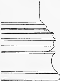
FIG. 74.—IONIC BASE FROM THE TEMPLE OF THE WINGLESS VICTORY (NIKÉ APTEROS).
