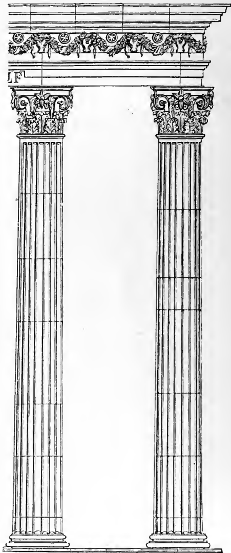
FIG. 123.—CORINTHIAN ORDER FROM THE TEMPLE OF VESTA AT TIVOLI.
