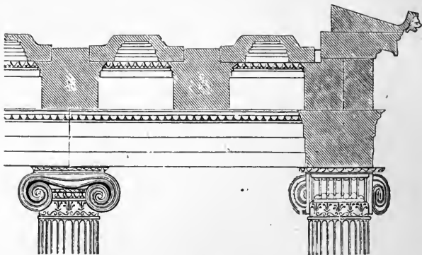
FIG. 88.—SECTION OF THE PORTICO OF THE ERECHTHEIUM.
