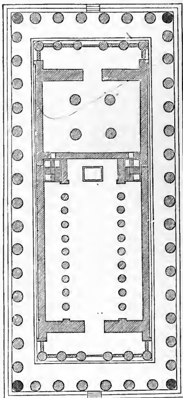
FIG. 55.—PLAN OF THE PARTHENON AT ATHENS.
