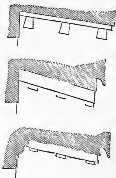
FIG. 64.—DETAILS OF THE METULES.
