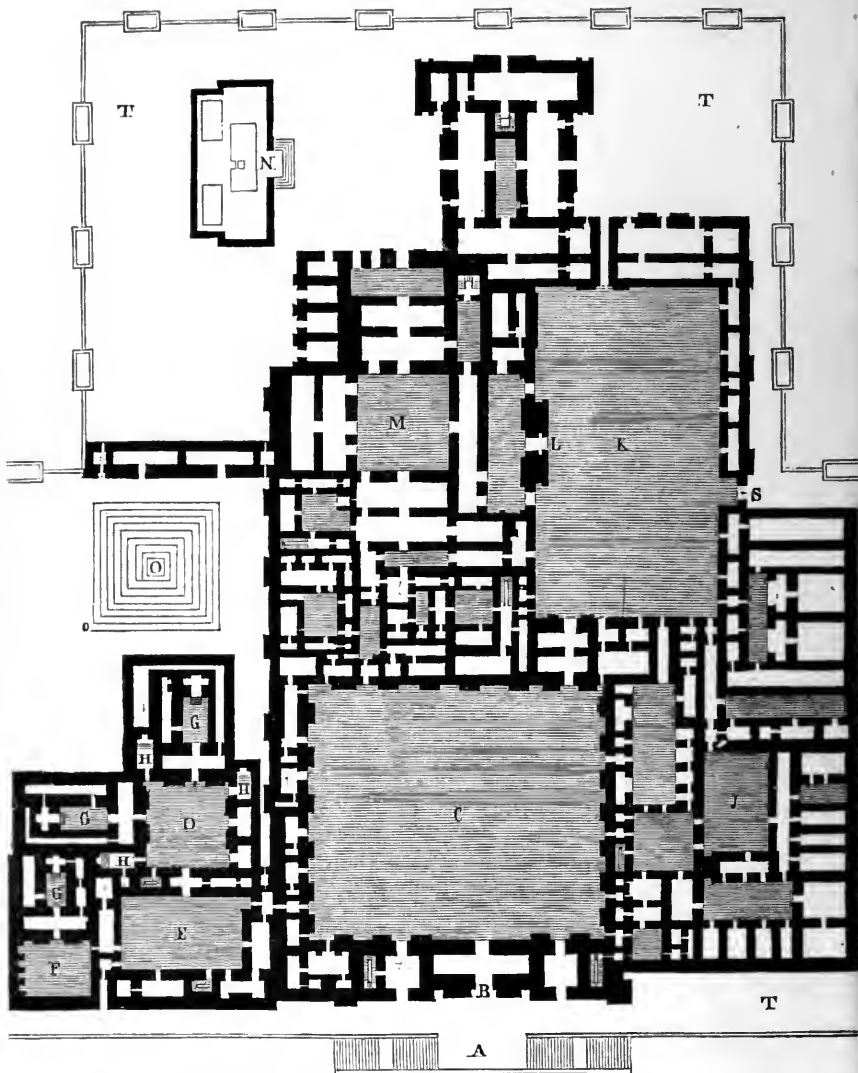
FIG. 32.—PALACE OF KHORSABAD. BUILT BY KING SARGON ABOUT 710 B.C.
