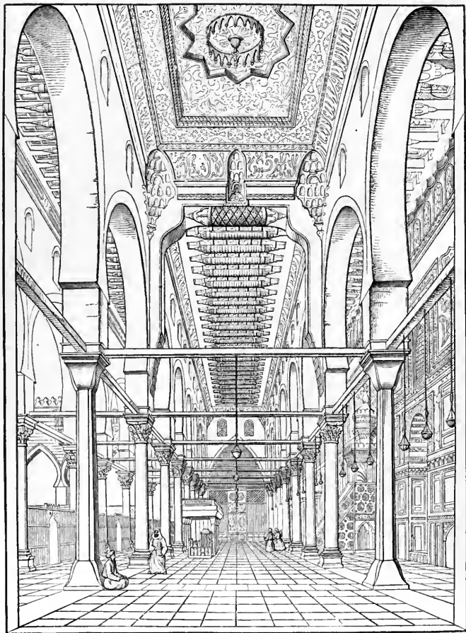
FIG. 189.—Mosque 'EL MOYED' AT CAIRO.
