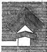
FIG. 10.—THE SEPULCHRAL CHAMBER IN THE PYRAMID OF CEPHREN AT GIZEH.
