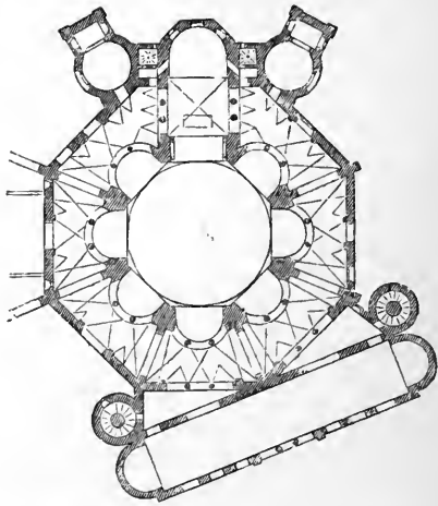
FIG. 160.—PLAN OF SAN VITALE AT RAVENNA.
