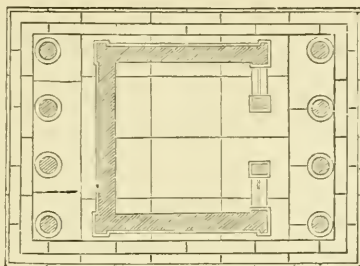
F.G. 50A.—PLAN OF A SMALL GREEK TEMPLE.
