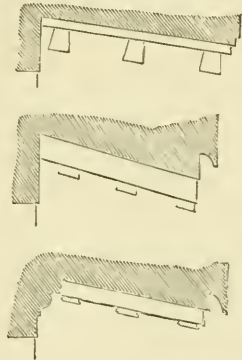
FIG. 61.—DETAILS OF THE MUTULES.
