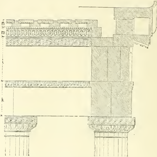
FIG. 61.—SECTION OF THE ENTABLATURE OF THE GREEK DORIC COLUMN.
