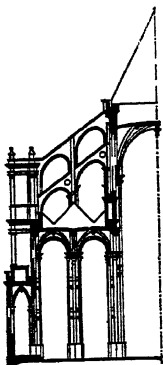
84. HALF CROSS-SECTION.
