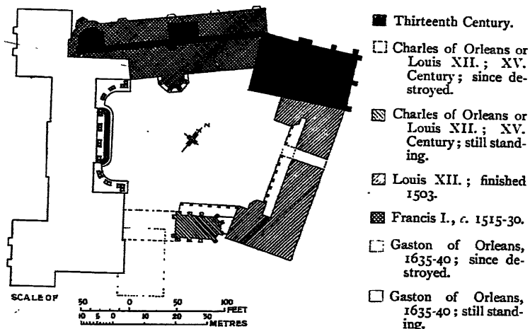
48. CASTLE OF BLOIS: PLAN.
