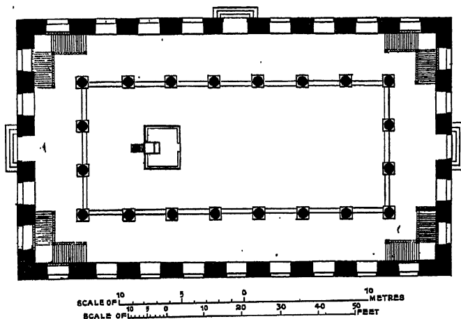
248. CHARENTON: "TEMPLE" OR PROTESTANT CHURCH, BY S. DE BROSSE (1623, DESTROYED 1686). SECTION AND PLAN. FROM MAROT.
