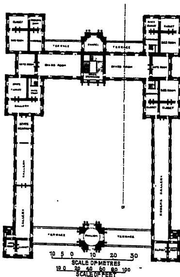
231. LUXEMBOURG PALACE: PLAN.
