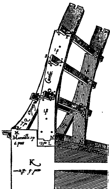
133. PHILIBERT DE L'ORME'S SYSTEM OF ROOF CONSTRUCTION.
