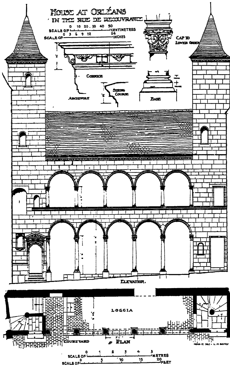
76. ORLEANS: HOUSE IN RUE DE RECOUVRANCE KNOWN AS "MAISON DE FRANÇOIS I." (1536-50): LEFT SIDE OF COURT. PLAN AND ELEVATION.
