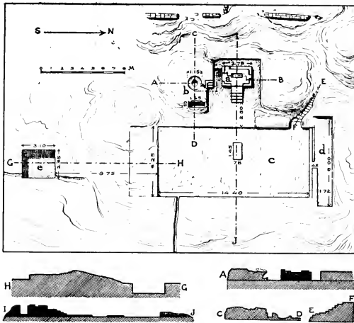
FIG. 215. PLAN OF THE HIGH PLACE AT PETRA (after Brünnow).
