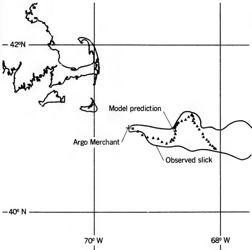
Figure 2-12. Predicted and observed location and shape of oil slick, December 22. Model prediction shows oil released from the Argo Merchant from 1000, December 17, through 1000, December 22. Wind input is from Nantucket Light Ship.
