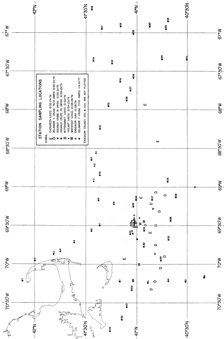
Figure 3-3. Water sampling locations.
