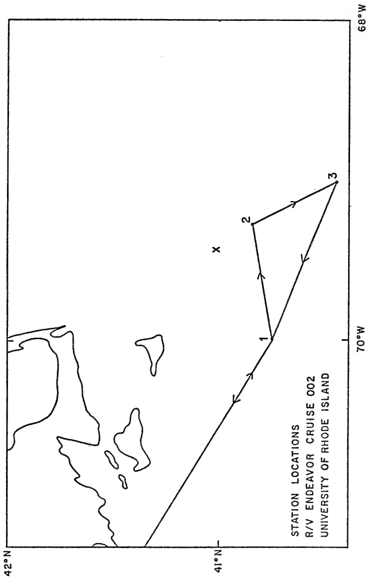
Figure 3-4. Stations where samples for total extractable organics were taken during Endeavor cruise 002.
