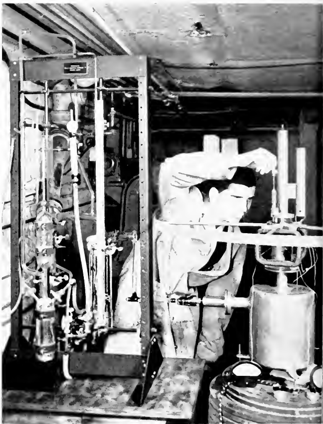
Special Knudsen-type direct reading high vacuum gauge developed for study of vacuum pumps.
