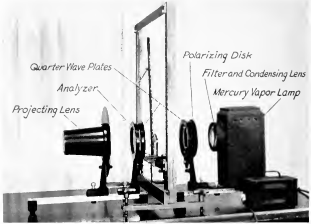
FIG. 6—Polariscope with component parts indicated.
