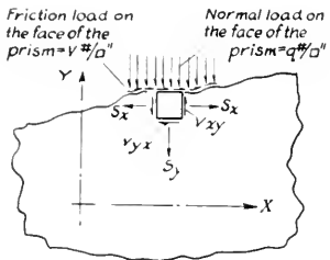
FIG. 5—General condition of loading and stress on an elemental prism having one face in the boundary.
