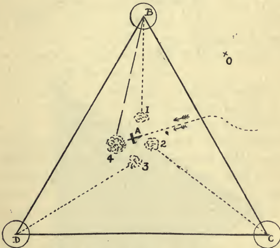
FIG. 13.—THE GERMAN METHOD OF PICKING UP THE RANGE WITH ANTI-AIRCRAFT GUN-FIRE. (Plan View.)
