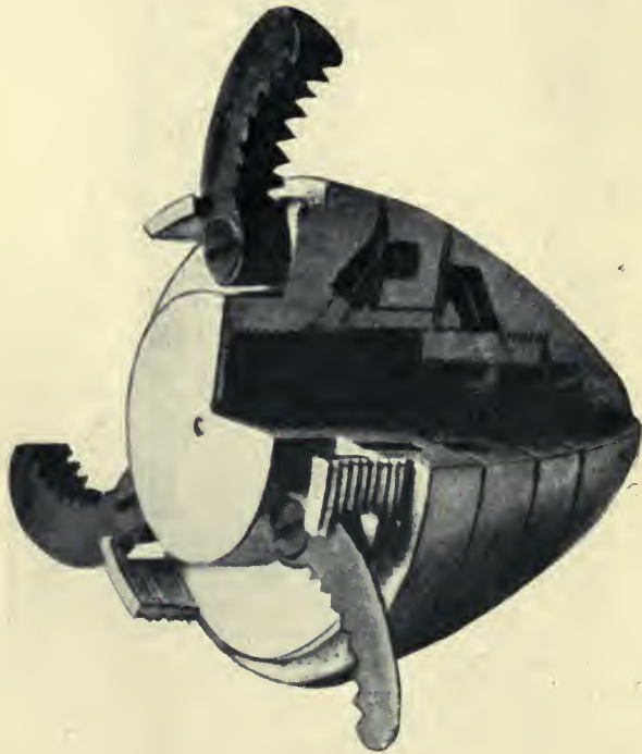
NOSE OF THE GRENADE SHOWING FUSE-HEAD MECHANISM.
