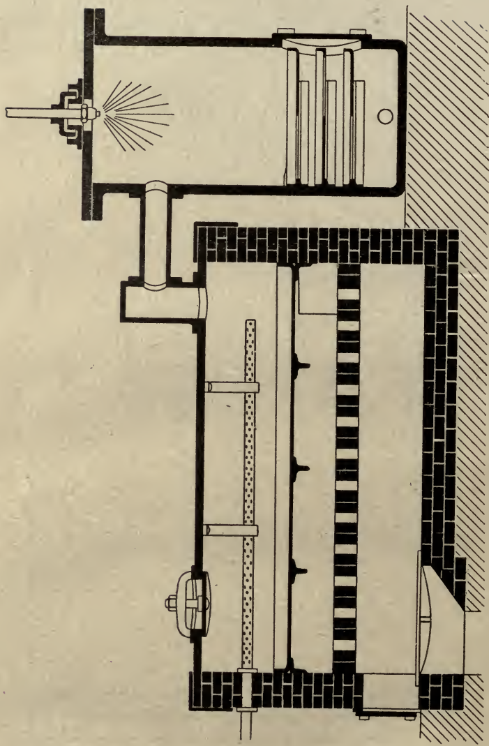
FIG. 11.—Anthracene Subliming Plant.
