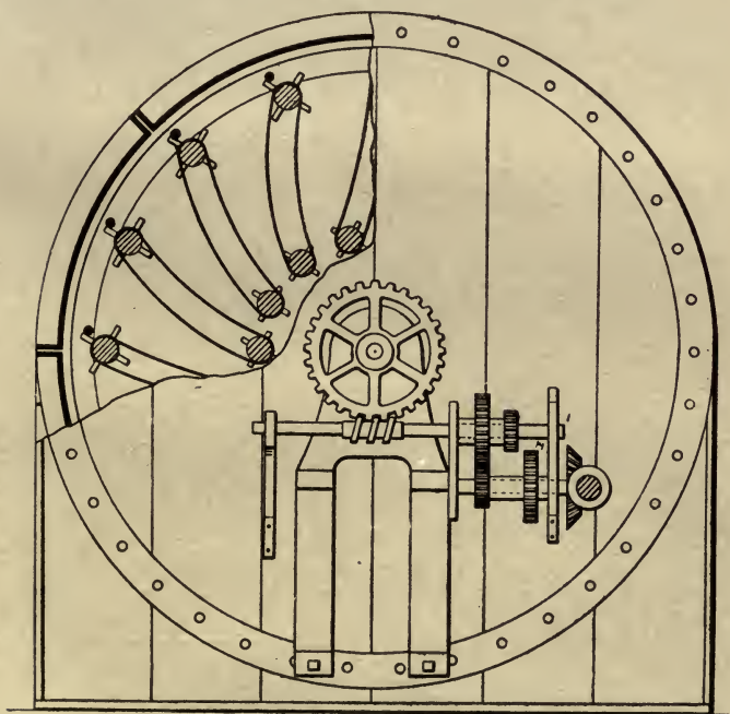
FIG. 19.—Hank-Dyeing Machine.
