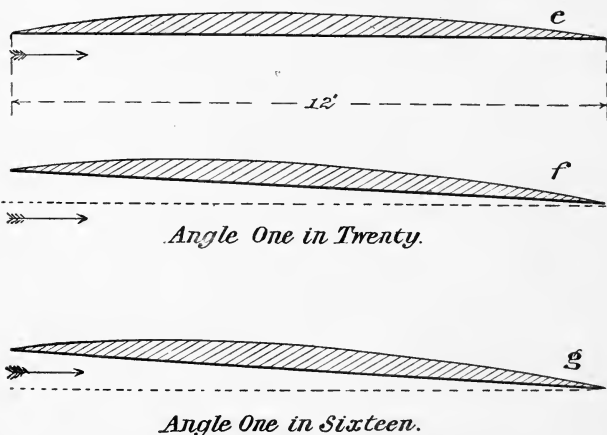
Fig. 26.—A flat aeroplane placed at different angles.
