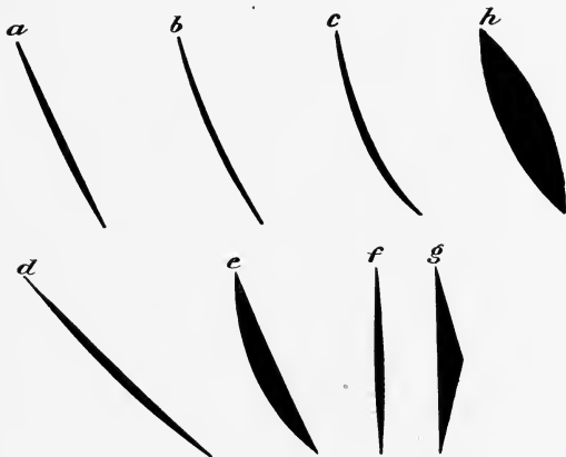
Fig. 14.—This drawing shows the ends of screw blades in which a is a plain screw; b , screw with increasing pitch; c , screw with compound increasing pitch; d , end of screw blade 45^\circ ; e , screw with very thick blade; f , blade with no pitch at all; g , blade which gave a thrust in the direction of the convex side, no matter in which direction it was revolved; h , screw said to have been used in the French Government experiments.
