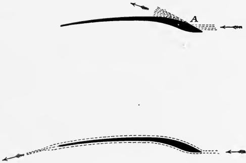
Fig. 88.—The very narrow aeroplanes, or sustainers, employed by Mr. Philipps. It has been supposed that the air in striking at A was deflected in the manner shown, but such is not the case. The air in reality follows the surface, as shown in the dotted line in the second illustration.
