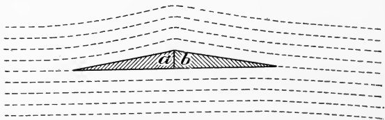
Fig. 65.—The aerofoil here shown is a mathematical paradox. This aerofoil lifts, no matter in which direction it is driven. It encounters air which is stationary and leaves it with a downward trend; therefore it must lift. However, if we remove the section b , and only subject a to the blast, as shown at Fig. 66, no lifting effect is produced. On the contrary, the air has a tendency to press a , downwards. The path which the air takes is clearly shown; this is most important, as it shows that the shape of the top side is a factor which has to be considered. All the lifting effect in this case is produced by the top side.
