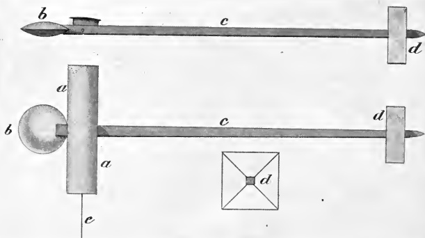
Fig. 39.—Apparatus for testing the lifting effect of aeroplanes at a low angle and extremely high velocity. a , a , the aeroplane; b , lead weight; c , long and slender pine rod; d , tail for keeping the apparatus head on and ensuring its travelling straight through the air; e , the point of suspension, also the centre of gravity. When this apparatus was travelling at the rate of 80 miles an hour, it gave a lifting effect of about 36 lbs., which is about 7 lbs. per square foot.
