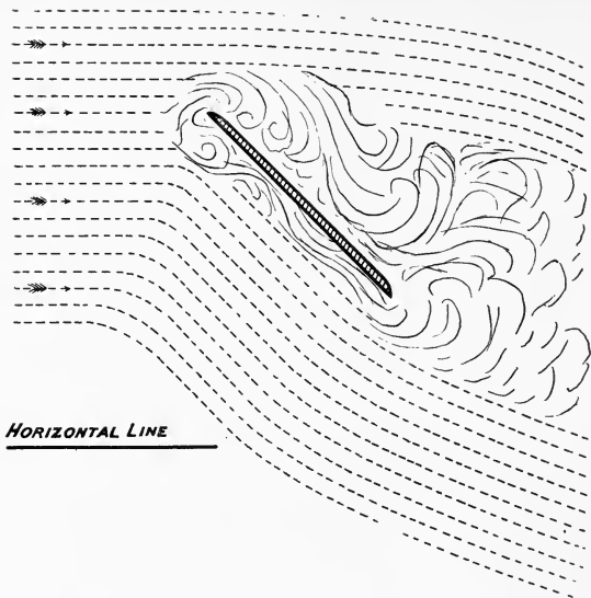
Fig. 64.—Shows a flat aerofoil placed at an angle of 45^\circ , an angle which will never be used in practical flight, but at this angle the momentum of the approaching air and the energy necessary to give it an acceleration sufficiently great to make it follow the back of the aerofoil are equal, and at this point, the wind may either follow the surface or not. Sometimes it does and sometimes it does not. See experiments with screws.
