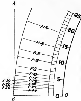
Fig. 72a.—Angles and degrees compared. It will be observed that an angle of 1 in 4 is practically 14^{\circ} .
