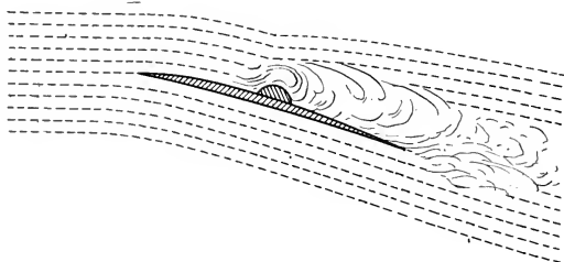
Fig. 63.—Section of a screw blade having a rib on the back. The resistance caused by this rib is erroneously supposed to be skin friction.
