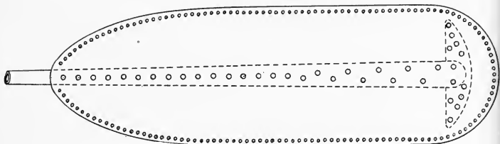
Fig. 19. — Shows the form of the blade of a screw propeller made of sheet metal. It is riveted at the edges and also to the arm of a screw with a stiffening piece at the extreme end. However, it is not necessary to rivet edges together. They may be welded with a flame of acetylene oxygen gases.
