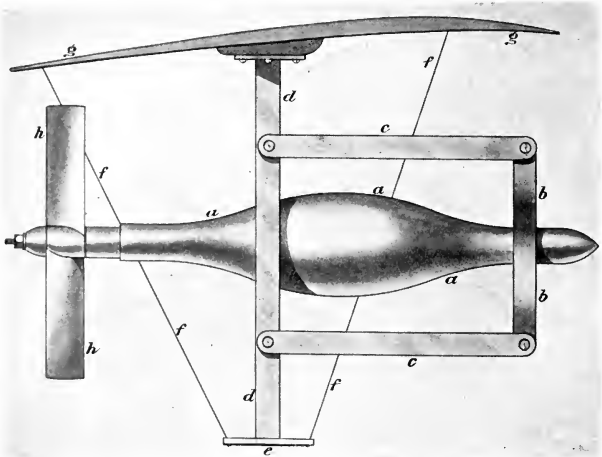
Fig. 36.—The machine attached to the end of the rotating shaft— a, a , the body of the machine; b, b , four-legged spider secured to a, a ; c, c , parallel bars; d, d , vertical member to which the aeroplane g, g is attached; h, h , the screw; f, f , wires for preventing distortion of the aeroplane.
