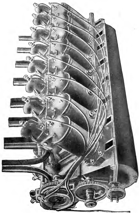
Fig. 49.—The Antoinette motor.
