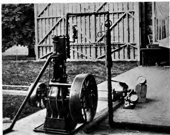
Fig. 35.—The little steam engine used by me in my rotating arm experiments; the tachometer and dynamometer are distinctly shown.
