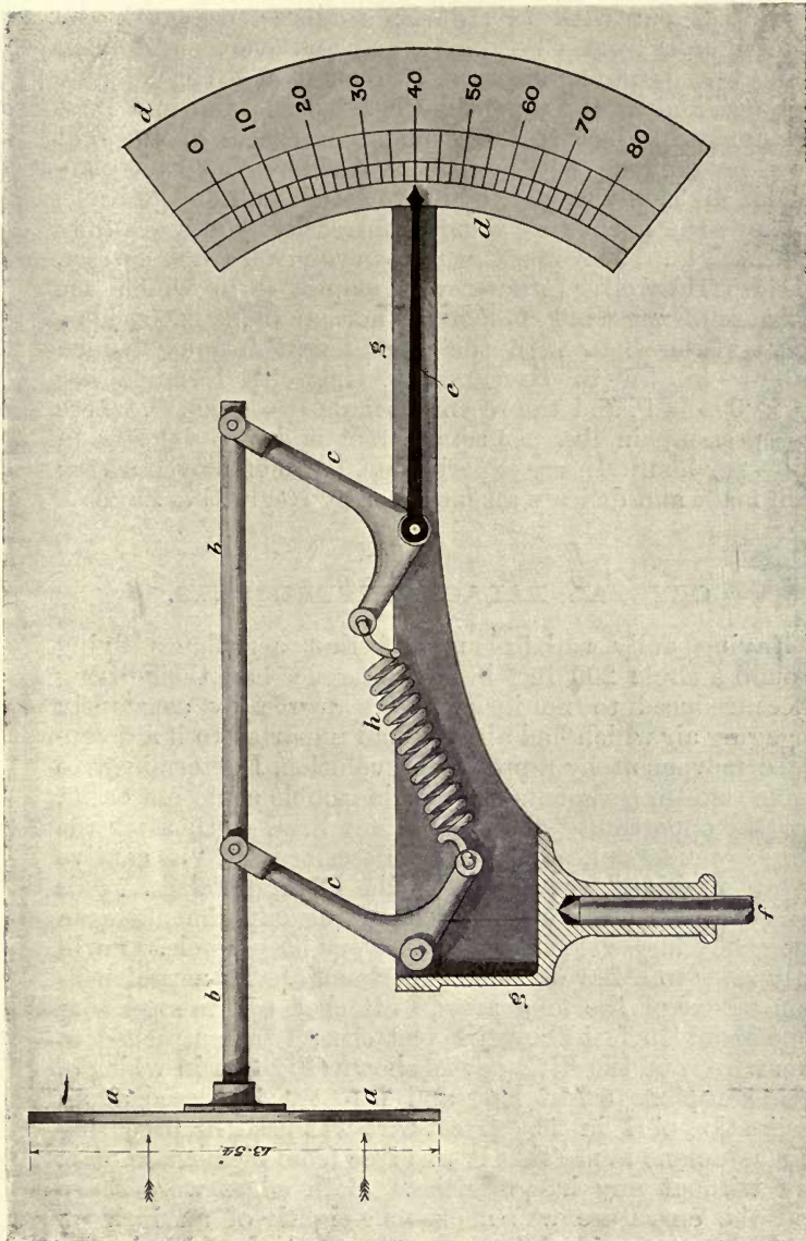
Fig. 33.—Apparatus for indicating the force and velocity of the wind direct without any timing, counting, or mathematical calculations.
