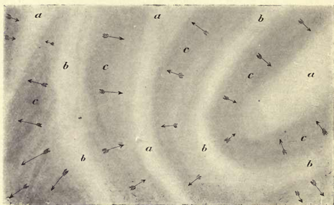
Fig. 6.—Air currents observed in the Mediterranean, ascending current at a, a, a , and descending currents at b, b, b .
