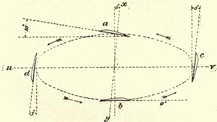
Fig. 44.—Shows the position of the blades of a hélicoptère as they pass around a circle, when the angle of the shaft and the angle of the blades are the same.
