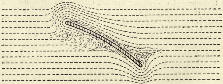
Fig. 59.—An illustration from another scientific publication also on the Dynamics of Flight. It will be observed that the air in striking the underneath side of the aeroplane is divided into two streams, a portion of it flowing backwards and over the top of the edge of the aeroplane where it becomes compressed. An eddy is formed on the back and top of the aeroplane, and the air immediately aft the aeroplane is neither rising nor falling. Just how these mathematicians reason out that the air in striking the front of the aeroplane would jump backwards and climb up over the top and leading edge against the wind pressure is not clear.
