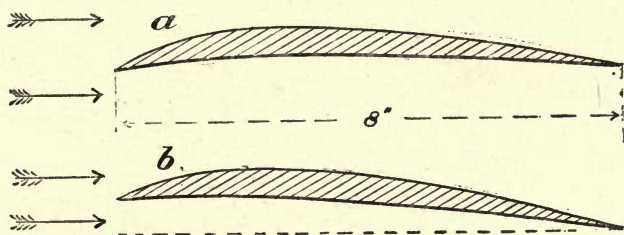
Fig. 28.—An 8-inch aeroplane which did very well. This aeroplane gave decided lifting effect when the bottom side was placed dead level, as shown at a .
