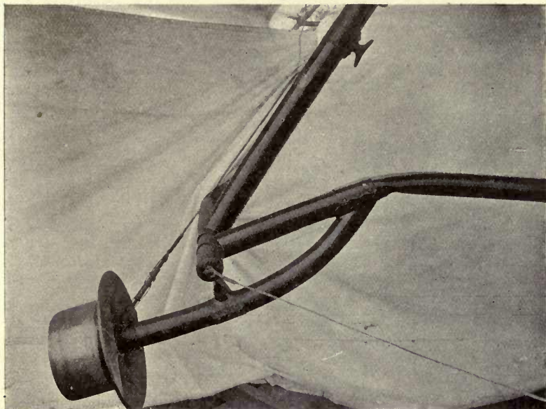
Fig. 80.—The outrigger wheel that gave out and caused an accident with the machine.
