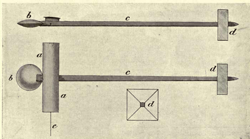
Fig 39.—Apparatus for testing the lifting effect of aeroplanes at a low angle and extremely high velocity. a , a , the aeroplane; b , lead weight; c , long and slender pine rod; d , tail for keeping the apparatus head on and ensuring its travelling straight through the air; e , the point of suspension, also the centre of gravity. When this apparatus was travelling at the rate of 80 miles an hour, it gave a lifting effect of about 36 lbs., which is about 7 lbs. per square foot.
