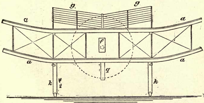
Fig. 40.—Front elevation of proposed aeroplane machine— a, a , the aero-planes; g, g , condenser; f , the engine; q , guard for screw; k, k , support for wheels.
