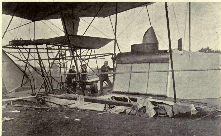
Fig. 82.—The condition of the machine after the accident. One of the broken planks that formed the upper track is shown. It will be observed that the wheels have sunk directly into the ground without leaving any tracks, showing that the machine did not run along the ground, but came directly down when it stopped.
