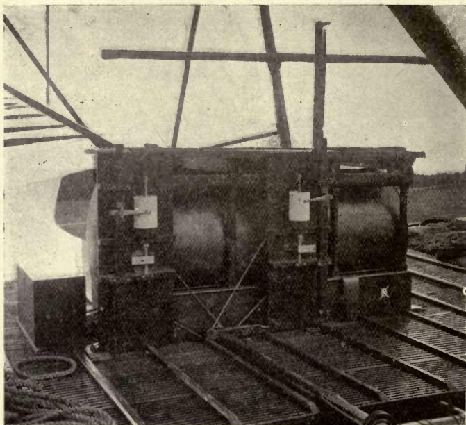
Fig. 79.—Two dynamographs, one for making a diagram of the lifting effect off the main axle-tree, and the other for making a diagram of the lift off the front axle-tree. By this arrangement, I was able to ascertain the exact lifting effect at all speeds, and to arrange my aeroplanes in such a manner that the center of lifting effect was directly over the center of gravity. The paper-covered cylinders made one rotation in 2,000 feet.
