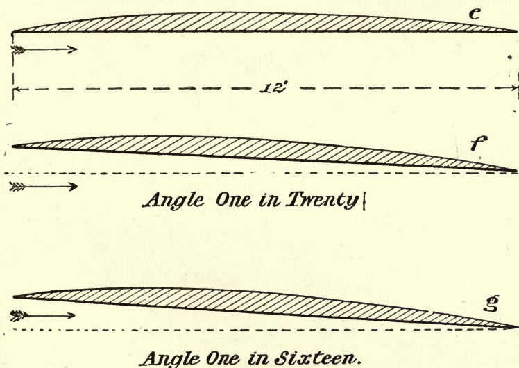
Fig. 26.—A flat aeroplane placed at different angles.
