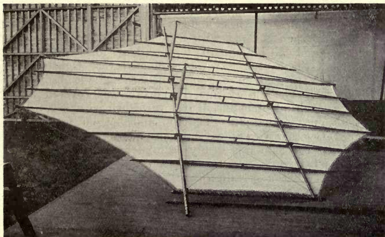
Fig. 76.—The forward rudder of my large machine, showing the fabric attached to the lower side. The top was also covered with fabric. This rudder considered as an aeroplane had a very high efficiency and worked very well indeed.
