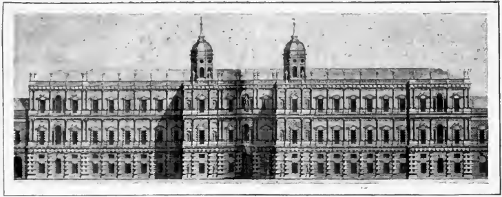
FIG. 171.—WHITEHALL. CENTRAL BLOCK OF NORTH FRONT, AS DESIGNED BY INIGO JONES.
