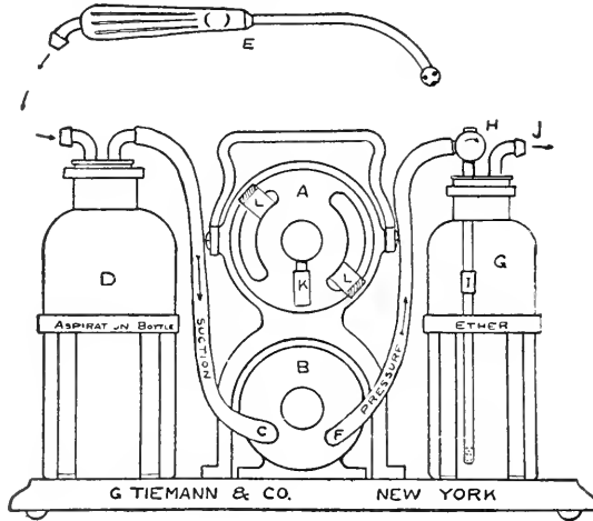
FIG. 132.—Electrical aspirator.
