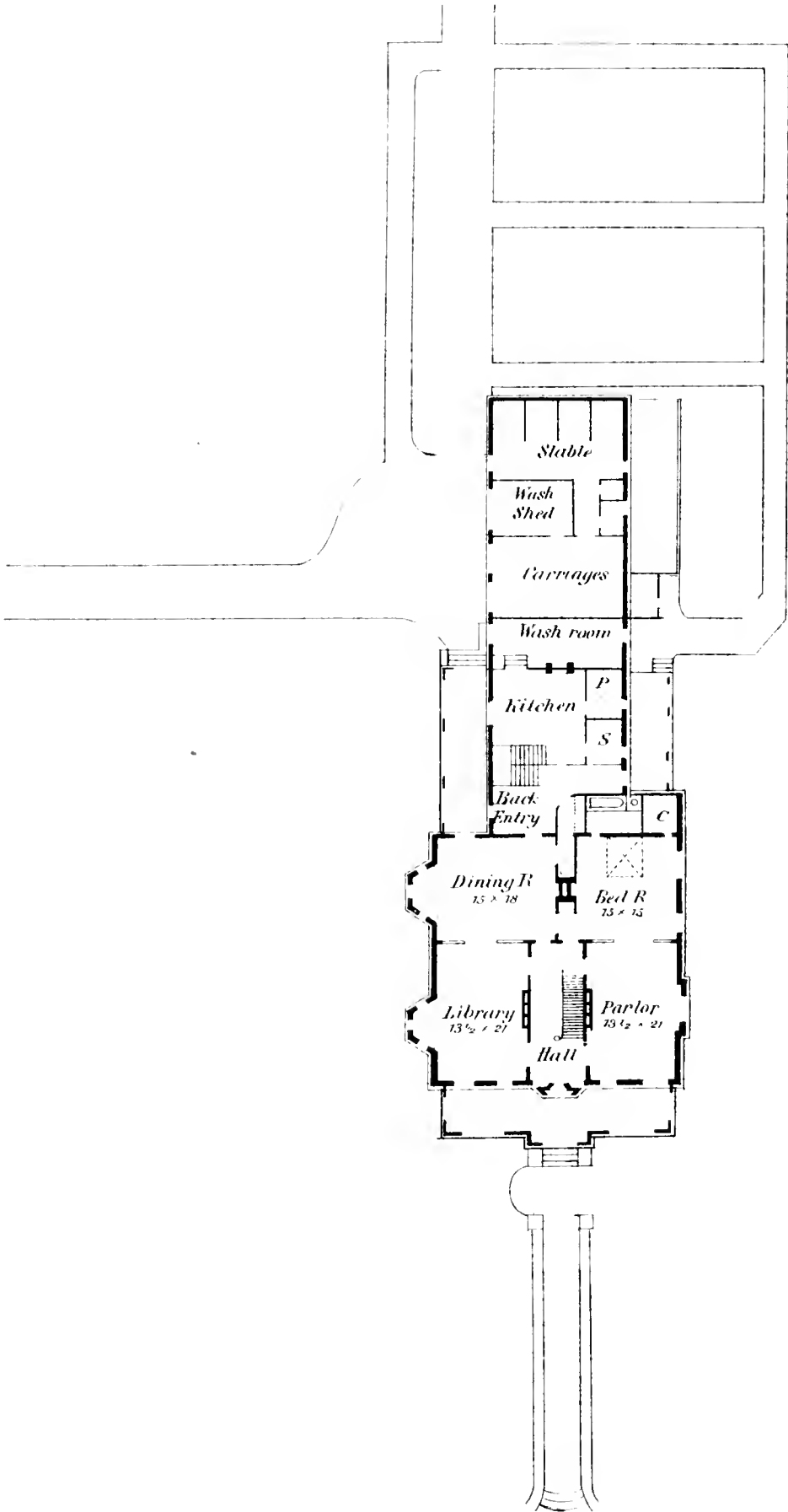
Scale \frac{1}{4} inch = 1 foot.
