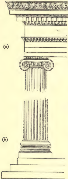
Fig. 10. (a) IONIC ENTABLATURE; (b) IONIC BASE (ASIATIC TYPE).
