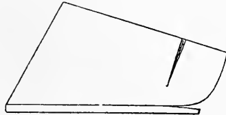
Fig. 110.—Bearing relieved at wrong place by "springing" the heel.
