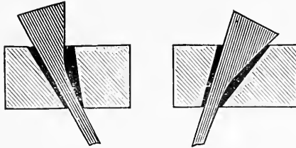
Fig. 50.—Nail-holes "pitched" in and out.
