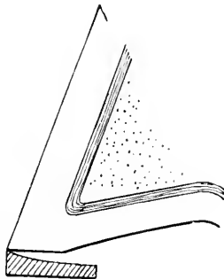
Fig. 74.—Section of a "saucer" shoe.
