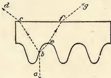
Fig. 73.—Diffusing Curves of Holophane.
