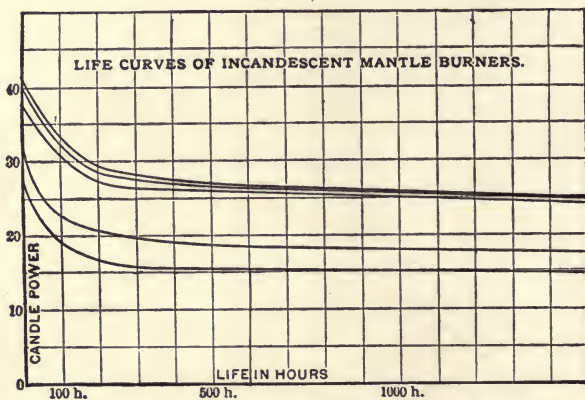
Fig. 27.—Life Curves, Welsbach Mantles.
