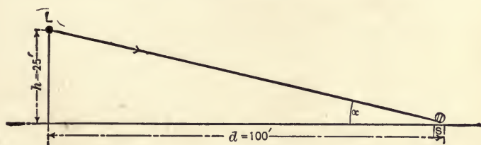
Fig. 95.—Illumination at a Surface.
