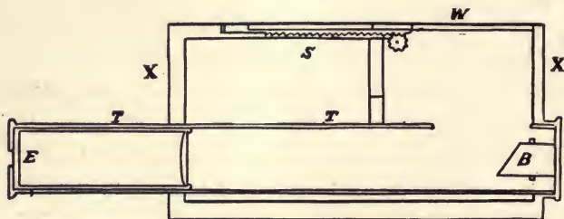
Fig. 127.—Illuminometer.
