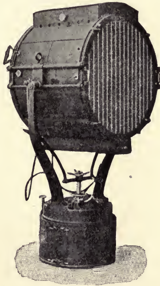
Fig. 120.—Search Light.
