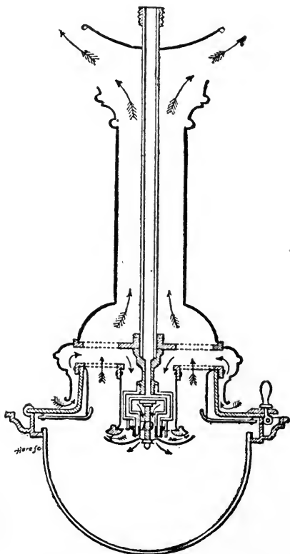
Fig. 22.—Siemens Regenerative Gas Burner.
