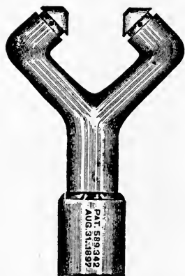
Fig. 23.—Acetylene Burner.
