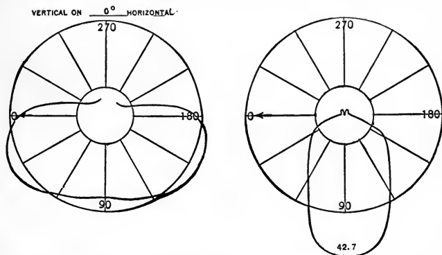
Figs. 67 and 68.—Curves of Distribution.
