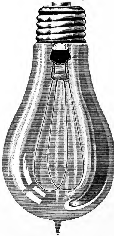
Fig. 29.—Lamp with Double Filament.
