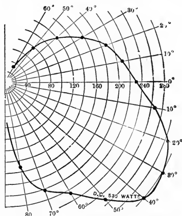
Fig. 50.—Distribution of Light from Enclosed Arc.
