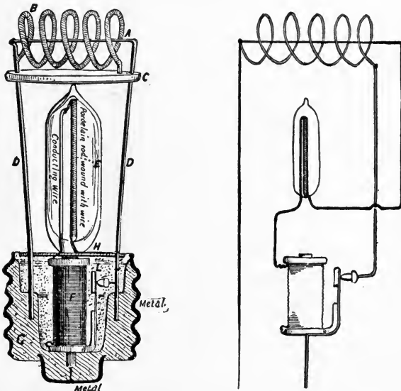
Fig. 39 and 40.—Connections of Nernst Lamp.
