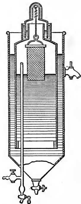
Fig. 24.—Small Acetylene Generator.
