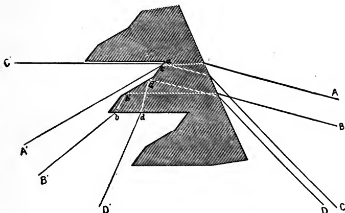
Fig. 72.—Section of Holophane Globe.
