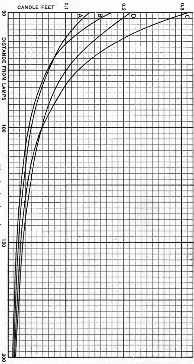
Fig. 99.—Illumination from Arcs.
