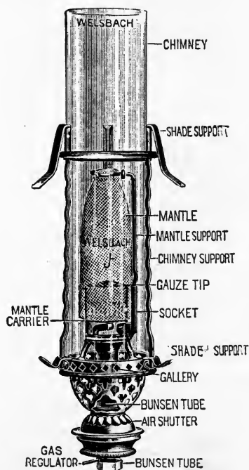
Fig. 26.—Standard Welsbach Burner.
