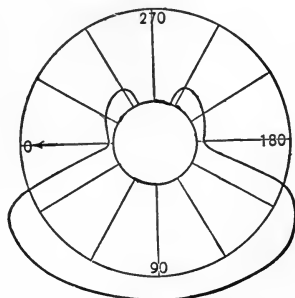
Fig. 64.—Distribution from Fluted Cone.
