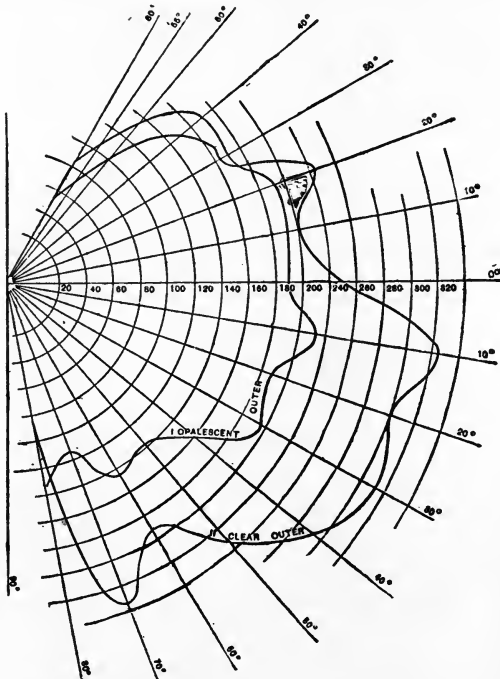
Fig. 51.—Effect of Globes on Enclosed Arc.
