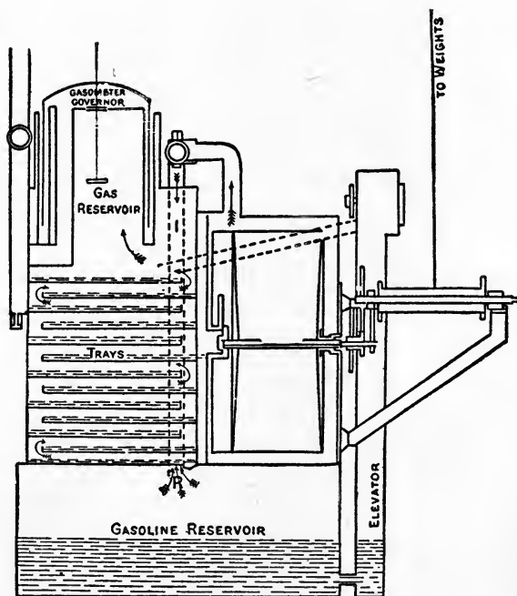
Fig. 19.—Gasoline Gas Machine.
