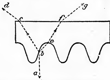
Fig. 73.—Diffusing Curves of Holophane.
