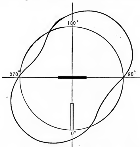
Fig. 30.—Distribution of Light from Flat Filament.
