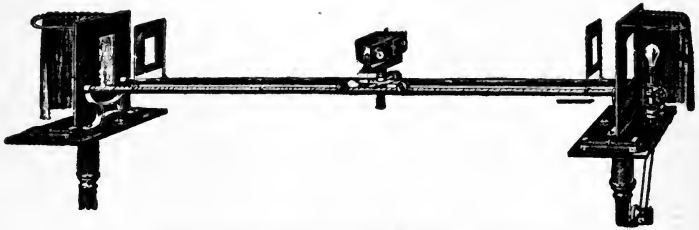
Fig. 123.—Photometer Bar Complete.
