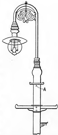
Fig. 106.—Boston Pole Fixture.
