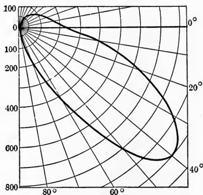
Fig. 49.—Distribution of Light from an Open Arc.
