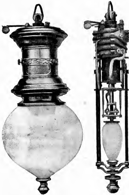
Fig. 48.—Typical Enclosed Arc Lamp.
