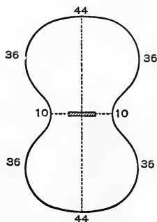
Fig. 44.—Horizontal Distribution from Nernst Lamp.
