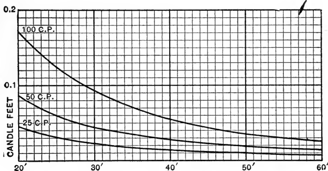
Fig. 102.—Illumination from Incandescent Lamps.
