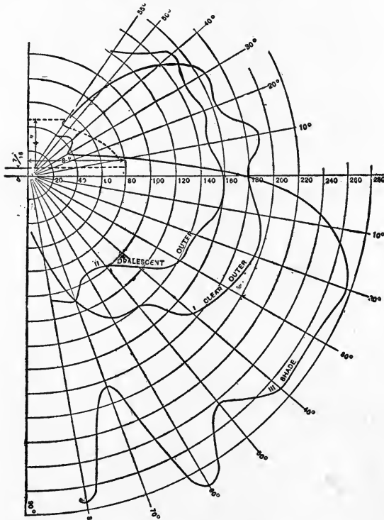
Fig. 52.—Distribution from Alternating Enclosed Arc.
