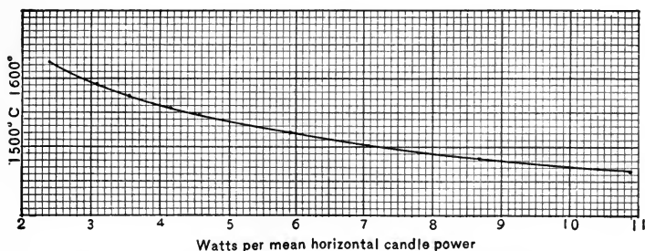
Fig. 35.—Variation of Efficiency with Temperature.
