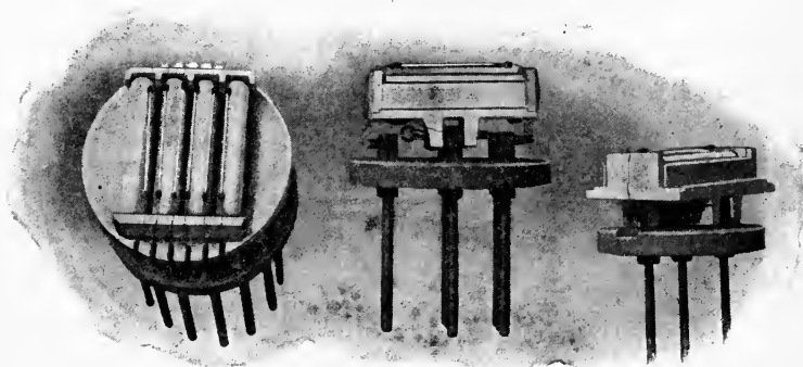
Fig. 42.—Glowers and Heaters of American Nernst Lamp.
