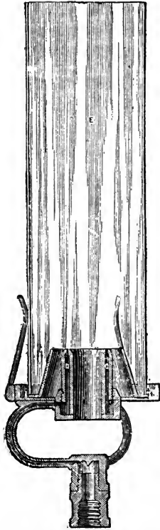
Fig. 20.—Section of Argand Gas Burner.
