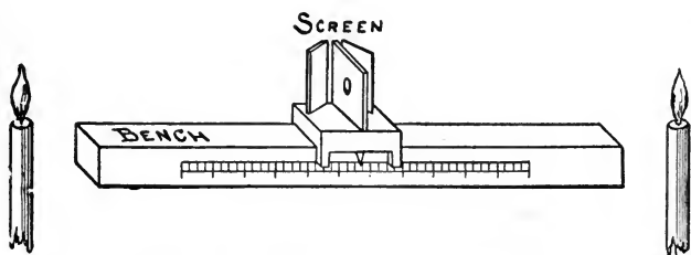
Fig. 122.—Bunsen Photometer.
