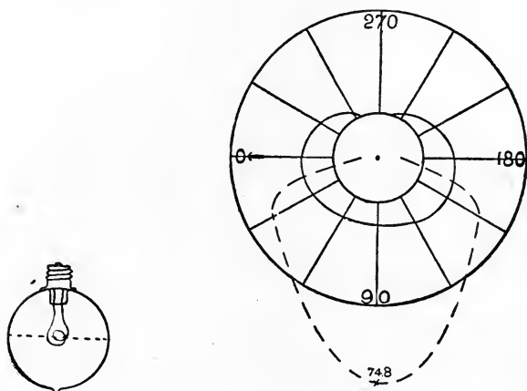
Figs. 69 and 70.—Reflector Lamp and Its Distribution.
