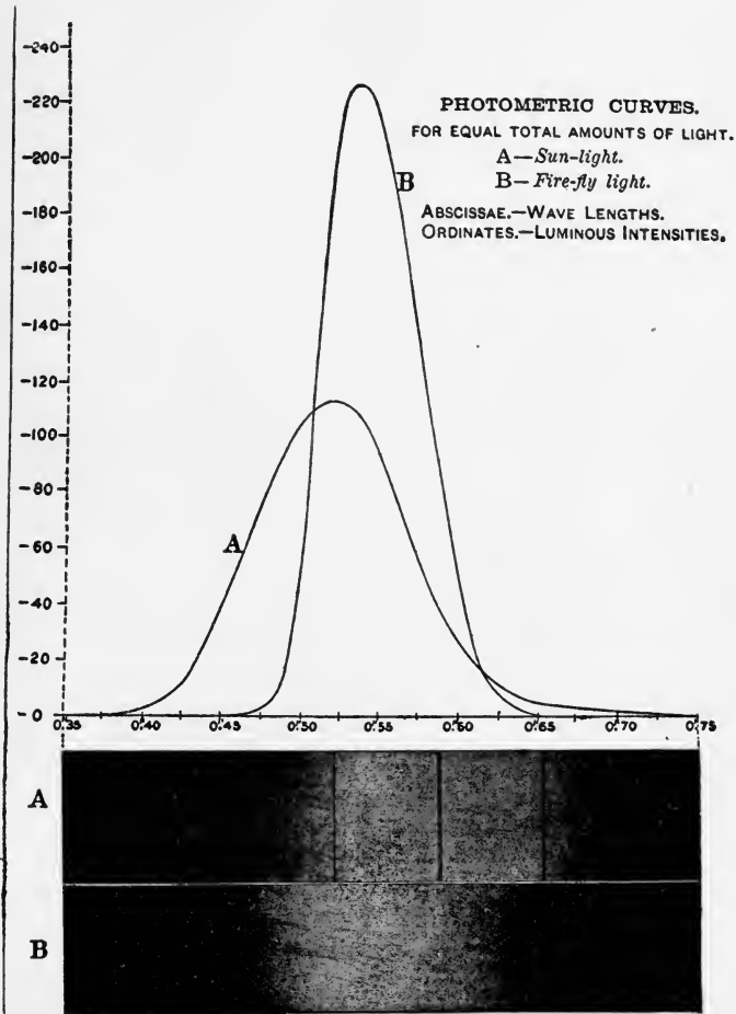
Fig. 45.—Curves of Firefly Light and Solar Light.
