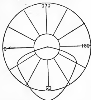
Fig. 63.—Distribution from Conical Shade.
