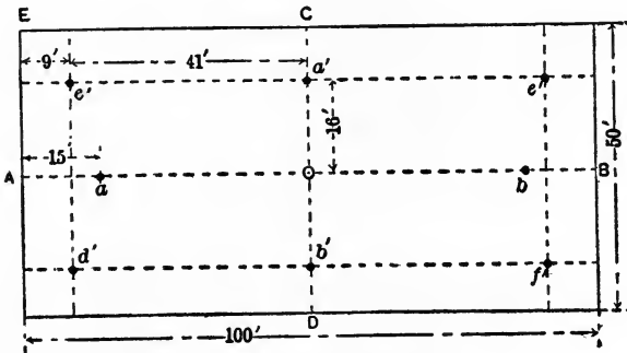
Fig. 89.—Plan of Hall.
