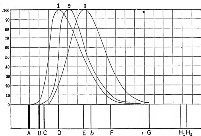
Fig. 9.--Effect of Faint Light on Color.
