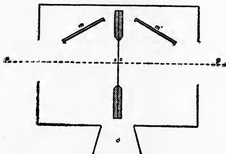
Fig. 121.—Bunsen Photometer Screen.
