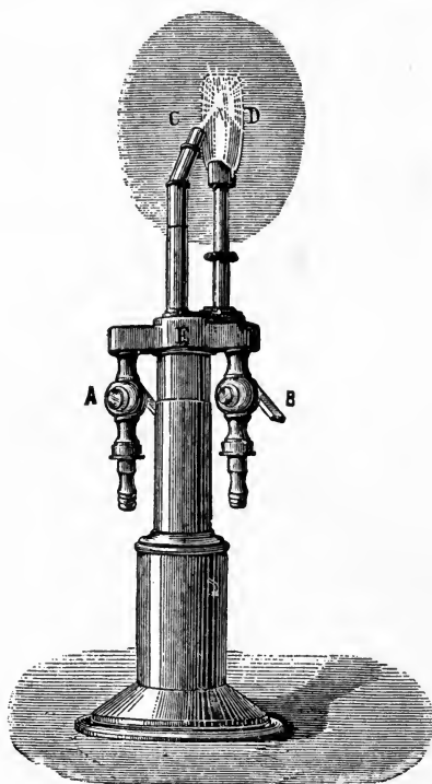
Fig. 25.—Oxy-hydrogen Burner.
