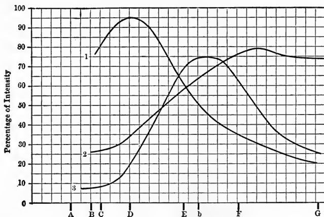
Fig. 12.—Selective Reflection.
