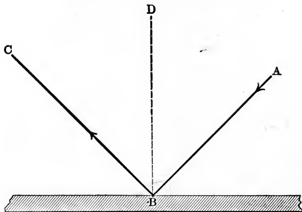
Fig. 10.—Regular Reflection.
