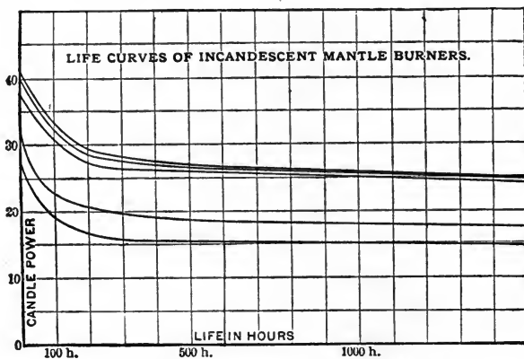
Fig. 27.—Life Curves, Welsbach Mantles.
