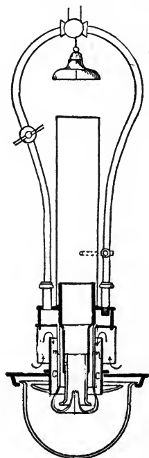
Fig. 21.—Wenham Regenerative Burner.
