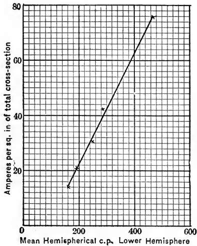
Fig. 47.—Relation between Current Density and Intensity.
