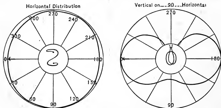
Figs. 31 and 32.—Distribution of Light from Looped Filament.
