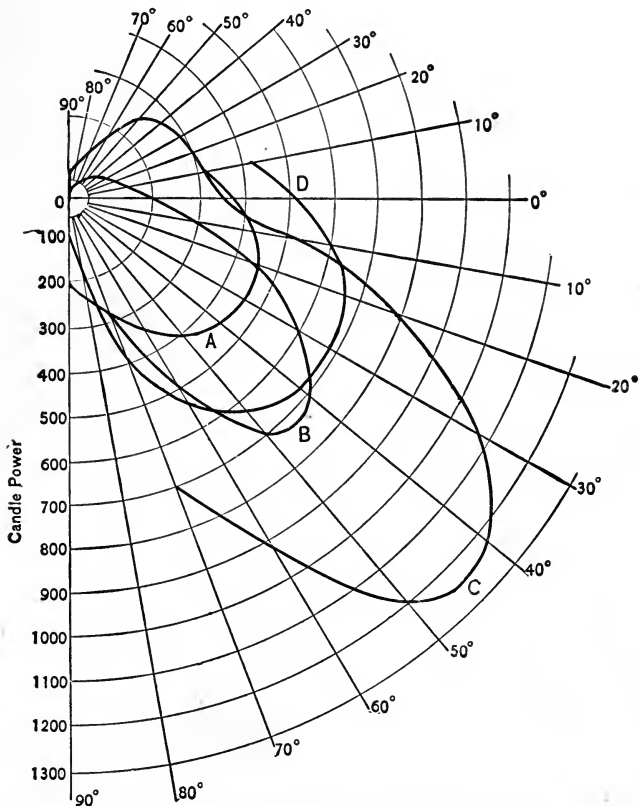
Fig. 97.—Distribution of Light from Arcs.
