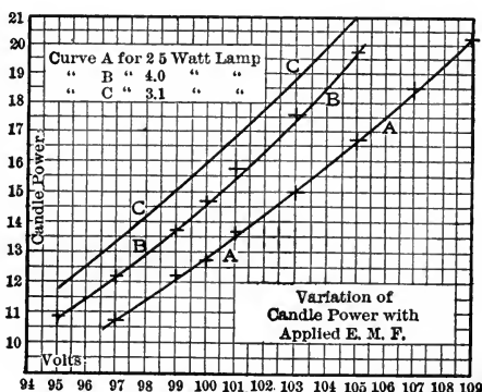
Fig. 125.—Variation of Light with Voltage.
