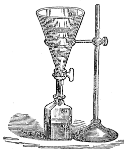
Tap funnel for separating ottoes from water and spirits from oil.
