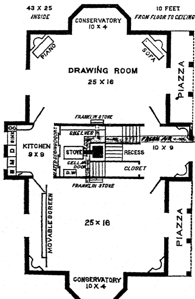
FIG. 12. VERNACULAR BUILDINGS IN CULTIVATED DRESS. Farm house planned by Lewis F. Allen, as rendered by Otis and Brown, architects, of Buffalo. As usual, the architects insisted upon fashionable decoration. The design, Allen remarked in his book, "is rather florid . . . but the cut and moulded trimmings may be left off by those who prefer a plain finish. Such, indeed, is our own taste" (from Allen's Rural Architecture , New York, 1852).
