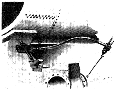
FIG. 27. FLEXIBLE POWER. The Stow flexible shaft (from The Masterpieces of the Centennial , Philadelphia, 1877).
