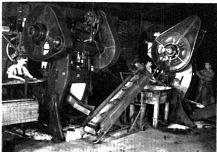
FIG. 28. FLEXIBLE FACTORY LAYOUT. Portable conveyor, electrically operated, receives stampings from chute of one punch press, carries them upward on cleated belt, and deposits them on tray by operator of next press, and so on through progressive operations (photograph of Press-Veyor installation at Dodge Tool and Manufacturing Company, courtesy of Rapids-Standard Co., Inc., Grand Rapids, Michigan).
