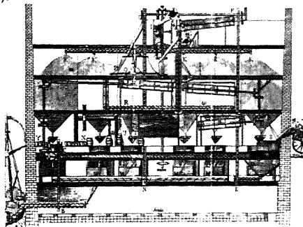
FIG. 6. OLIVER EVANS' AUTOMATIC CONVEYORS, 1785. A diagrammatic drawing of Thomas Ellicott's grain mill, near Baltimore, in which automatic machine production was achieved by the use of the conveyors, elevators, hopper-boys, and descenders invented by Oliver Evans (from Evans' The Young Mill-Wright and Miller's Guide , Philadelphia, 1795).
