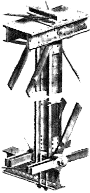
FIG. 8. DETAIL OF IRON BRIDGE CONSTRUCTION. The Point Bridge, Pittsburgh, built by the American Bridge Company, 1875 (from The Masterpieces of the Centennial International Exhibition, Philadelphia, 1877 ).
