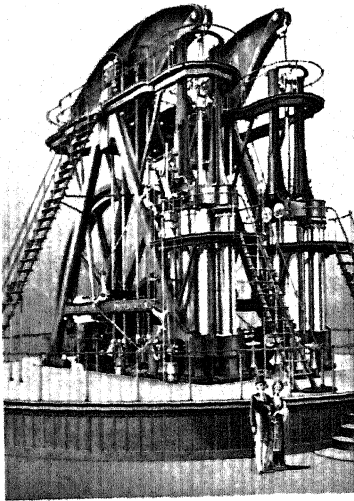
FIG. 3. THE CORLISS ENGINE AT THE CENTENNIAL EXHIBITION, 1876. This vast steam engine, designed without any concessions to contemporary notions of ornament and decoration, was the dominant feature of the exhibits in Machinery Hall. This picture, never before reproduced, is taken from a chromo-lithograph published in Treasures of Art, Industry and Manufacture Represented in the American Centennial Exhibition at Philadelphia, 1876 , Buffalo, New York, 1877.
