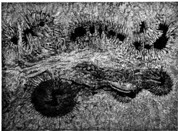
FIG. 40 —A Sun-spot.
