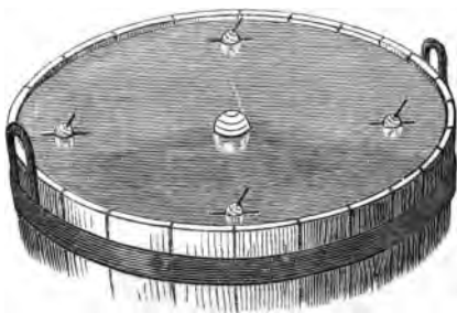
FIG. 15.—Earth with inclined axis of rotation.
