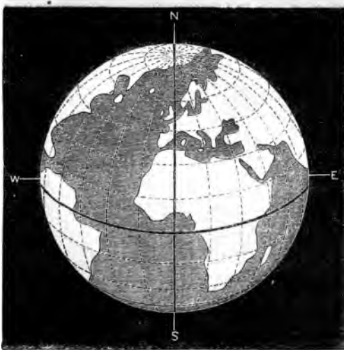
FIG. 16.—The Earth, as seen from the Sun at the Summer Solstice, June 22 (noon at London).
