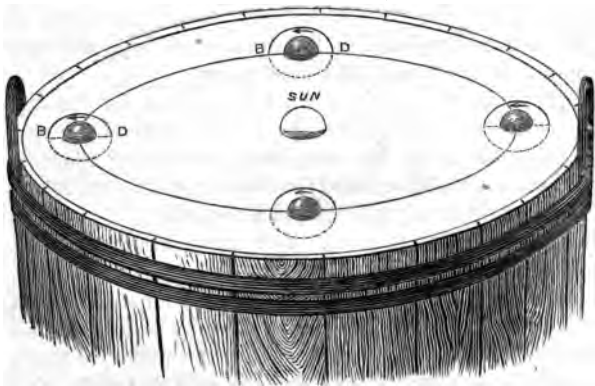
FIG. 26.—Shewing the inclination of the Moon's orbit to the plane of the ecliptic.
