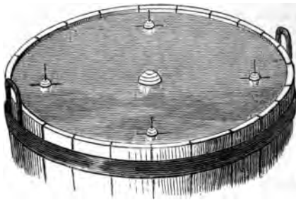
Fig. 12.—The plane of the Ecliptic.
