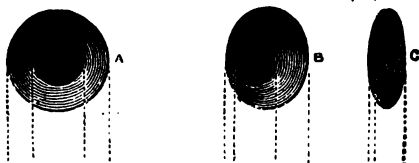
FIG. 41.—Explanation of the appearances presented by Sun-spots.
