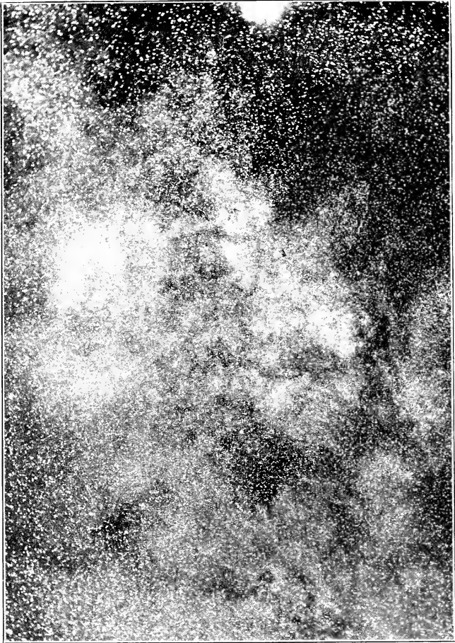
GREAT STAR CLOUD IN SAGITTARIUS
