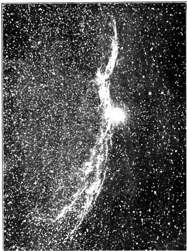
A PECULIAR NEBULAR FORMATION IN CYGNUS
