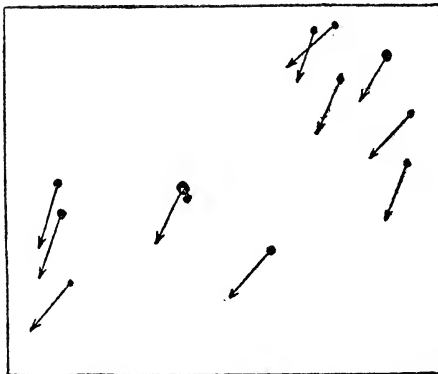
DIAGRAM OF THE PLEIADES
