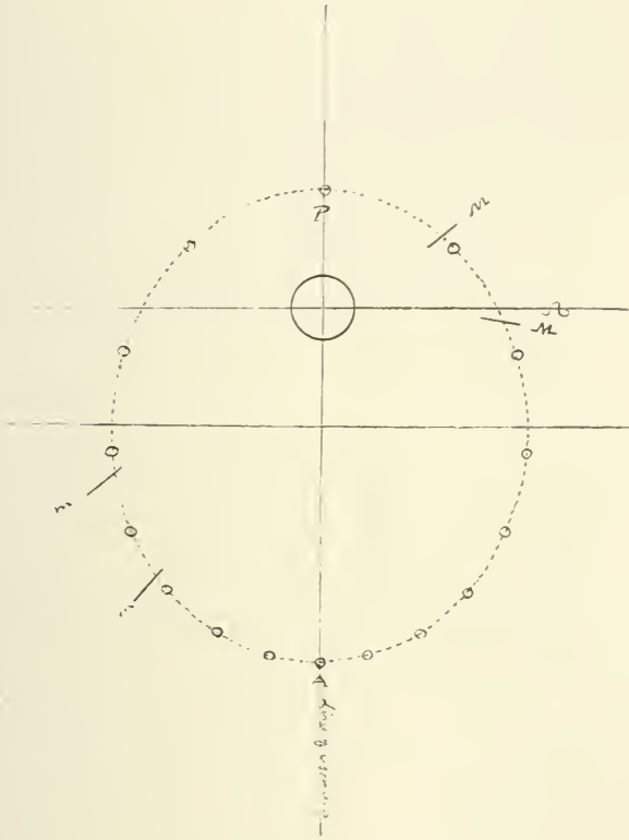
FIG. 1. Orbit of \delta Cephei. 1
