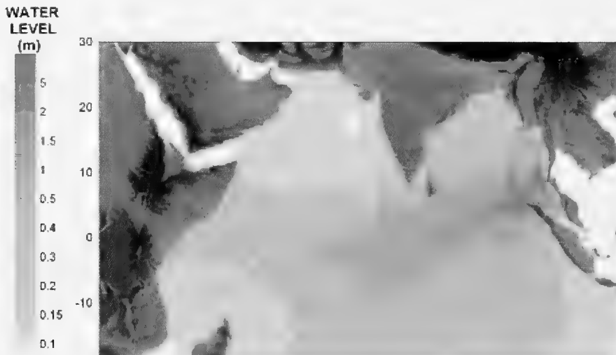
Figure 3. Computer modelling of the 26 December, 2004 tsunami after 900 minutes (courtesy of A. Yalciner, U. Kuran, T. Taymaz) (available at: http://yalciner.ce.metu.edu.tr/sumatra/max-elev-sim-1.jpg ).
