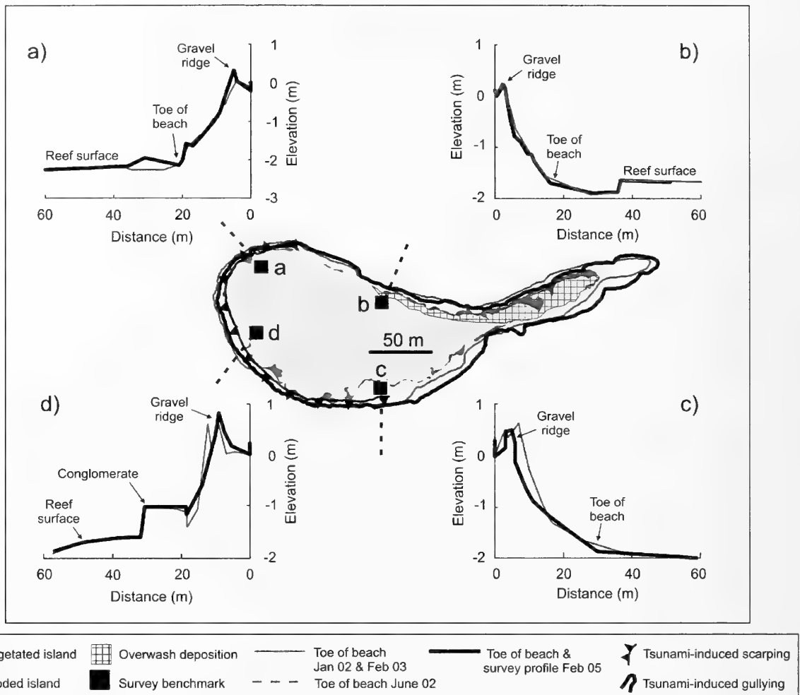
Figure 15. Pre- and post-tsunami plan and profile changes on Gaaviligili Island. Location of island shown in Figure 2.
