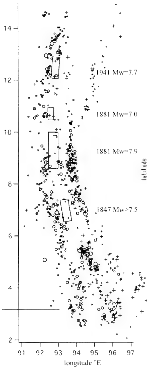
Figure 3. Large historical earthquakes between 2 and 14°N. Open circles are aftershocks to 14 January 2005 following the 26 December 2004 earthquake and crosses are seismic events (mostly \geq M = 5.5 ) 1964-2004) (after Bilham et al., 2005).
