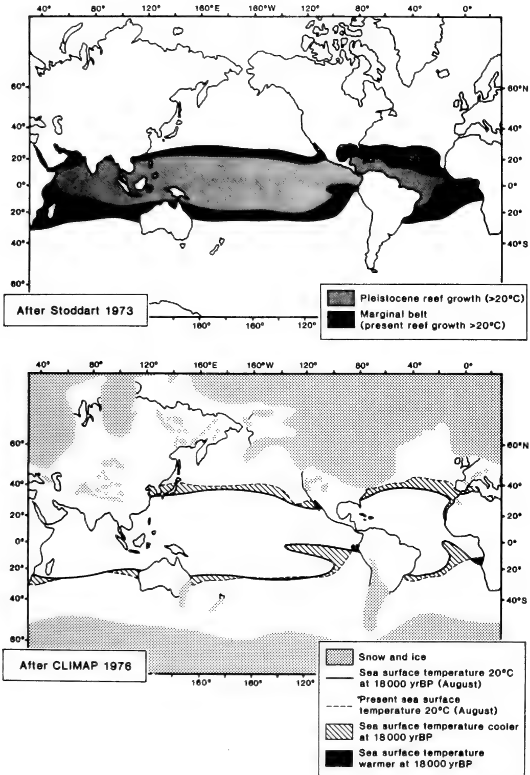
Figure 12. Possible changes in the extent of the reef seas, 18 \times 10^3 yr B.P. v. present. In each case the isotherm of 20^{\circ}\text{C} is taken as the effective limit of reef formation (Stoddart 1973. CLIMAP Project Members 1976).
