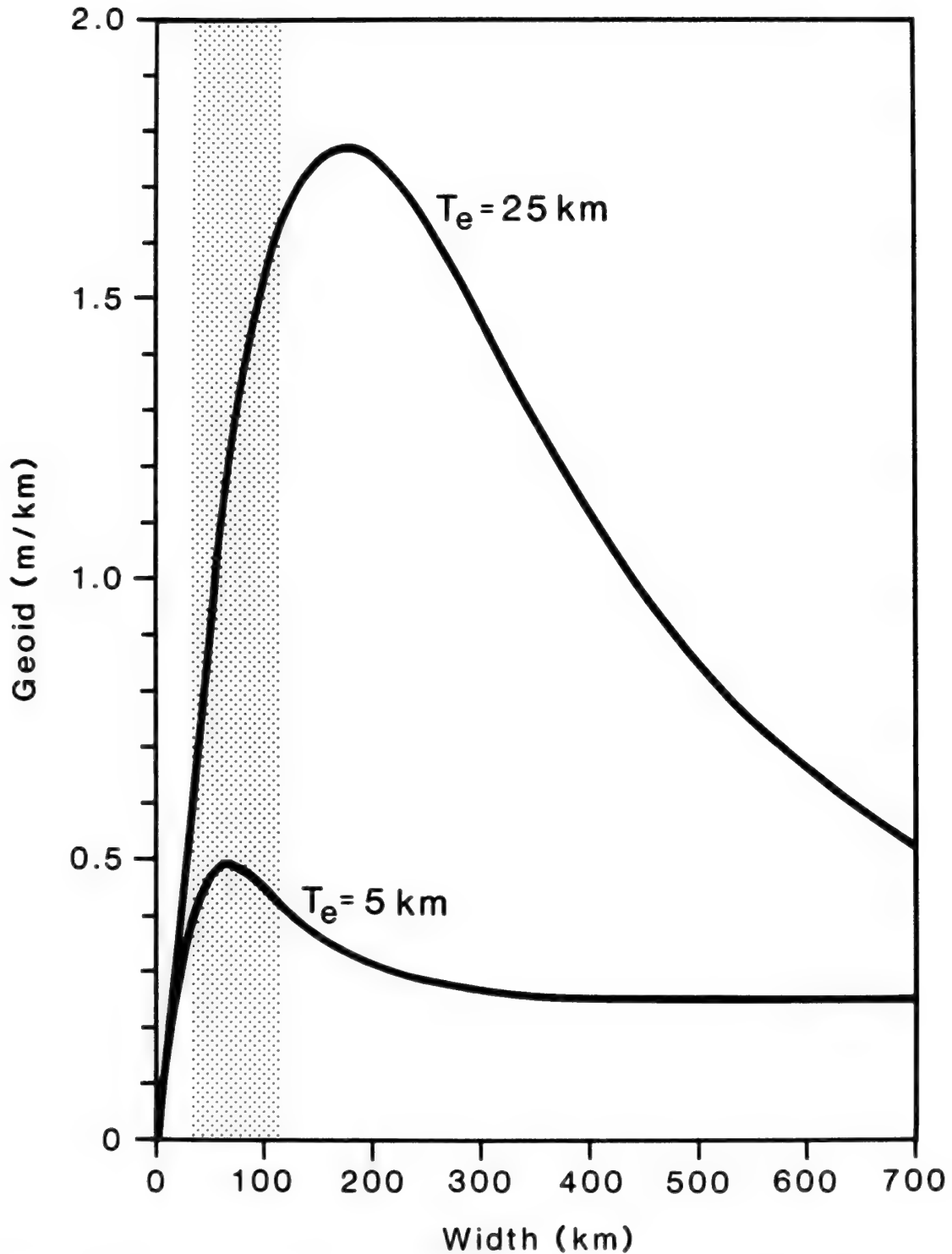
Figure 5. Maximum amplitude of geoid anomaly associated with two-dimensional seamount model. Upper curve for emplacement off-ridge ( T_e = 25 \text{ km} ), lower curve for on-ridge origin ( T_e = 5 \text{ km} ). Abscissa represents e^{-1} width of Gaussian seamount topography and vertical band indicates range of widths for typical oceanic seamount. Ordinate shows maximum geoid anomaly amplitude over feature 1 km high (after Watts and Ribe 1984).
