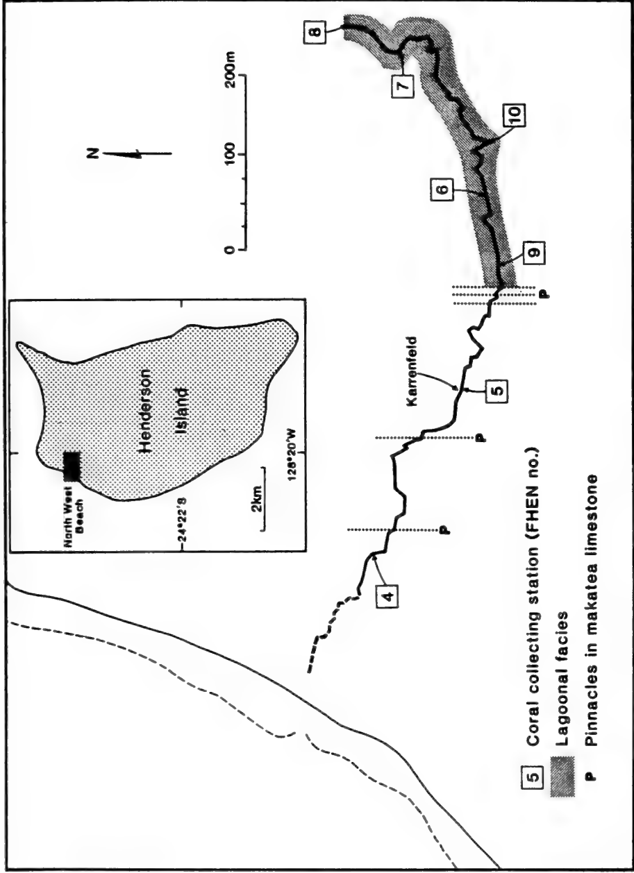
Figure 15. Plan of island cliff margin to island interior transect, North-west beach.
