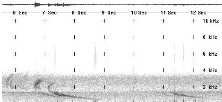
Spectrogram of nose whistlers accompanied by hissband recorded in northern Alberta 02 June 1996 at approximately 1430 UT - S. McGreevy
