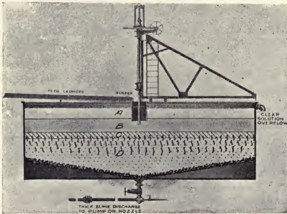
FIG. 103.—Dorr Thickener, Showing Slime-settling Zones.
