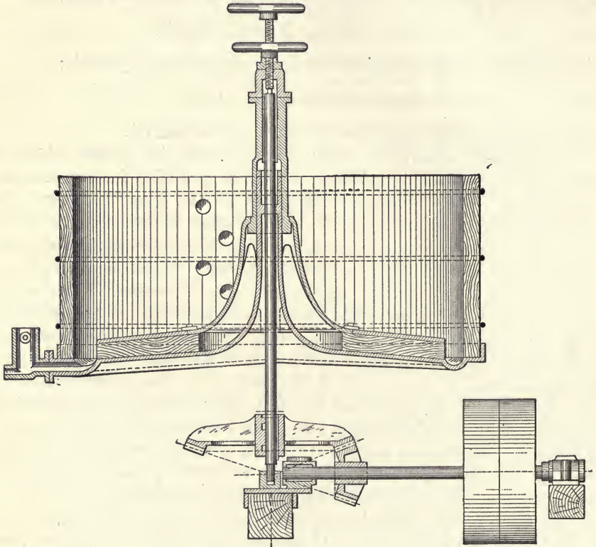
FIG. 136.—Eight-foot Settler.
