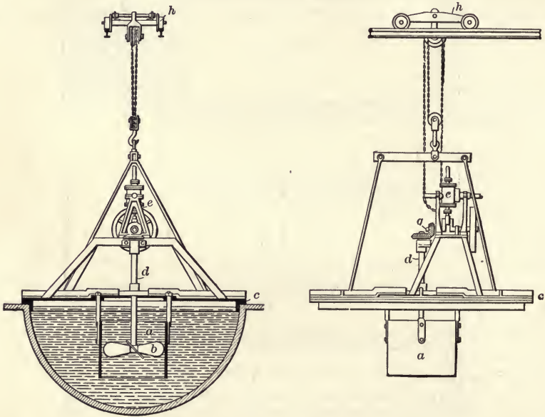
FIG. 272.—Howard Mixer.
