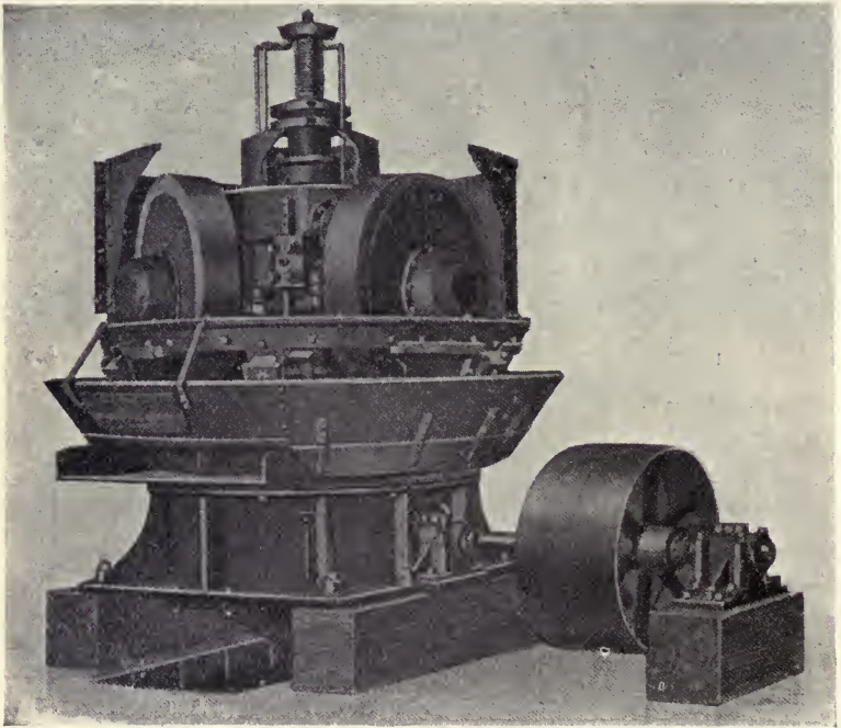
FIG. 46.—Chilian Mill.
