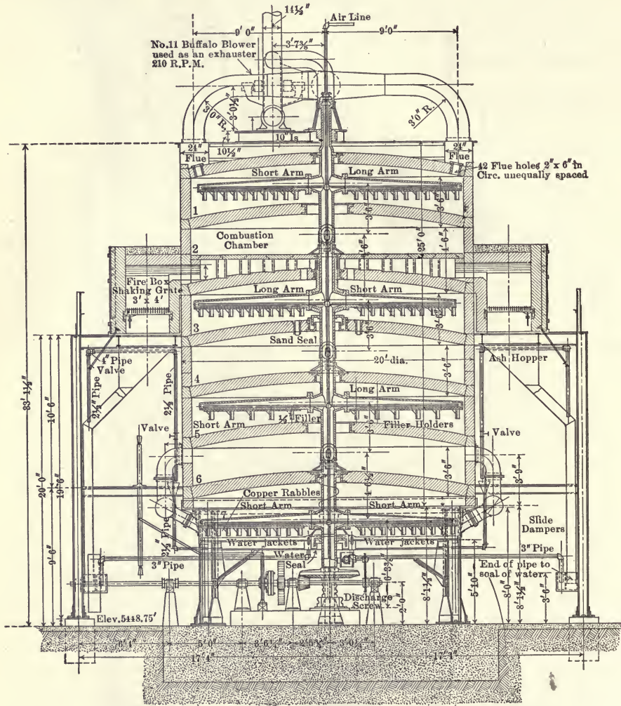
FIG. 236.—Sectional Elevation of Roasting Furnace.
