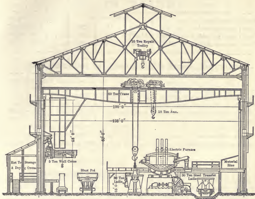
FIG. 189.—Electric-furnace Building.
