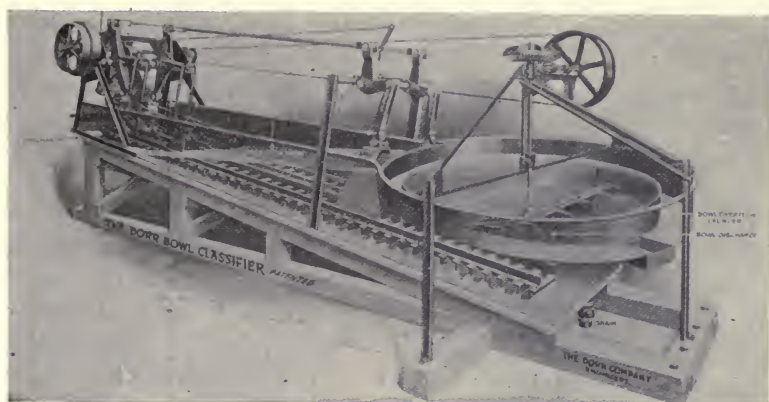
FIG. 61.—The Dorr Bowl-classifier.
