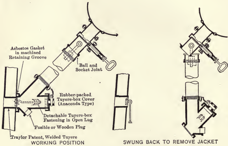
FIG. 259.—Blast-furnace Tuyere.
