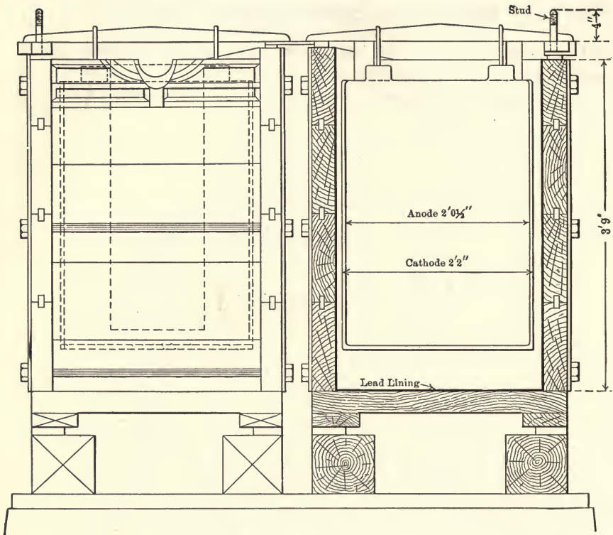
FIG. 247.—Electrolytic Tank.
