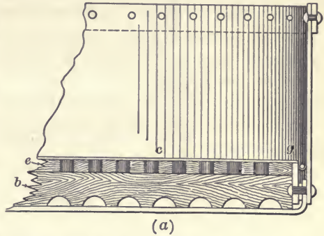
FIG. 98.—Section of Steel Leaching Tank.
