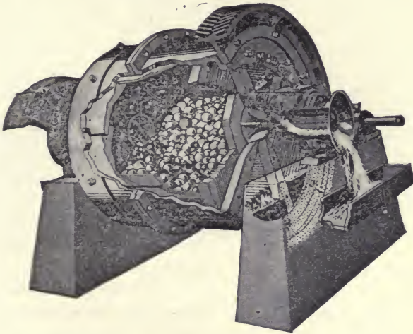
FIG. 39.—Marcy Ball-mill (perspective view).
