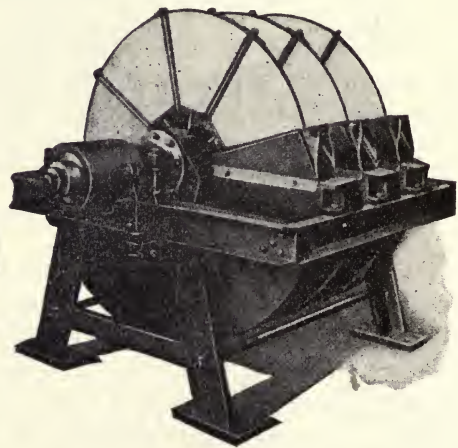
FIG. 109.—The American Filter.
