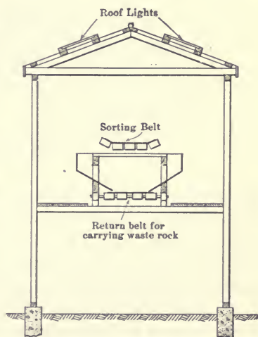
FIG. 121.—Sorting Belt.
