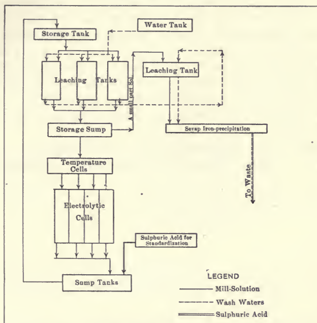
FIG. 237.—Solution Flow-sheet, Butte-Duluth Mill.
