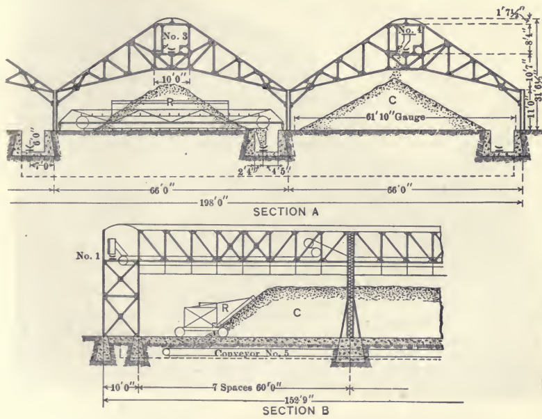
FIG. 193.—Messiter Bedding System.
