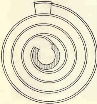
FIG. 326.—Section of Frenier Pump.
