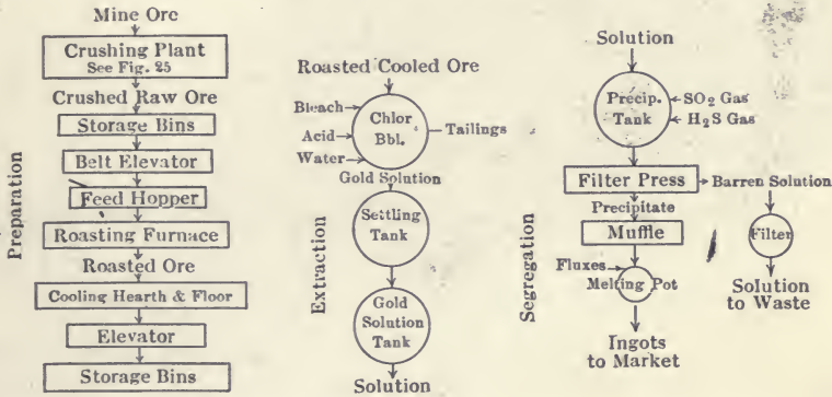
FIG. 92.—Flow-sheet of Barrel Chlorination.
