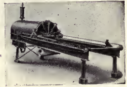
FIG. 112.—Single Kelly Filter Press.
