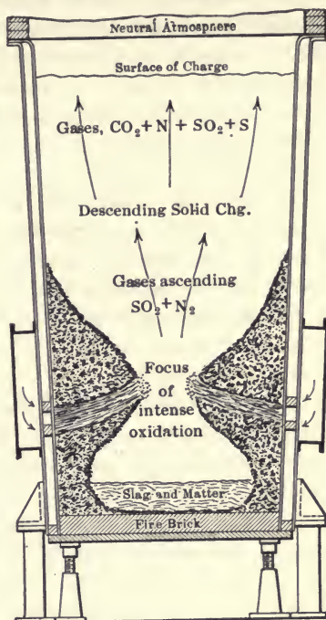
FIG. 209.—Section of Furnace in Pyritic Smelting.
