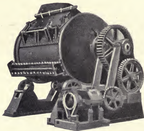
FIG. 217.—Horizontal Type of Converter.
