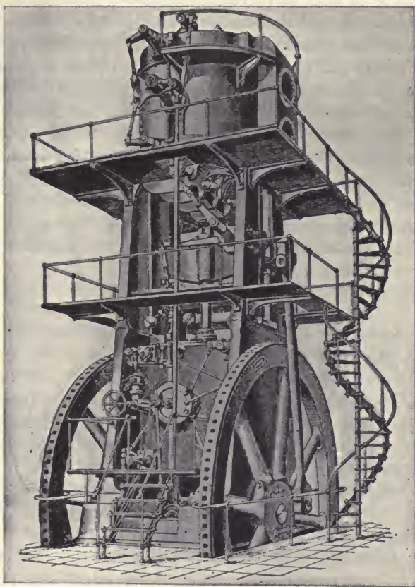
FIG. 160.—Blowing-engine.
