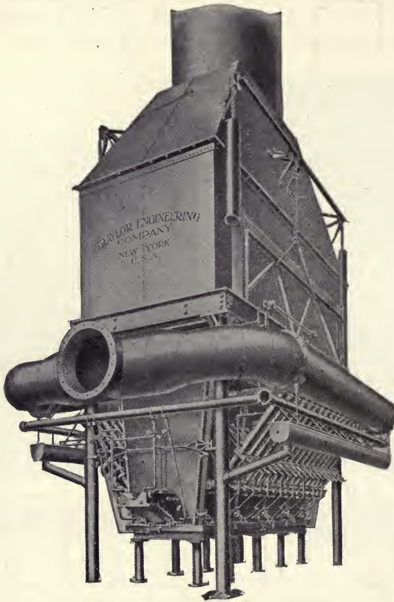
Fig. 196.—View of Copper Blast-Furnace.
