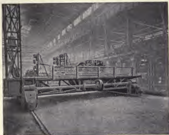
FIG. 181.—Charging Machine.
