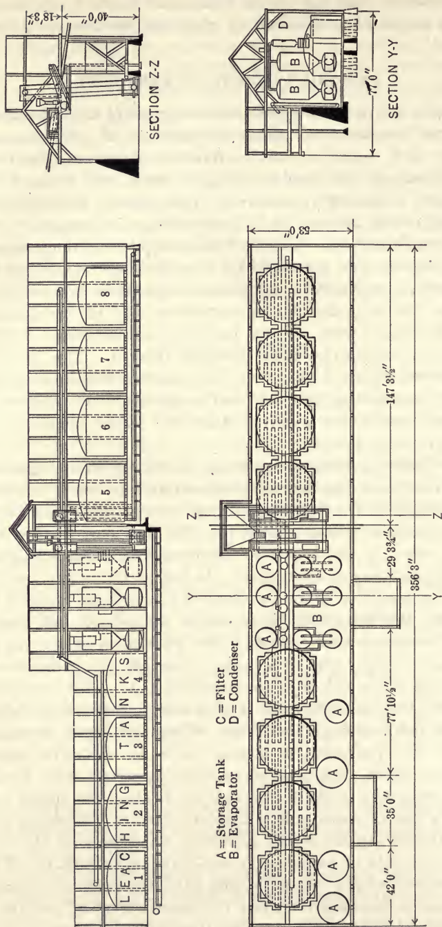
Fig. 240.—Ammonia Leaching Plant at Kennecott, Alaska.
