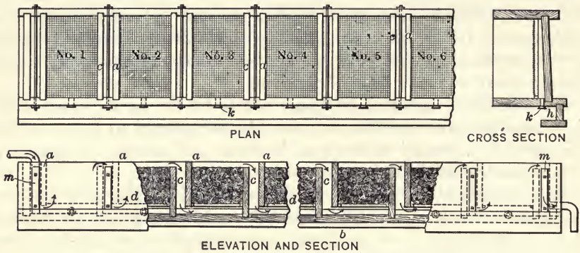
FIG. 118.—Seven-compartment Zinc-box.
