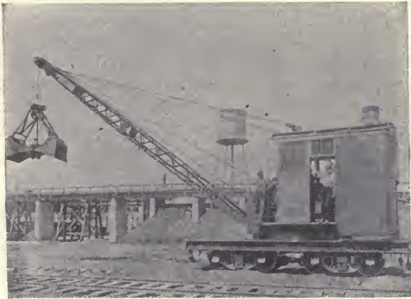
FIG. 306.—Track-crane and Grab-bucket.
