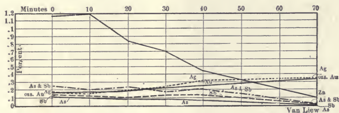
FIG. 131.—Elimination of Impurities in Converting.
