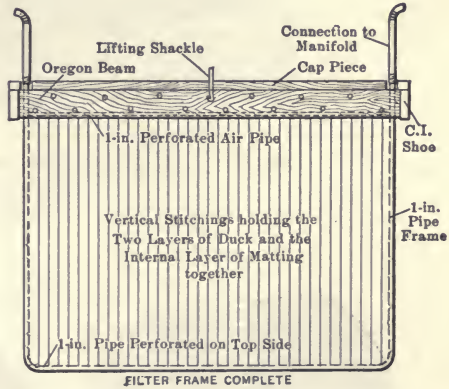
FIG. 106.—Butter's Filter-frame.
