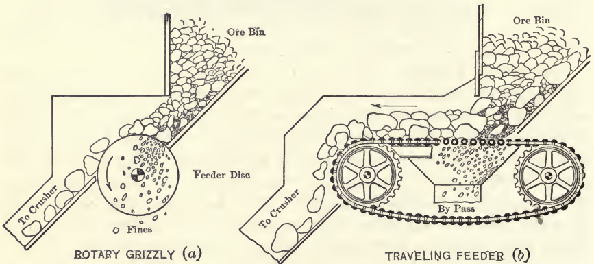
FIG. 320.—Moving Feeders.
