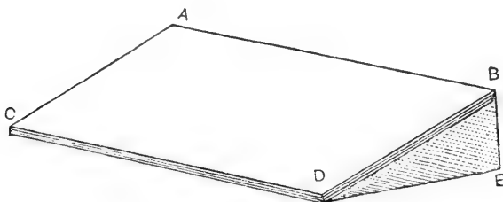
A B or C D, 16 in. ; A C or B D, 10 in. ; B E, 3 in.
