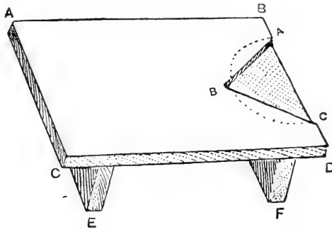
Bottom Board No. 1 for an 8-framed hive, A B or C D 2 feet, or 2\frac{1}{2} in. longer than the full width of the hive. A B or B D 14\frac{1}{2} in., or the full width of the hive. E F the legs, 16 in., or the length of the width of the board, and 3 in. wide. A B C, the points of the V entrance.
