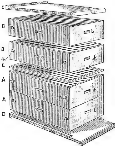
The Heddon Hive.—A, Bodies used as brood-chamber; B, Bodies used as super; c, Cover; D, Bottom board; Slatted wood and zinc honey-board (Queen excluding); a, Wood thumb-screws; b, Handholes for lifting.
