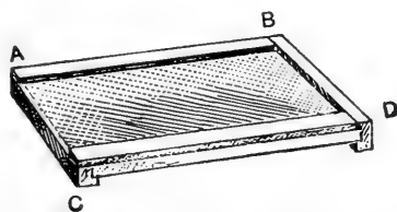
Bottom board No. 2 for an 8-frame hive. A B or C D 2 ft., or 2\frac{1}{2} in. longer than the full width of the hive. A C or B D 14\frac{1}{2} in., or the full width of the hive.
