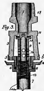
GRAY. (Section.)
