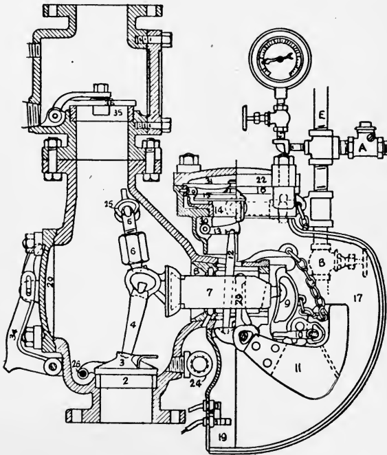
NIAGARA DRY VALVE NO. 3. (Section.)
