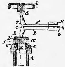
MANUFACTURERS. (Section.)
