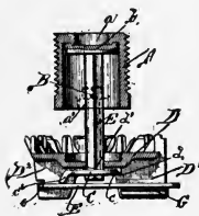
MACKEY 4. (Section.)
