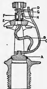
PHENIX. (Section.)
