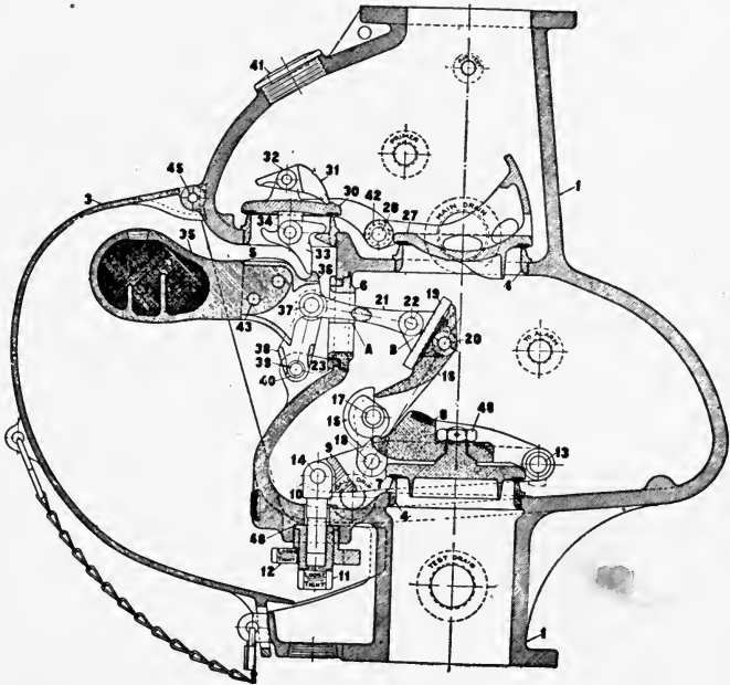
EVANS DRY VALVE. (Section.)
