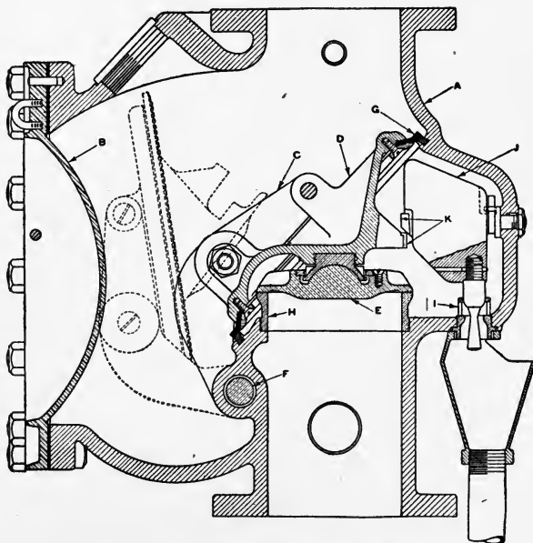
GRINNELL DRY VALVE MODEL C. (Section.)
