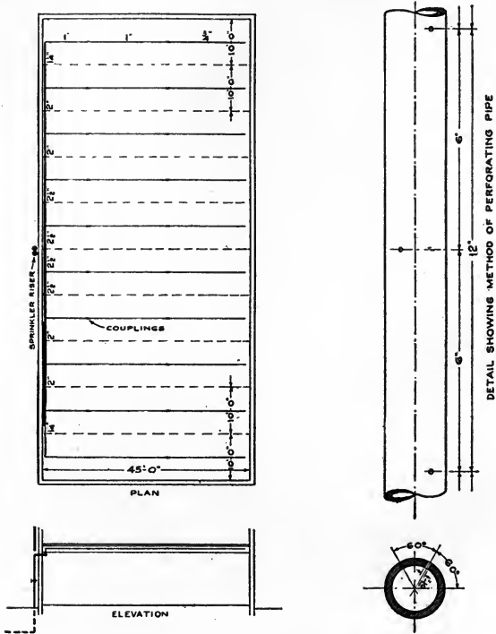
FRANCIS SYSTEM
