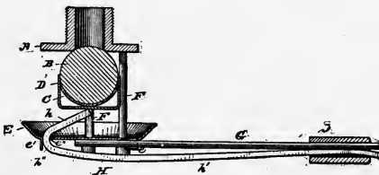
RUTHENBURG. (Section.)
