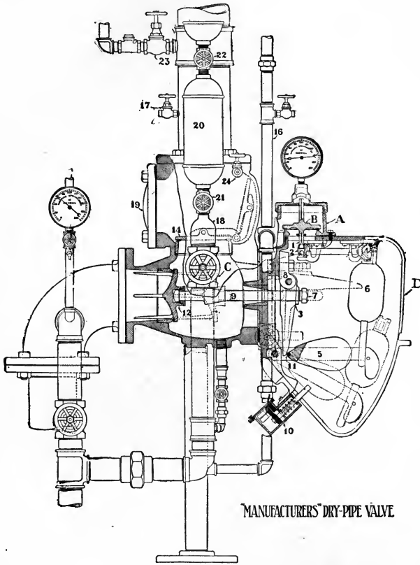
MANUFACTURERS DRY-PIPE VALVE 3. (Section.)
