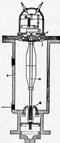
GARRETT RETARDING CHAMBER. (Section.)
