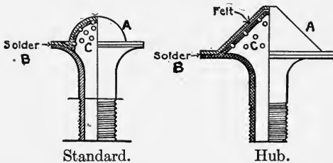
WHITING SPRINKLER.
