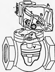
NEU ALARM VALVE.
