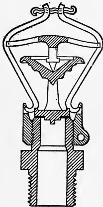
HIBBARD 1. (Section.)
