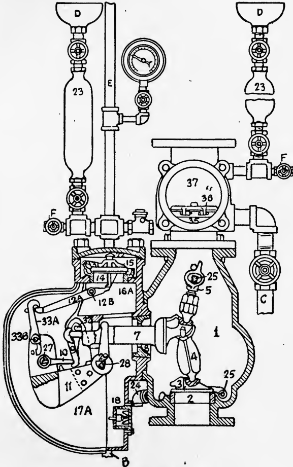
NIAGARA DRY VALVE No. 6 (Section)
