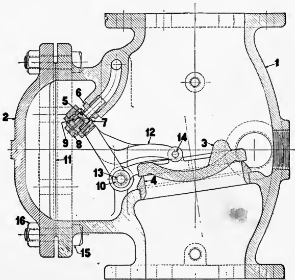
GLOBE ALARM VALVE (Model E).
