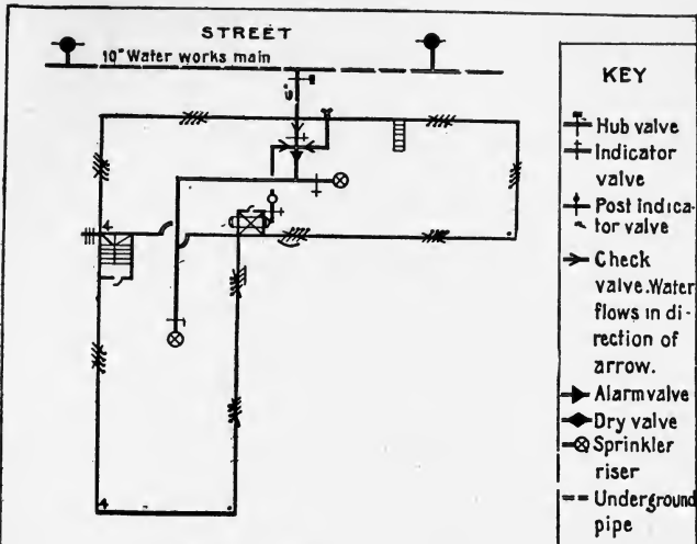
PIPE SCHEME 1 City Plant with water works pressure tank and steamer connection.
