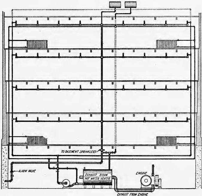
COMBINED HEATING AND SPRINKLER SYSTEM. (Sectional view showing arrangement of piping.)
