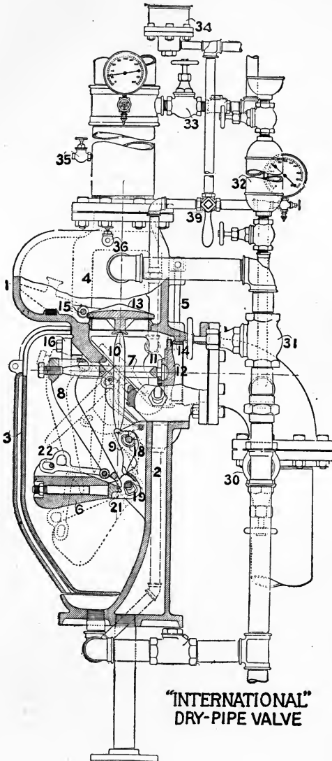
INTERNATIONAL DRY-PIPE VALVE 4. (Section.)
