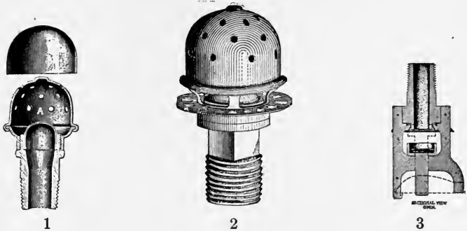
BURRITT SPRINKLERS.
