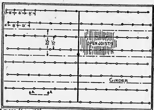
METHOD OF SPACING SPRINKLER HEADS UNDER OPEN JOIST CEILINGS IN BUILDINGS OF ORDINARY CONSTRUCTION SPRINKLERS STAGGERED
