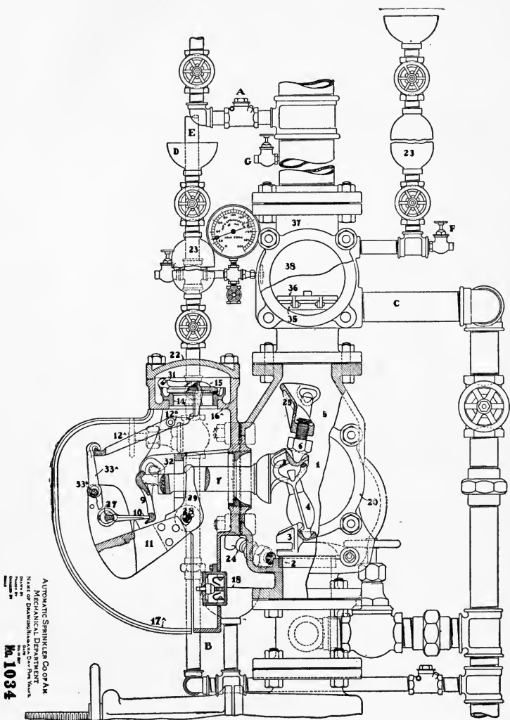
NIAGARA DRY VALVE MODEL 8 OR G. (Section.)
