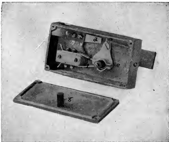
A. D. T. GATE VALVE ATTACHMENT. INTERIOR.
