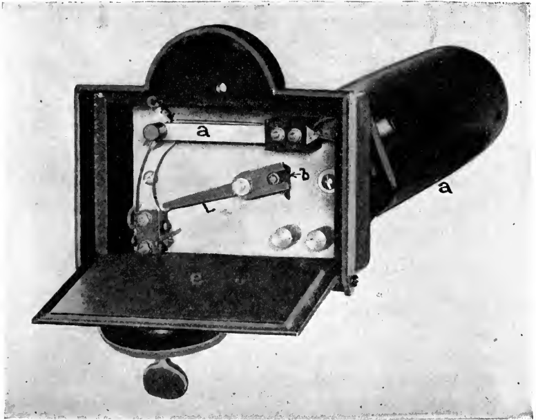
A. D. T. WATER LEVEL DEVICE. 1906 TYPE. No longer used. a , case. b , lever attached to float. c , contact point. d , case contact springs. e , case cover. L , lever operated by float.
