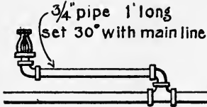
STRAIGHT OFFSET.
