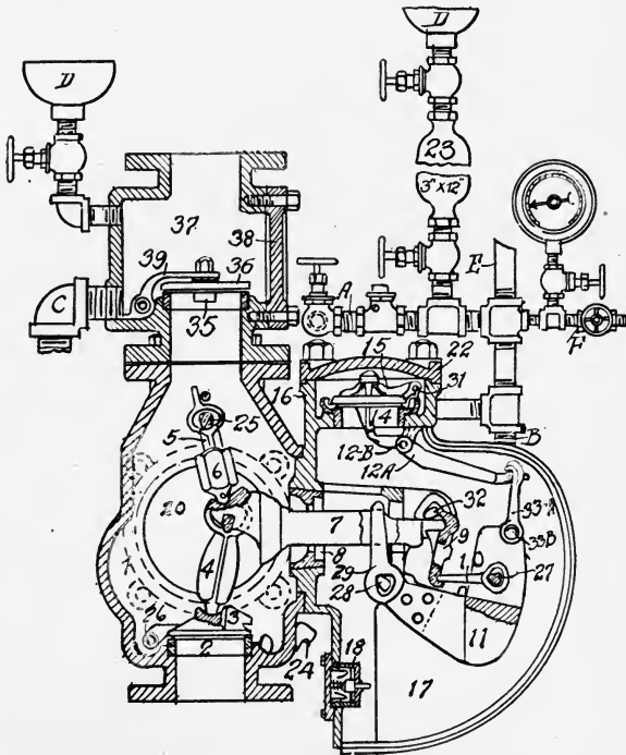
NIAGARA DRY VALVE No. 5 (Section).
