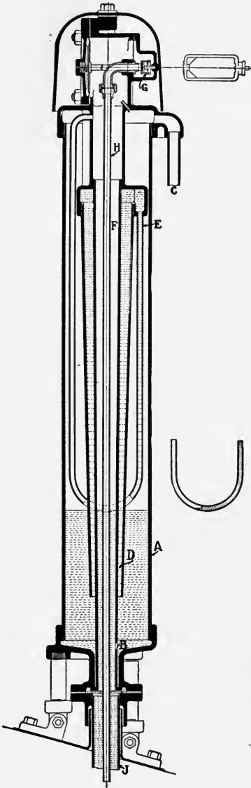
EXPANSION CHAMBER. (Sectional View.)
