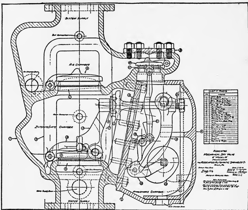
ASSOCIATED DRY VALVE (Section).
