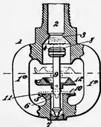
HILL. (Open.) (Section.)
