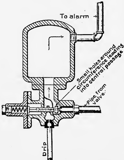
ASSOCIATED ALARM VALVE RETARDING CHAMBER. (Section.)
