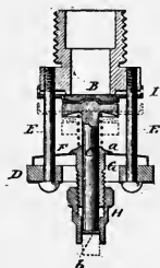
BISHOP 2 \frac{1}{4} . (Section.)
