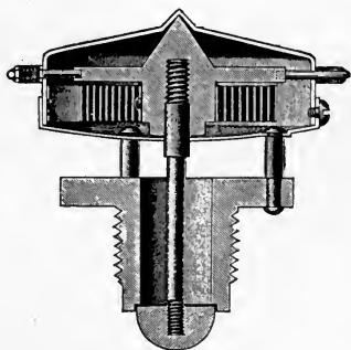
NAGLE. (Section.)
