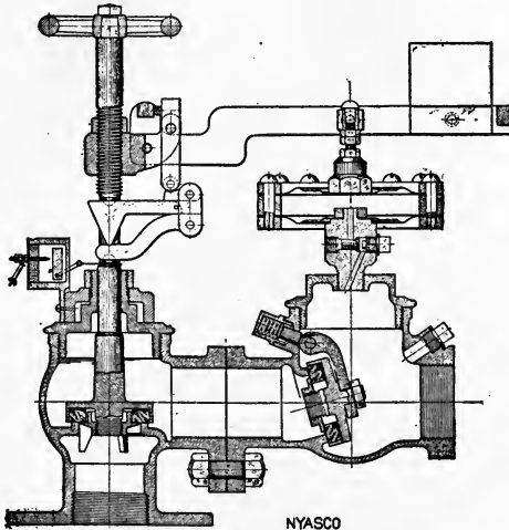
NYASCO DRY VALVE. (Section.)
