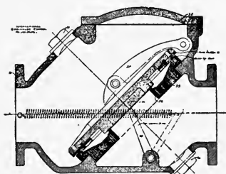
INTERNATIONAL DIFFERENTIAL DRY VALVE. (Section.)
