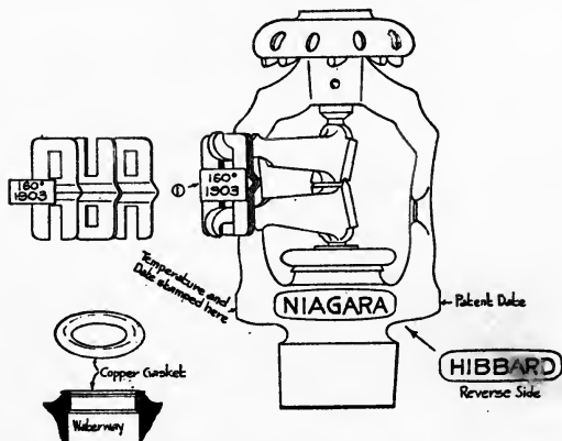
NIAGARA-HIBBARD A 2 -1903.
