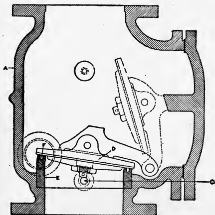
GARRETT ALARM VALVE. (Section.)
