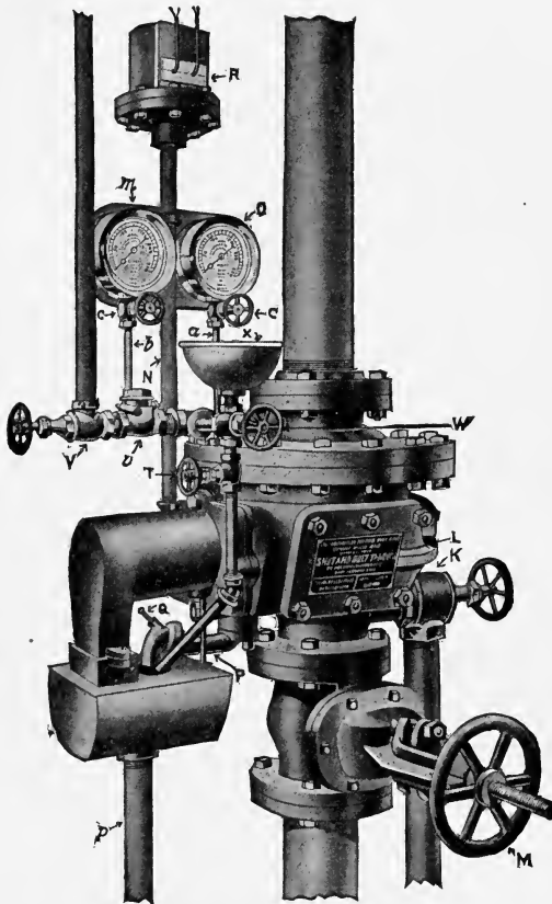
GRINNELL DRY VALVE. Straightway Type. General view showing fittings.
