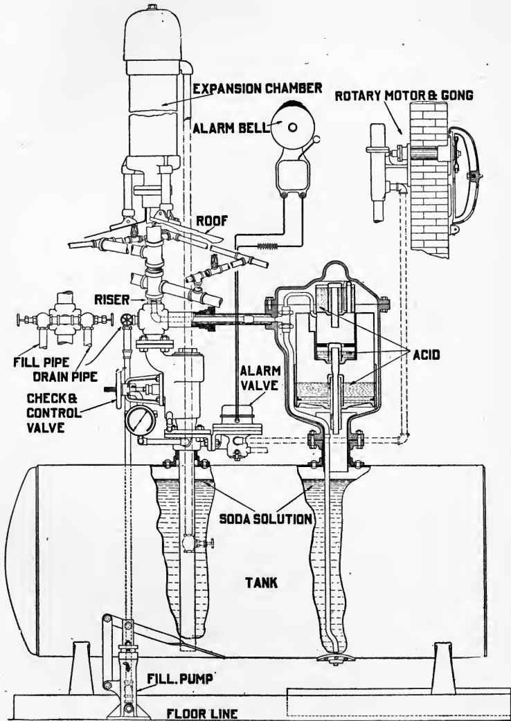
GENERAL VIEW OF SYPHO CHEMICAL SPRINKLER SYSTEM. (Condensed and not to scale.)
