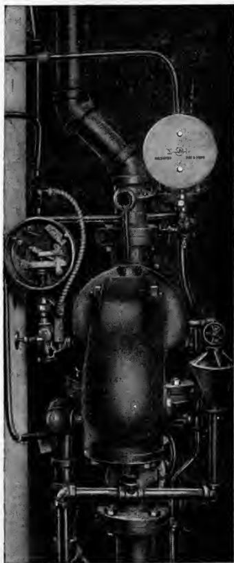
A. D. T. DRY VALVE ATTACHMENT.
