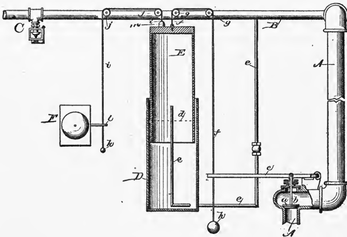
WALWORTH DRY VALVE 1. (Section.)
