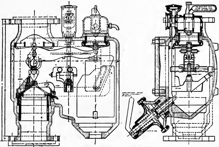
GENERAL DRAWING 3" PHENIX MECHANICAL DRY VALVE PHENIX FIRE EXTINGUISHER CO. 1838-39-40 FIRST NATIONAL BANK BLDG. CHICAGO ILL.
