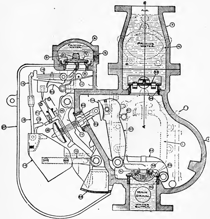
GLOBE DRY VALVE "B." (Section.)
