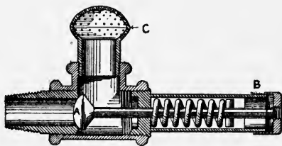
BROWN AND FOSKETT SPRINKLER. A, valve disc. B, releasing device. C, distributor.
