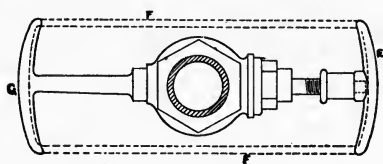
Top View CONANT SPRINKLER.
