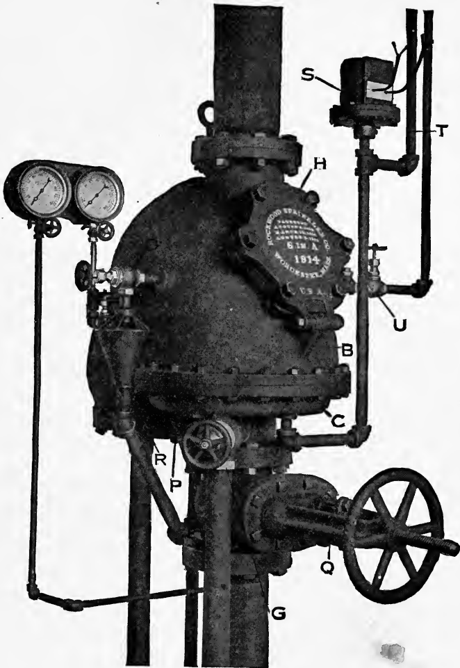
ROCKWOOD DRY VALVE A. (General view.)
