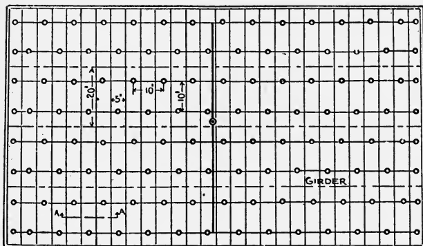
METHOD OF SPACING SPRINKLER HEADS UNDER CEILINGS OF SLOW-BURNING AND FIREPROOF CONSTRUCTION BAYS 5 FT X 20 FT SPRINKLERS STAGGERED IN ALTERNATE BAYS.
