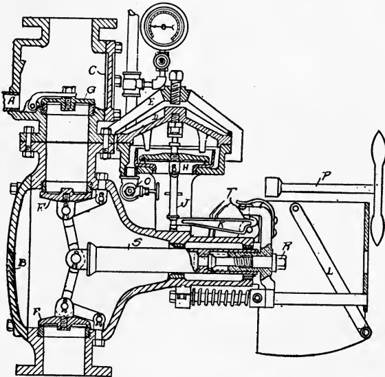
NIAGARA DRY VALVE NO. 2. (Section.)
