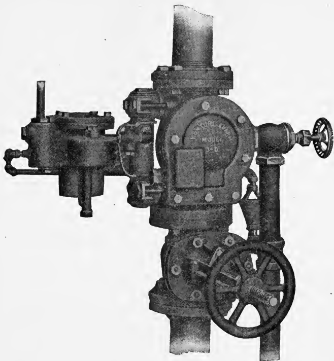
VENTURI ALARM VALVE 3D.
