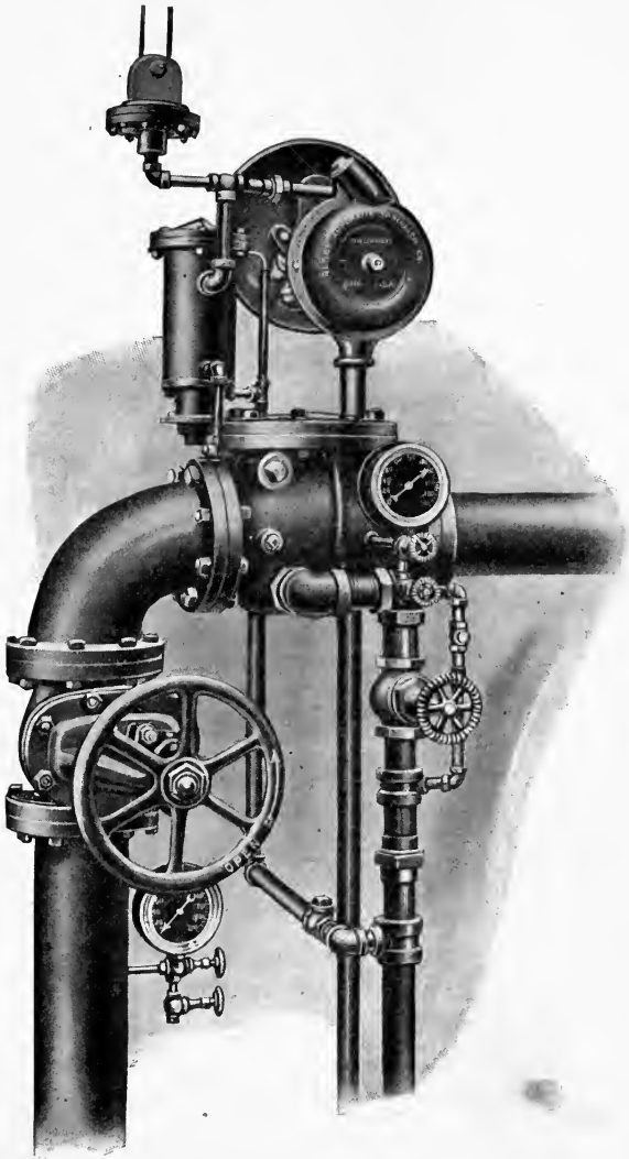
GARRETT ALARM VALVE.
