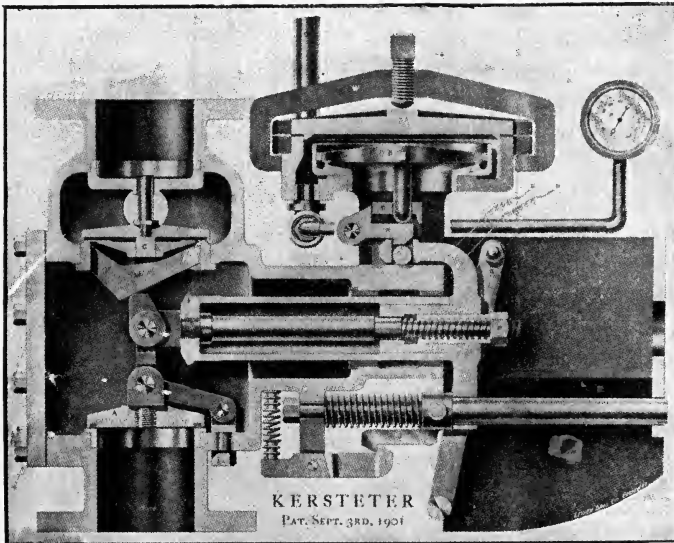
KERSTETER DRY VALVE 2. (Section.)
