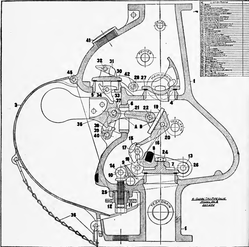
GLOBE DRY VALVE MODEL 5.
