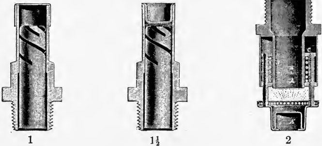
BISHOP SPRINKLERS. (Section.)
