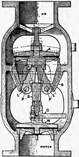
CATARACT DRY VALVE.
