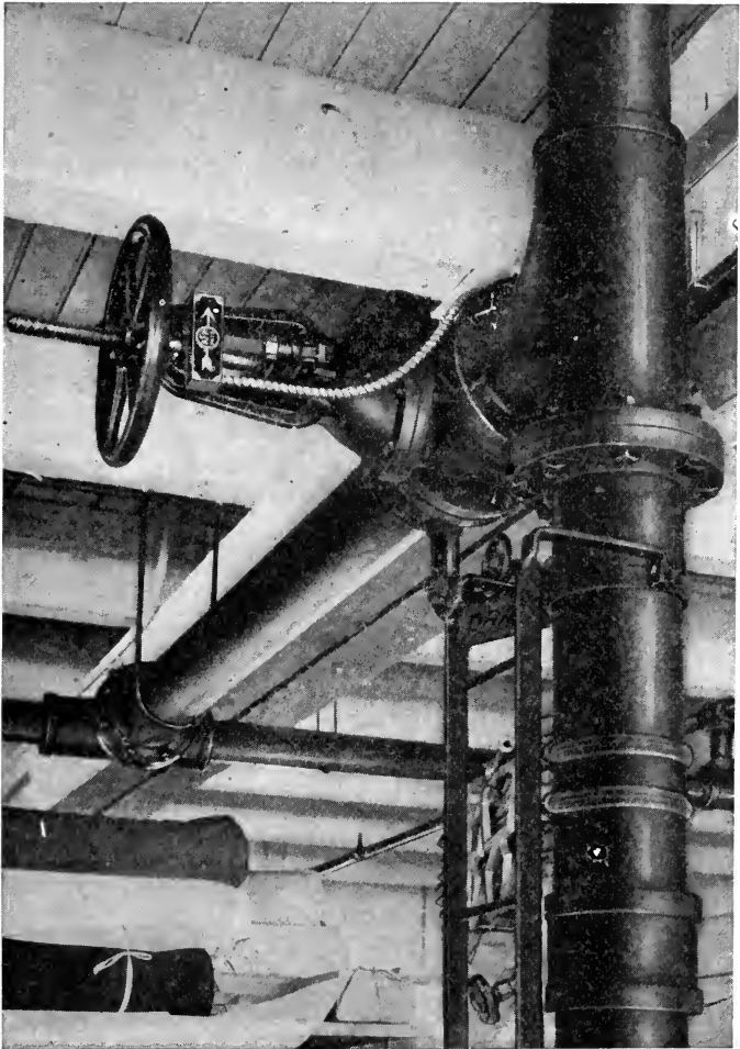
A. D. T. GATE VALVE ATTACHMENT. Showing attachment to an O. S. & Y. floor valve. Wiring in flexible conduit.
