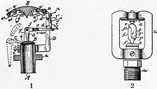
CLAPP SPRINKLERS.
