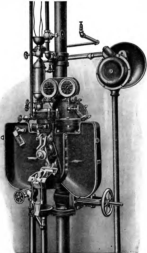
GLOBE DRY VALVE "B." Interior View. Tripped.
