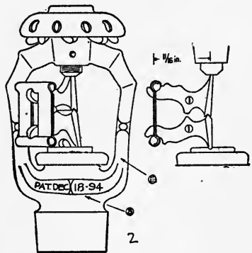
HIBBARD 2.
