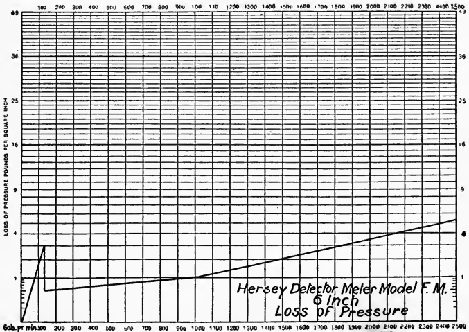
HERSEY DETECTOR METER.
