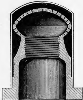
PARMELEE 3. (Section.)
