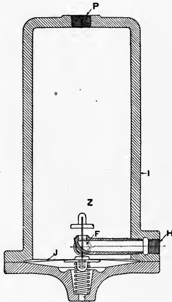
GRINNELL ENGLISH ALARM VALVE 3. RETARDING CHAMBER.
