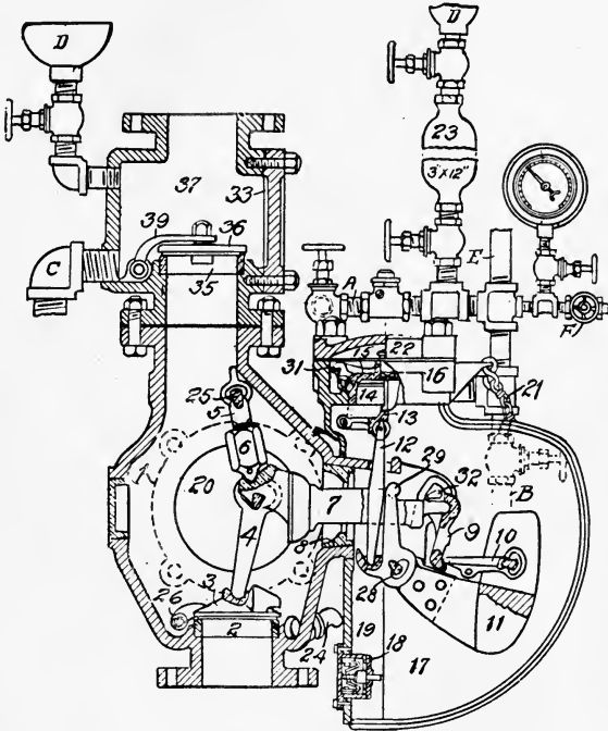
NIAGARA DRY VALVE No. 4. (Section.)
