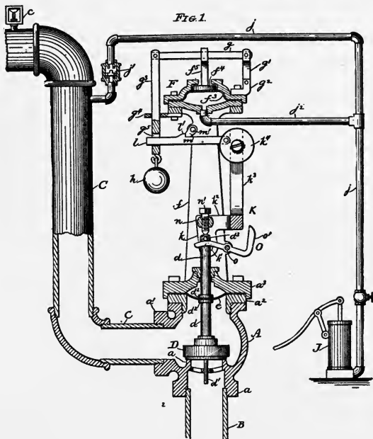
CLAPP DRY VALVE 1. (Part section.)
