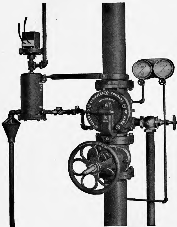
ROCKWOOD ALARM VALVE. Exterior view showing retarding chamber, etc.
