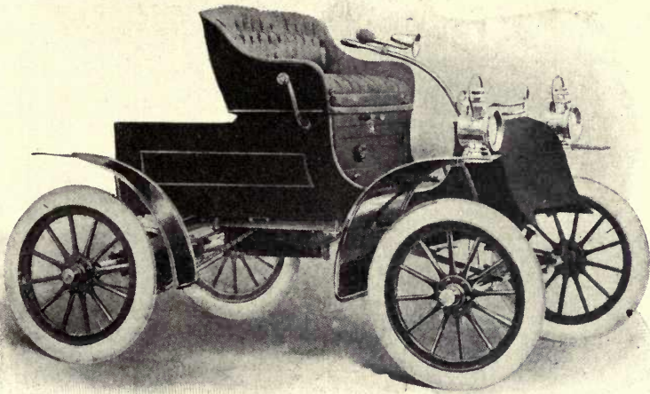
Fig. 150. Runabout. Northern Automobile Company, Detroit, Mich.
