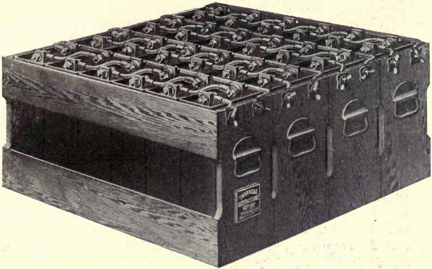
Fig. 144. Assembled Battery of 24 Cells, Bolt-Connected, Ready to Put into Car. Universal Electric Storage Battery Company, Chicago, Ill.
