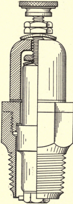
Fig. 84. Section of Sta-Rite Spark-Plug. R. E. Hardy Company, New York, N. Y.
