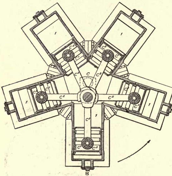
Fig. 57. Diagram Showing Operation of Adams-Farwell Rotating-Cylinder Engine. Adams Company, Dubuque, Iowa.
