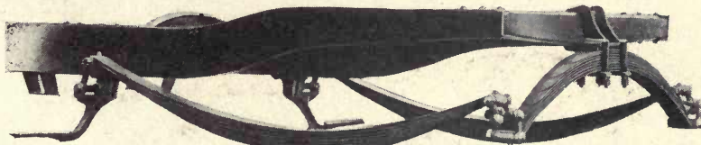
Fig. 10. Rear Spring Suspension. Peerless Motor Car Company, Cleveland, Ohio.
