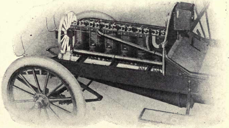
Fig. 50. Exhaust Side of Franklin Six-Cylinder Engine, Showing Regular Exhaust Pipe from Top and Auxiliary Exhaust from Bottom of Cylinders. H. H. Franklin Manufacturing Company, Syracuse, N. Y.
