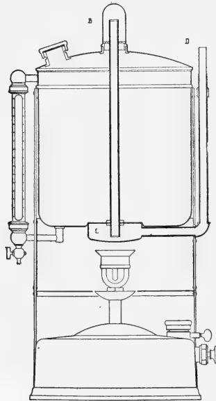
Formaldehyde apparatus.
