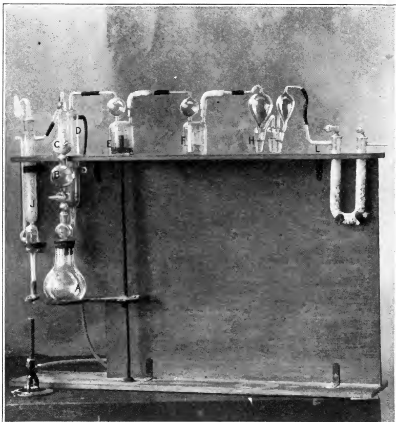
Modified Knorr Apparatus
