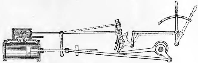
Fig. 11.—VARIABLE CUT-OFF ADJUSTMENT.
