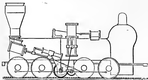
Fig. 9.—BALDWIN ENGINE FOR RACK-RAIL, 1847.
