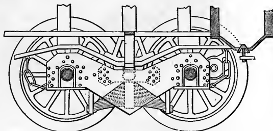
Fig. 7.—BALDWIN FLEXIBLE-BEAM TRUCK, 1842.—ELEVATION.
