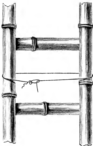
Fig. 10.—Method of Cramping Bamboo Joints.
