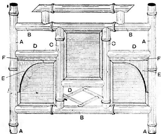
Fig. 157.—Bamboo Photograph-frame.
