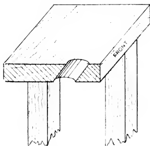
Fig. 20.—Section of Bench.
