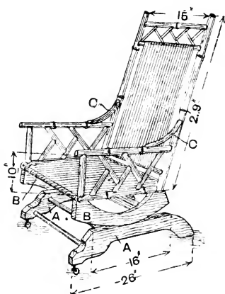
Fig. 72.—Bamboo Rocking Chair.
