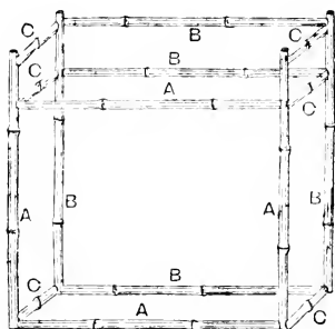
Fig. 117. —Framing of Bookcase.
