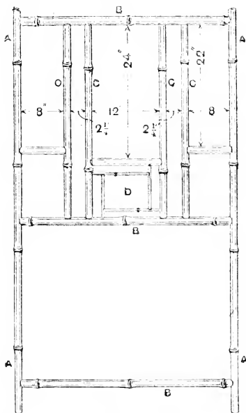
Fig. 109.—Back Section of Bamboo Cabinet.
