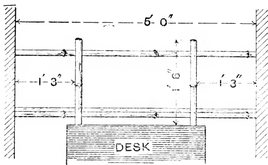
Fig. 123.—Bamboo Bookshelf.
