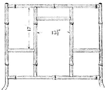
Fig. 110.—Front Section of Bamboo Cabinet.
