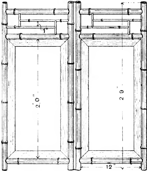
Fig. 162.—Two-fold Bamboo Screen.
