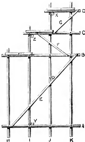
Fig. 147.—Bamboo Flower-pot Stand for Window.
