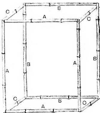
Fig. 116.—Framing of China Cupboard.
