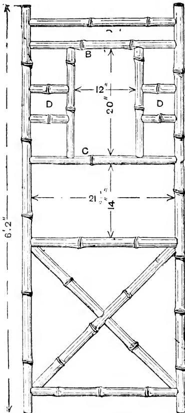
Fig. 96.—Back Section of Umbrella Stand.
