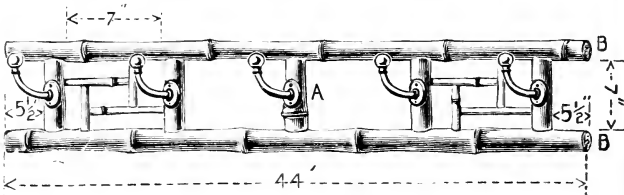
Fig. 85.—Hat Rack.
