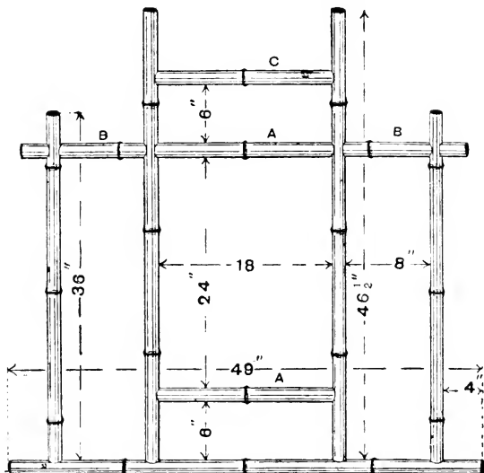
Fig. 155.—Framing of Bamboo Overmantel.
