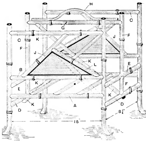
Fig. 100.—Two-Division Music Rack.
