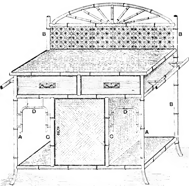
Fig. 81.—Bamboo Washstand.
