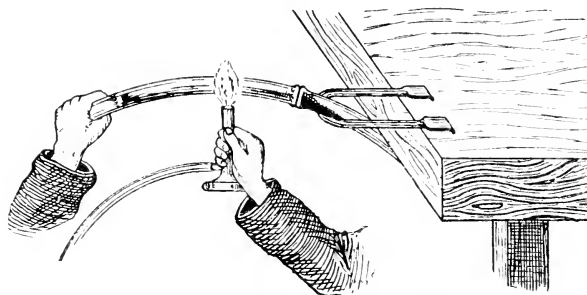
Fig. 17.—Method of Bending Bamboo.
