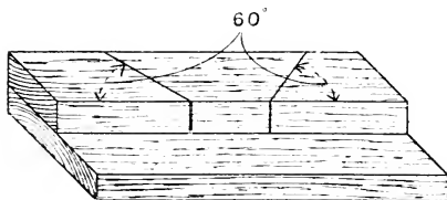
Fig. 41.—Block for Hexagonal Joints.
