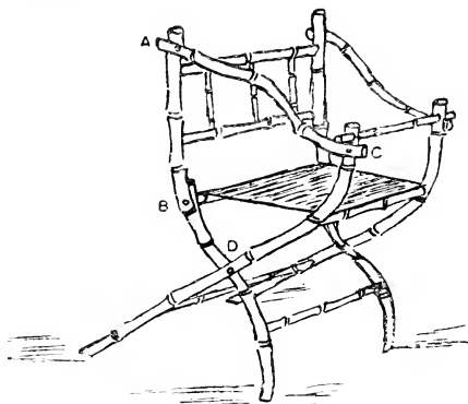
Fig. 71.—Baby's Folding Chair.
