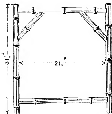
Fig. 97.—Front Section of Umbrella Stand.
