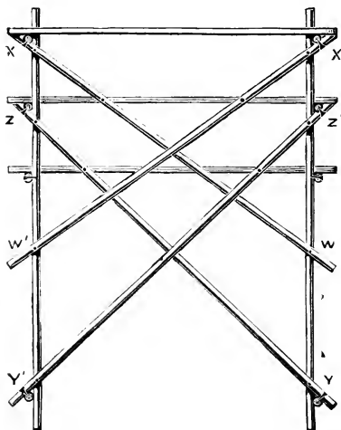
Fig. 148.—Bamboo Flower-pot Stand for Window.
