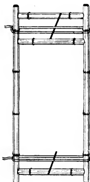
Fig. 163.—Framing of Bamboo Screen.
