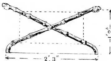
Fig. 135.—Legs of Bamboo Coal-box.
