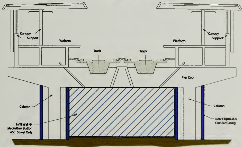
Cross Section of Aerial Station with Seismic Retrofit
