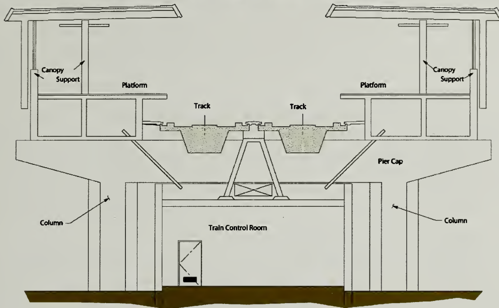
Cross Section of Typical Existing Aerial Station before Seismic Retrofit
