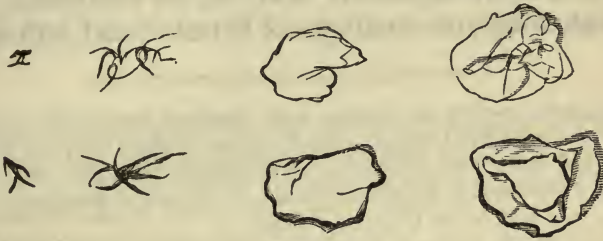
Figure 1. Indeterminate Form.
