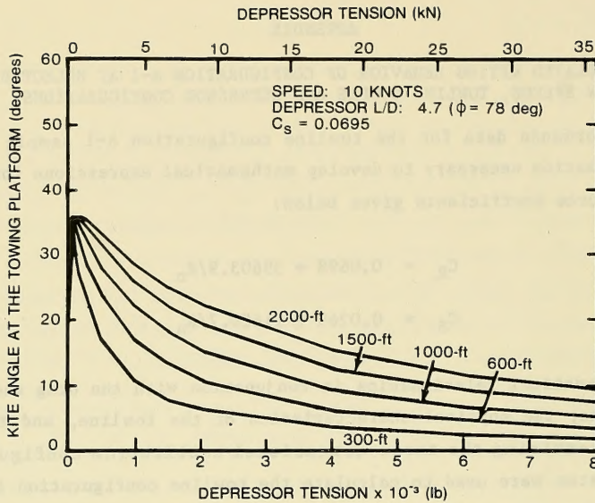
Figure A.1 - Kite Angle as a Function of Depressor Tension at Selected Towline Scopes at 5.15 m/s (10 Knots)
