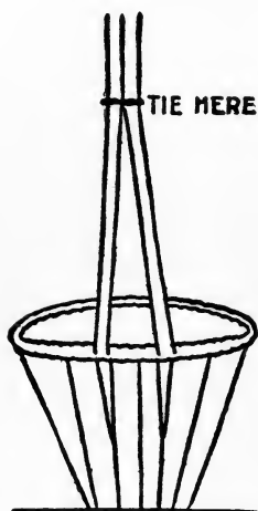
DIAGRAM NO. 11. INSERTING SPLIT HANDLE-BARS
