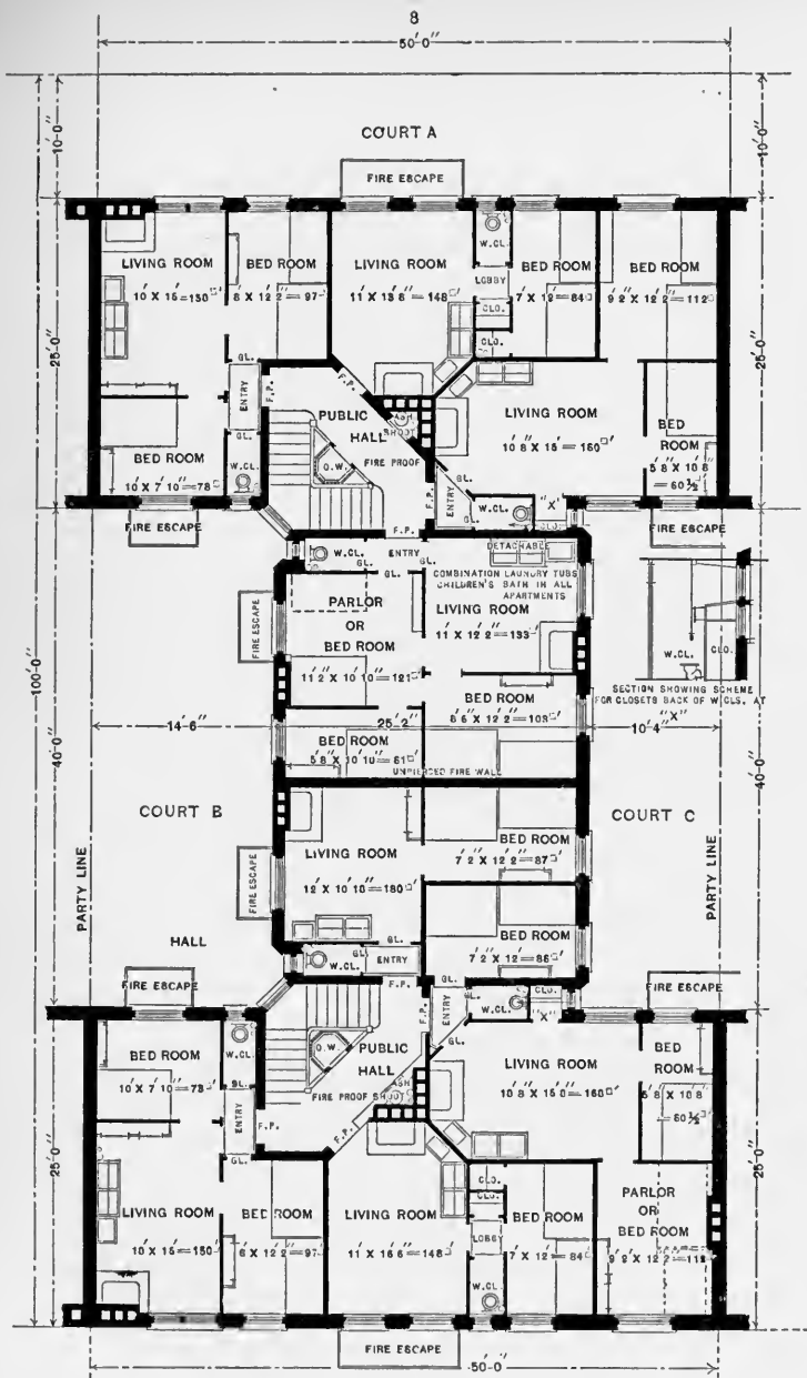
Plan of a Typical Floor in Class First of the Competition in the C. O. S. Plans of Model Tenements.
